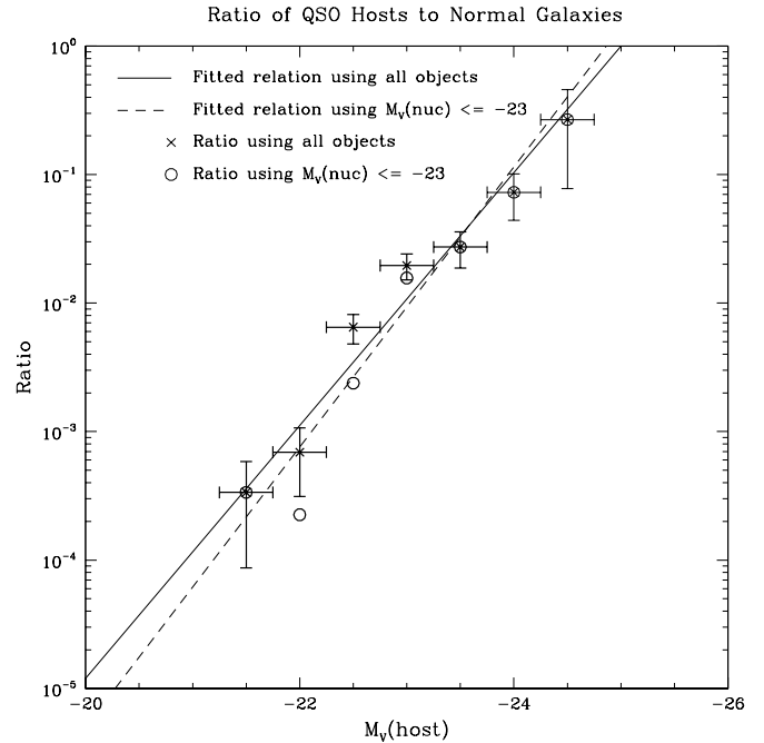
FIG. 7.—Low-redshift QSO host galaxy luminosity function divided by the normal local galaxy luminosity function, yielding the probability that a galaxy of absolute magnitude M_V will host a QSO. Crosses show this result for the entire sample, while circles show this result for QSOs with nuclear magnitudes brighter than M_V = -23 . The solid line shows the fit specified in the text for all hosts, while the dashed line shows the fit for QSOs with M_V(\text{nuc}) \leq -23 . The upper two points, drawn with thin lines, are in the extrapolated region of the normal galaxy luminosity function.
