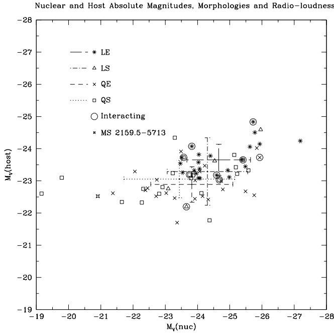
Fig. 2.—Distribution of morphological and radio properties of the sample with respect to host and nuclear luminosities. “LE” refers to radio-loud QSOs in ellipticals, “QE” to radio-quiet QSOs in ellipticals, “QS” to radio-quiet QSOs in spirals, and “LS” to radio-loud QSOs in spirals. The rms error bars for each subclass are overlaid, centered on the mean of each distribution according to the legend.
