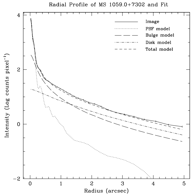
FIG. 11.—Radial profiles of MS 1059.0+7302 (solid line) and model. Note that line styles and axes differ from the previous figures. The dotted line represents the PSF model, the long-dashed line the bulge model, the dot-dashed line the disk model, and the short-dashed line the total model. This QSO has a spiral host with a bulge and a disk. The profile is not perfectly smooth but is fairly well modeled. The host model is slightly fainter than the image profile at large radii, but the excess light is included in the host magnitude.
