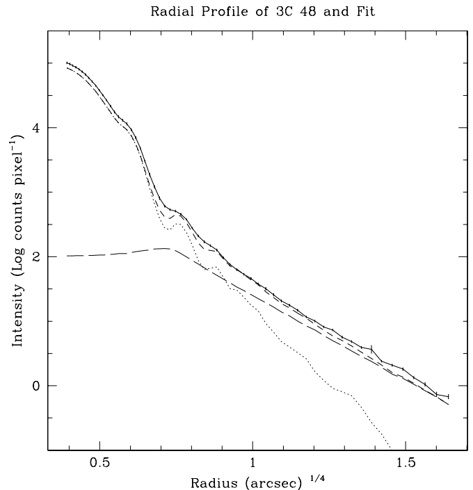
FIG. 9.—Same as Fig. 8, but for 3C 48. The higher S/N makes a smoother profile than in the case of 3C 93, but the irregular host shape causes the model to underestimate the light at small radii slightly. The turnover of the host profile is due to its center being offset from the QSO nucleus by 0''.25 .
