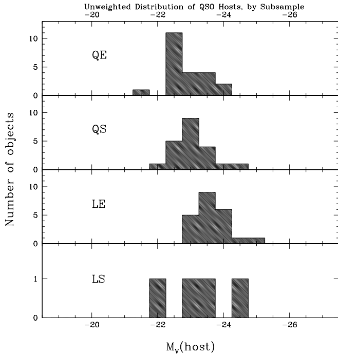
FIG. 3.—Individual host distributions of radio-quiet QSOs in ellipticals (QE), radio-quiet QSOs in spirals (QS), radio-loud QSOs in ellipticals (LE), and radio-loud QSOs in spirals (LS). Note that the vertical axes cover the same range for all but the LS subsample.
