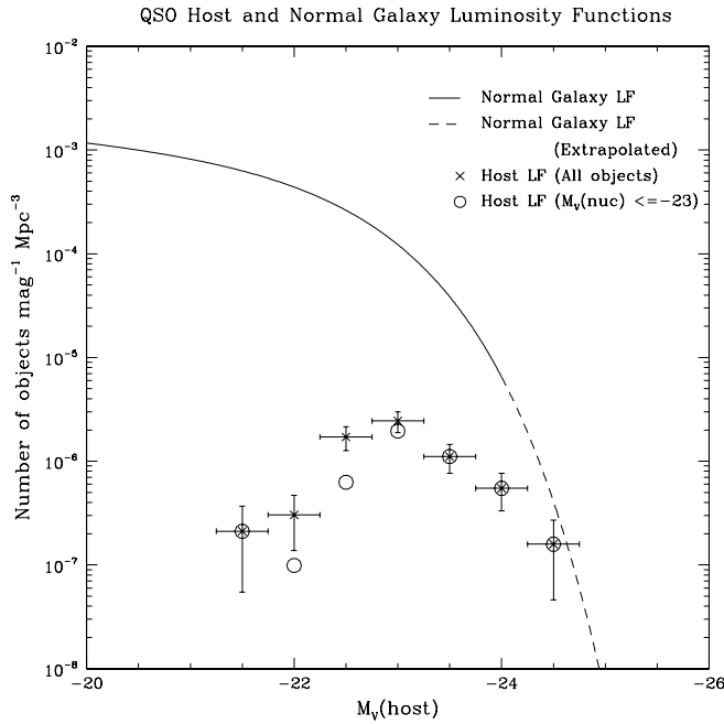
FIG. 6.—Combined luminosity function of QSO host galaxies for our sample, compared with the normal galaxy luminosity function of Metcalfe et al. (1998). The dashed line shows the extrapolated region of the normal galaxy luminosity function. Crosses show the derived luminosity function for the entire sample, while circles show the derived luminosity function for QSOs with nuclear magnitudes brighter than M_V = -23 .
