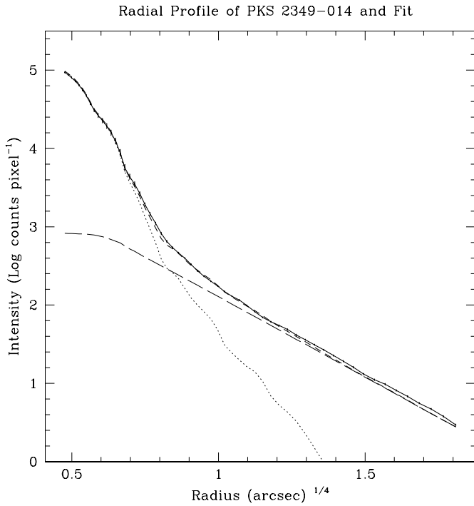
FIG. 10.—Same as Fig. 8, but for PKS 2349–014. Despite the irregularity of the host morphology, a good fit to the profile is obtained.
