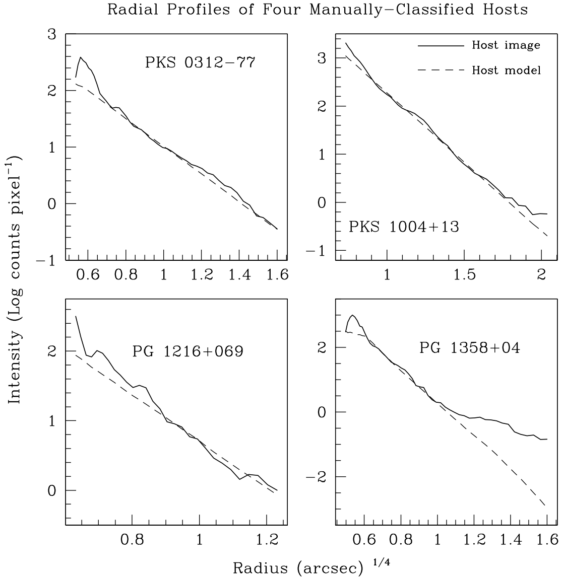
FIG. 1.—Radial profiles of four manually classified hosts. These are the four, classified as spirals by the automated fit, whose profiles more closely follow an r^{1/4} law, as shown here. The PSFs and sky backgrounds have been subtracted to show the profiles of the underlying hosts ( solid lines ). The profiles of the fitted elliptical host models ( dashed lines ) are shown for comparison. The straightness of the profiles shows that these hosts generally follow the r^{1/4} law. For PG 1358+04, this is true for the bright, inner regions. It has a distinct second component at large radii that is not modeled and is masked from the fit, but this only exists in regions fainter than 1 count pixel -1 . The tilt of PG 1216+069's host profile relative to the model is due to the weighting scheme and the imperfect fit of the bright PSF. On the basis of these profiles, all four of these hosts are classified as ellipticals.
