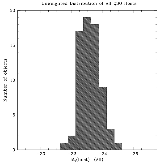
FIG. 4.—Unweighted absolute magnitude distribution function of all QSO hosts. The narrow width of the distribution is evident.
