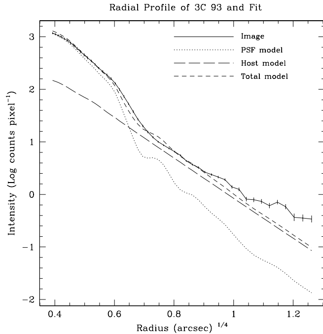
FIG. 8.—Radial profiles of 3C 93 (solid line) and model. Error bars on the image profile represent uncertainties in the elliptical isophotes used to plot the profile. The model PSF is represented by the dotted line, the model host by the long-dashed line, and the total model by the short-dashed line. Because of the low S/N, the model is not a perfect match to the image profile. Note the deviation of the host from a strict r^{1/4} law profile at large radii. Although this feature is not fitted by the model, the extra light is included in the host magnitude.
