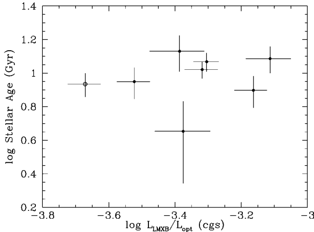
FIG. 1.—Mean ages of the stars in elliptical galaxies (Trager et al. 2000) are plotted against the ratios of the X-ray luminosity of their LMXBs to their optical B -band luminosity (White 2002b). Open circle indicates an upper limit to L_{\text{LMXB}} due to the presence of an AGN.
