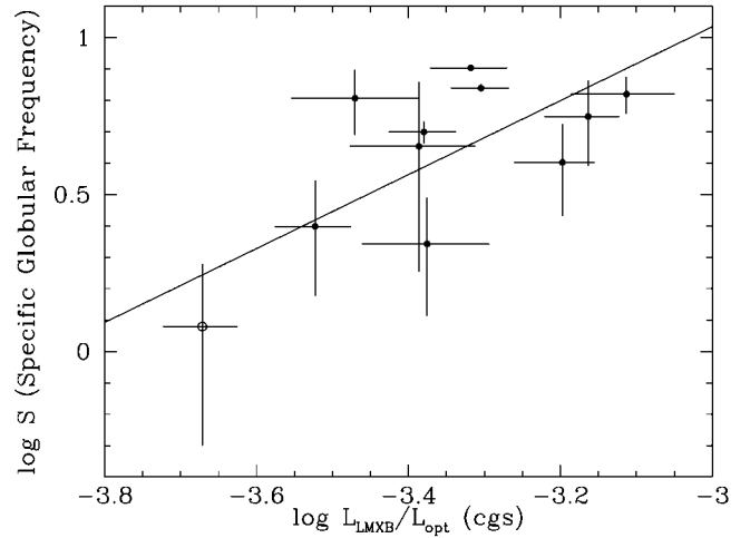
FIG. 2.—Logarithm of the specific frequency of globular clusters S (Kissler-Patig 1997) vs. the X-ray/optical luminosity ratio for elliptical galaxies. Best-fit relationship (using the ASURV statistical package; Isobe, Feigelson, & Nelson 1986) is L_{\text{LMXB}}/L_{\text{opt}} \propto S^{1.2 \pm 0.4} , with a 90% probability of correlation via Kendall's \tau test. Open circle indicates an upper limit to L_{\text{LMXB}} due to the presence of an AGN.
