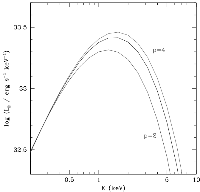
FIG. 2.—Phase-averaged spectrum, plotted as luminosity measured by an observer at infinity at different photon energies, for a neutron star with a magnetic field of 10^{14} G and two antipodal hot emitting regions with effective temperature T_{\text{eff}} = 0.5 keV and angular size \rho = 15^\circ . Here the two orientation angles \alpha and \beta are taken to be 90^\circ . [See the electronic edition of the Journal for a color version of this figure.]
