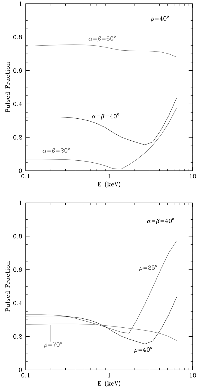
FIG. 4.—Same as in Fig. 3 but for one hot emitting region and a neutron star compactness corresponding to p = 2.5 . Curves in panel (a) correspond to different values of the orientation angles for a size of \rho = 40^\circ . In panel (b) \alpha = \beta = 40^\circ and the size \rho of the hot region is varied. [See the electronic edition of the Journal for a color version of this figure.]
