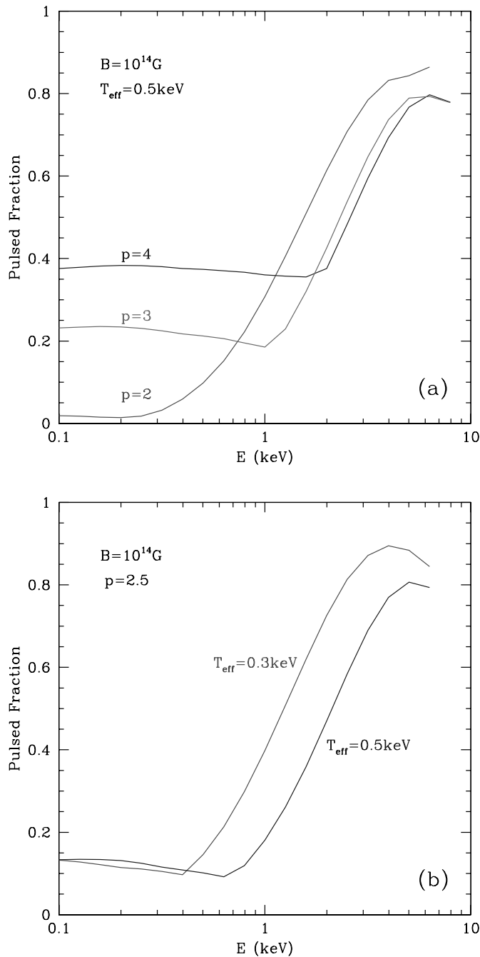
FIG. 3.—Predicted energy dependence of the pulsed fraction for surface emission from a magnetar with two antipodal hot regions of size \rho = 15^\circ and different values of the (a) neutron star compactness and (b) effective temperature, for \alpha = \beta = 90^\circ . [See the electronic edition of the Journal for a color version of this figure.]
