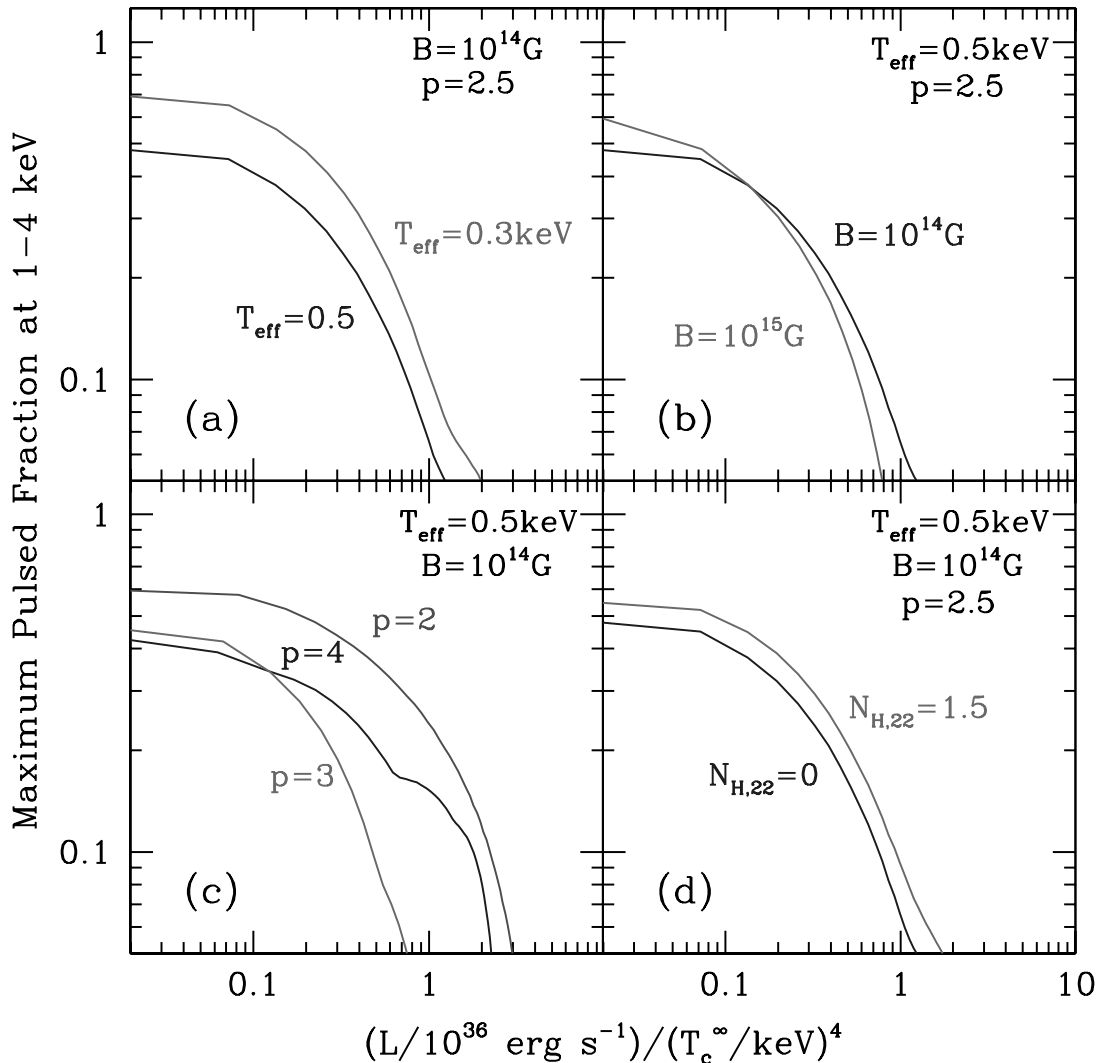
FIG. 5.—Maximum pulsed fractions in the 1–4 keV range plotted against the ratio of the luminosity to the fourth power of the color temperature, as inferred by an observer at infinity, for different values of the (a) effective temperature, (b) magnetic field strength, (c) compactness of the neutron star, and (d) hydrogen column to the source in units of 10^{22} \text{ cm}^{-2} . For each curve, regions below and to the left of the curve are allowed, whereas the regions above and to the right are excluded for any choice of \alpha and \beta . [See the electronic edition of the Journal for a color version of this figure.]
