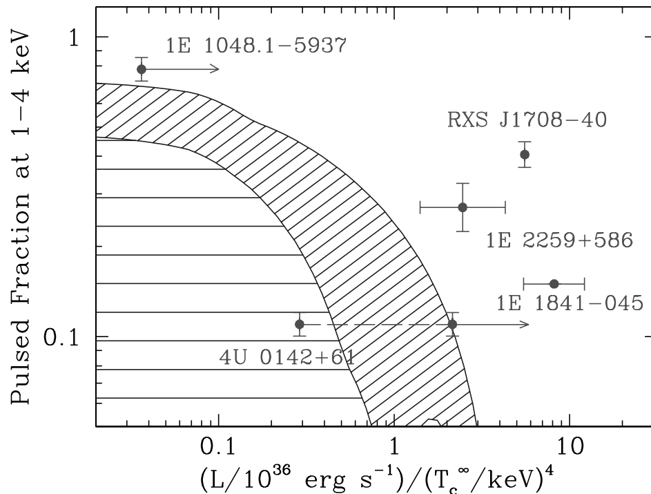
FIG. 6.—Comparison of the AXP data to the maximal predictions of the thermally emitting magnetar model with two antipodal emitting regions. The diagonally shaded band shows the maximum pulsed fraction as a function of the ratio of luminosity to the fourth power of the color temperature, and spans the entire range of curves shown in Figure 5 for \alpha = \beta = 90^\circ . The horizontally shaded region is also allowed for smaller orientation angles. The right arrows on the data points indicate conservative lower limits, while the error bars represent an allowed range of values. Most of the sources lie outside the allowed region of the diagram. [See the electronic edition of the Journal for a color version of this figure.]
