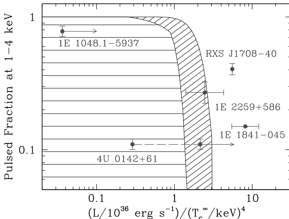
FIG. 7.—Same as in Fig. 6, but for a single emitting region on the neutron star. Most data points lie within the allowed region. [See the electronic edition of the Journal for a color version of this figure.]
