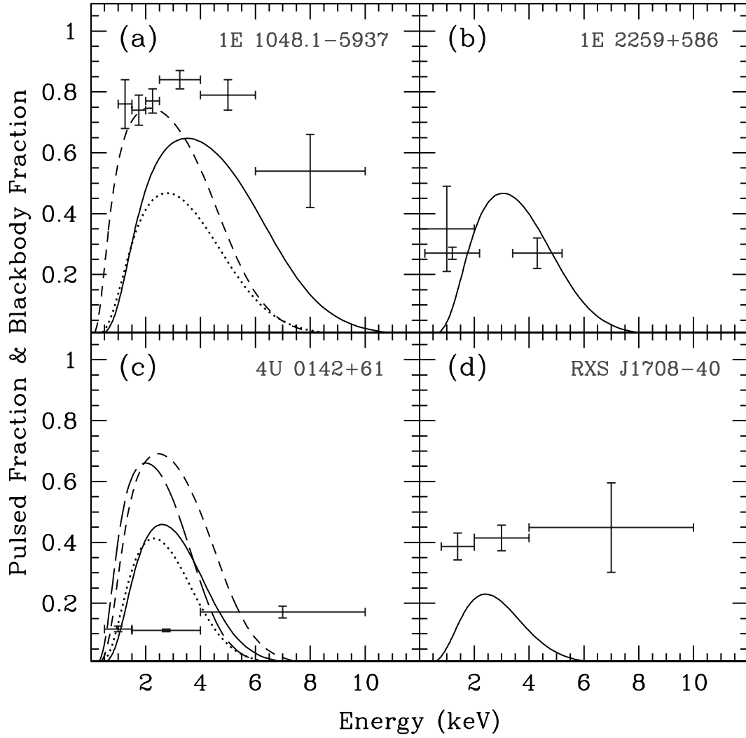
FIG. 1.—Observed pulsed fraction (error bars) and the fractional contribution of the blackbody component to the X-ray spectrum (lines) as a function of photon energy, for four AXPs. The multiple lines in each panel correspond to fits to different data sets; the references and details are given in Table 3. [See the electronic edition of the Journal for a color version of this figure.]
