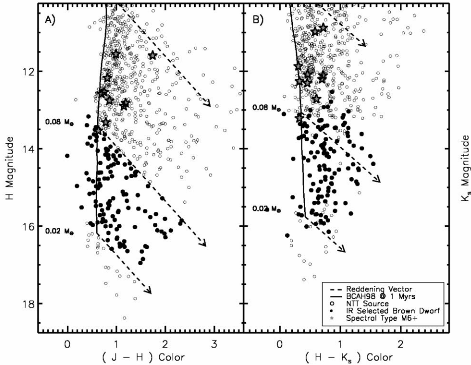
FIG. 1.—Candidate brown dwarfs from the Trapezium Cluster infrared color-magnitude diagrams. Only sources having NTT observations and JH and K_s magnitudes are shown. Trapezium sources are compared with the location of the 1 Myr (at 400 pc) isochrone from the BCAH98 model atmospheres. Candidate brown dwarfs (filled circles) were selected by their H -band luminosities (and colors) and are marked in both color-magnitude diagrams. Reddening vectors for 1, 0.08, and 0.02 M_{\odot} objects are drawn at visual extinctions of 20, 20, and 10 mag, respectively. Stars with spectral types \geq M6 are identified as stars. (a) J-H/H color-magnitude diagram. (b) H-K_s/K_s color-magnitude diagram. [See the electronic edition of the Journal for a color version of this figure.]
