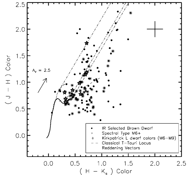
FIG. 2.— H-K_s/J-H color-color diagram for the 109 sources with NTT JHK_s magnitudes and that fall into the brown dwarf regime of Fig. 1a. The candidate brown dwarfs are compared with the intrinsic colors of giants and A0–M6 dwarfs from Bessell & Brett (1988), the late-M (M6–M9) color sequence from Kirkpatrick et al. (2000), and the classical T Tauri locus from Meyer, Calvet, & Hillenbrand (1997). Appropriate reddening vectors (Cohen et al. 1981) are drawn for giants, for M6 stars, and for M9 stars. Colors of Trapezium sources with very late (M6+) spectral types are shown as stars. Circled sources have color errors of less than 10%, and the size of 15% uncertainties in color is illustrated at the upper right. [See the electronic edition of the Journal for a color version of this figure.]
