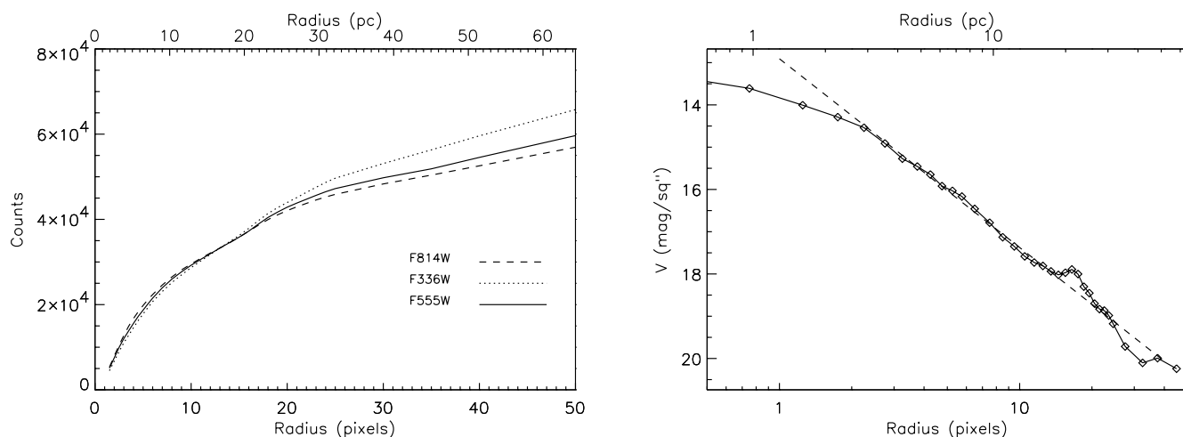
FIG. 5.— Left : Luminosity of the cluster as a function of radius, measured on F336W, F555W, and F814W images. The F336W and F814W profiles have been normalized to that measured on the F555W image. Right : The V -band surface brightness profile, corrected for foreground extinction. Note the bump in the profile at r \sim 15 pixels, resulting from the fainter companion cluster. The power-law envelope clearly extends to very large radii. One pixel equals 0''.045 , or about 1.3 pc. The dashed line is a power-law fit. No correction for the instrumental profile has been made.
