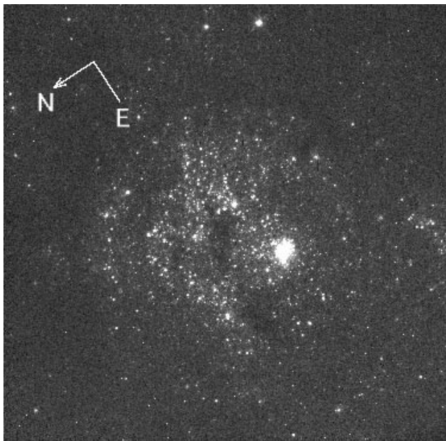
FIG. 2.—An F555W image showing the PC field of view. North and east are indicated by the arrow. The young globular cluster is easily recognizable as the single most luminous object, near the center of the image.
