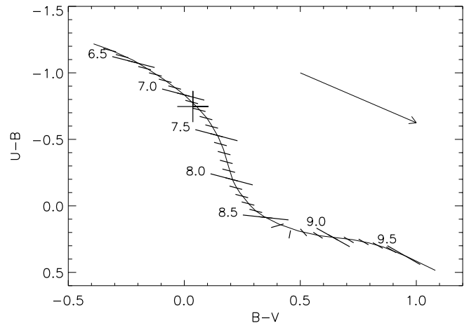
FIG. 10.— (B - V, U - B) two-color diagram showing the Girardi et al. (1995) S-sequence and the colors of the young globular cluster in NGC 6946 (large cross); log (age) values are indicated along the S-sequence. The arrow indicates a reddening of E(B - V) = 0.5 .
