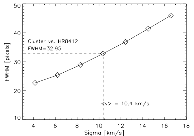
FIG. 7.—Illustration of the technique used for deriving velocity dispersions. Diamonds : FWHM of the cross-correlation peak for the template star HR 8412 vs. HR 9053, the latter convolved with Gaussians of different dispersions as indicated on the x-axis of the plot. The FWHM of the cluster vs. HV 8412 cross-correlation peak of 32.95 pixels corresponds to a velocity dispersion of 10.4 km s -1 .
