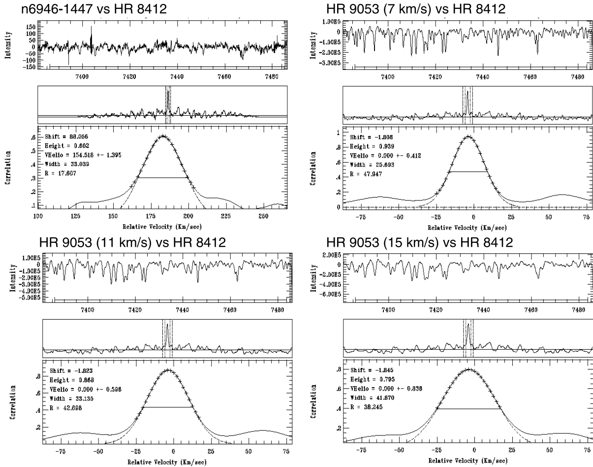
FIG. 6.—Cross-correlation functions for the young cluster vs. HR 8412 ( upper left ) and for HR 9053 vs. HR 8412, where the HR 9053 spectrum has been convolved with Gaussians corresponding to velocity dispersions of 7, 11, and 15 km s -1 .
