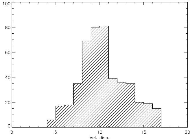
FIG. 8.—Distribution of velocity dispersions derived from all combinations of template stars and echelle orders.
