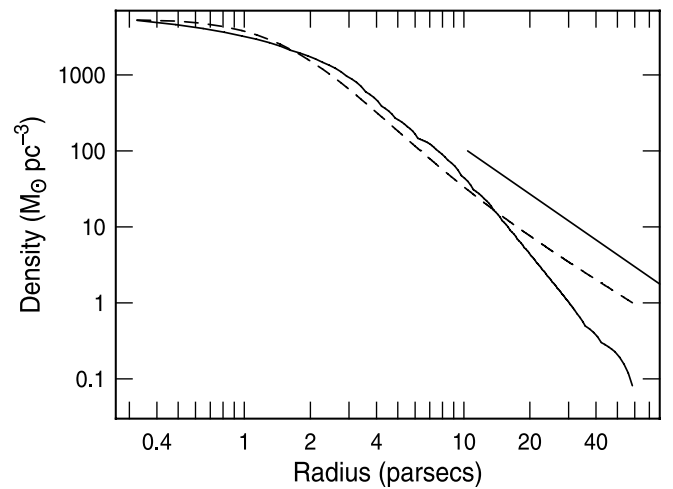
FIG. 9.—Best-fit solution for the three-dimensional density of the cluster (solid line) and the corresponding isothermal profile are plotted as functions of radius. The straight line has a slope of -2 ; pixel scale is 1.3 pc, so the fitted points at small radii are unresolved. The observed cluster is close to isothermal in the inner regions, but it becomes cooler in the outer regions where the density drops off faster than the inverse square of radius.
