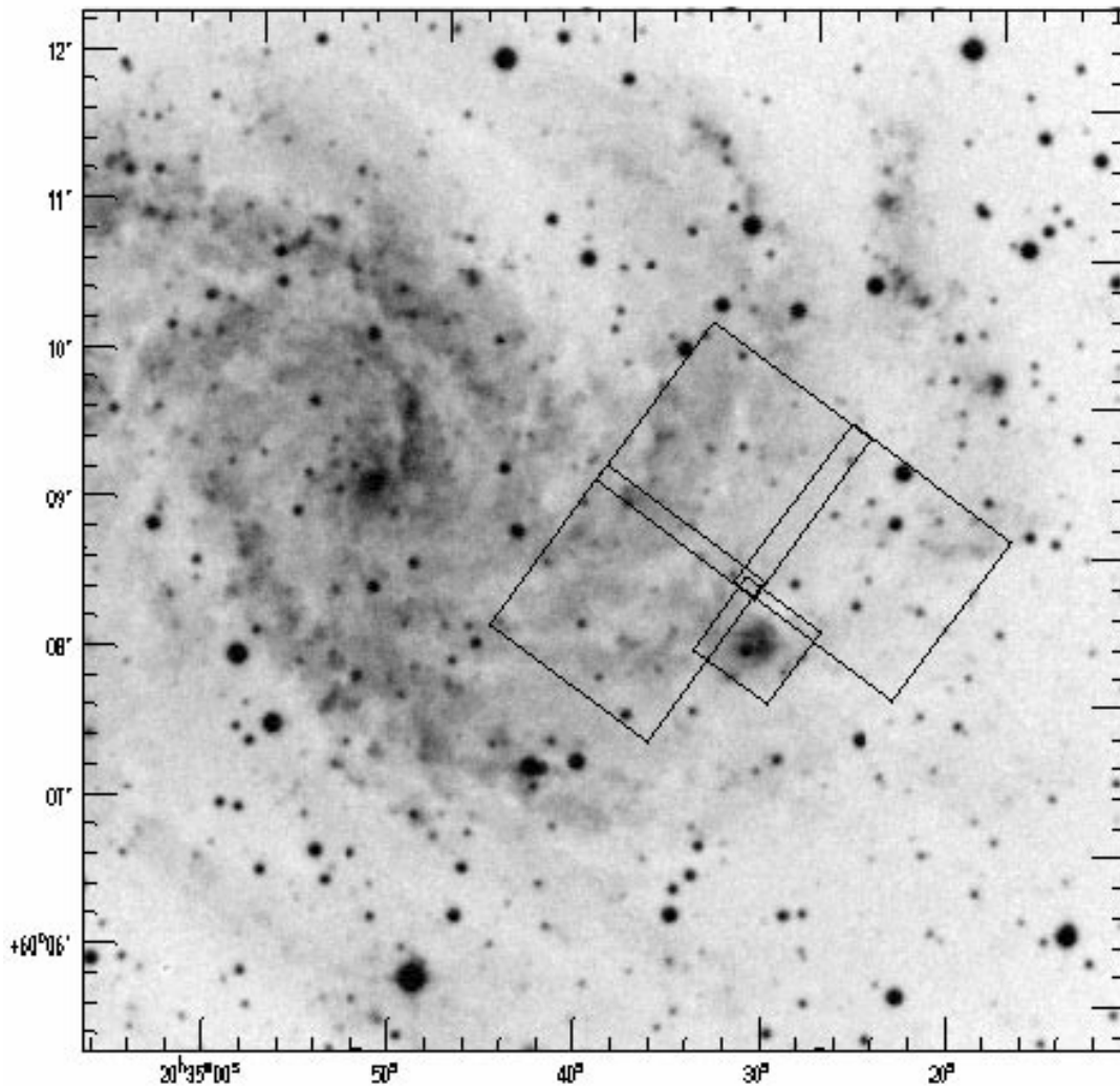
FIG. 1.—WFPC2 field of view superimposed on a Digital Sky Survey image of NGC 6946; north is up and east toward the left
