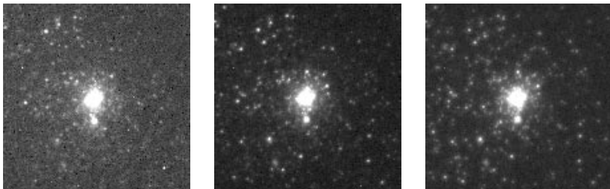
FIG. 4.—Close-ups of the young globular in F336W, F555W, and F814W. Each image spans about 6'' . Orientation is the same as in Fig. 2.
