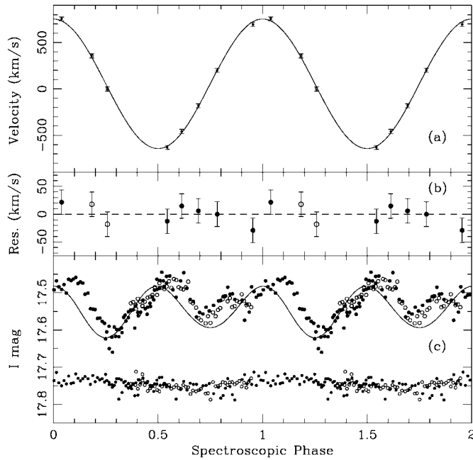
FIG. 1.—Spectroscopic and photometric data folded on the orbital period and the ephemeris given in Table 1. (a) Radial velocity measurements of the secondary star. The smooth curve is a fit to a circular orbit based on the velocity amplitude and phase given in Table 1. (b) The residual differences between the data and the fitted curve. Open and filled symbols are for December 1 and 4, respectively. (c) The top trace is the I -band light curve of XTE J1118+480 with a superposed ellipsoidal model. Filled and open symbols are for November 30 and December 1, respectively. The bottom trace shows the intensity of a nearby comparison star of magnitude I = 17.0 ; the trace is shown here offset by 0.75 mag for convenience of display. The rms variation in the star's intensity is 0.015 mag.
