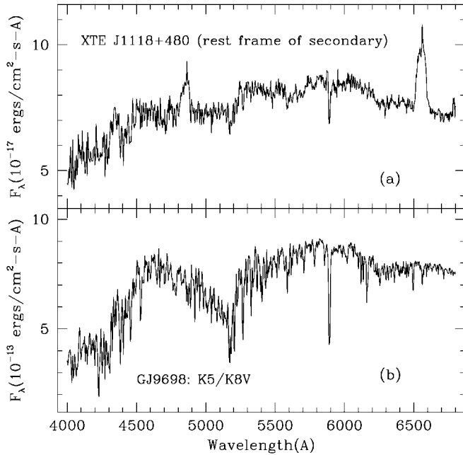
FIG. 2.—(a) Spectrum of XTE J1118+480 in the rest frame of the secondary star. The photospheric absorption features are most apparent in this frame; however, the prominent Balmer emission lines are significantly distorted. (b) The spectrum of GJ 9698, which was used as a velocity template for the cross-correlation analysis.
