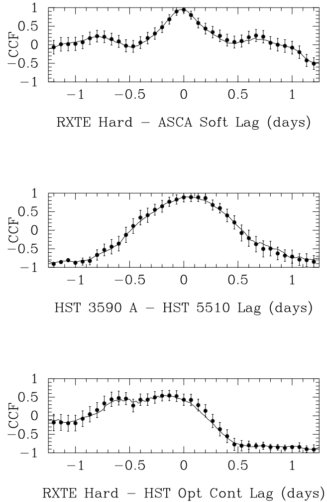
FIG. 6.—Interband temporal cross-correlation functions. The solid line refers to the interpolated cross-correlation function, while the error bars refer to the discrete cross-correlation function. At the top is the RXTE hard– ASCA soft correlation function, next is the HST 3590–5510 Å correlation function, and at the bottom is the RXTE hard–mean optical continuum correlation function. In all plots a negative lag means that the first listed band leads the second.
