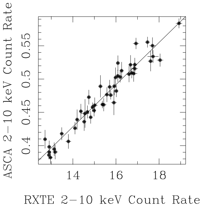
FIG. 5.—Zero-lag correlation plot of 2–10 keV count rates measured from RXTE and ASCA . The solid line is a linear fit to the data, which goes within 0.5\sigma of the origin (not shown). Note that the RXTE data have much higher count rates, and much better signal-to-noise ratios, than the ASCA data.
