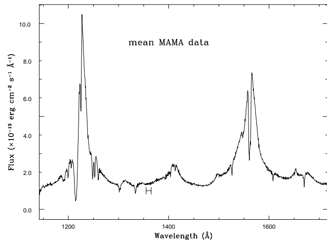
FIG. 3.—Ultraviolet spectrum of NGC 3516. The position of the 1355–1365 Å continuum extraction band is noted by the small horizontal error bar.
