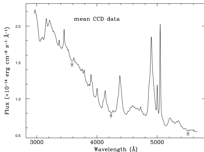
FIG. 4.—Optical spectrum of NGC 3516. Positions of continuum extraction bands (3575–3600 Å, 4223–4245 Å, and 5500–5525 Å) are noted by the small horizontal error bars.
