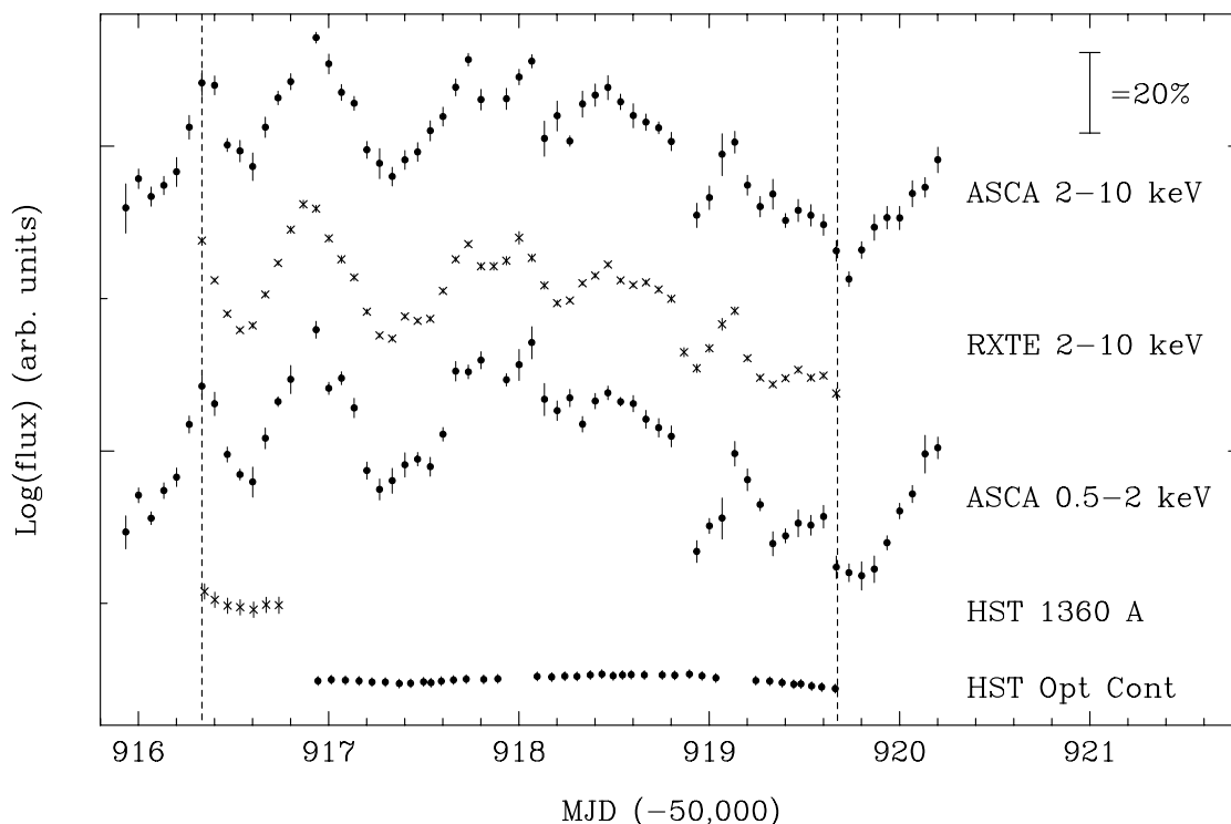
FIG. 1.—X-ray, ultraviolet, and optical continuum light curves of NGC 3516. The light curves are, from the top, the ASCA hard (2–10 keV) band, the RXTE hard (2–10 keV) band, the ASCA soft (0.5–2 keV) band, the HST ultraviolet (1360 Å) band, and the HST mean optical band. The error bar in the upper right shows a factor of 20% change. Error bars are 1\sigma statistical uncertainties, except for the ultraviolet data, which have 1.7% added in quadrature to account for the systematic errors. Note the strong variability in the X-ray bands, but the ultraviolet and optical variations are quite weak, as shown in detail in Fig. 2.
