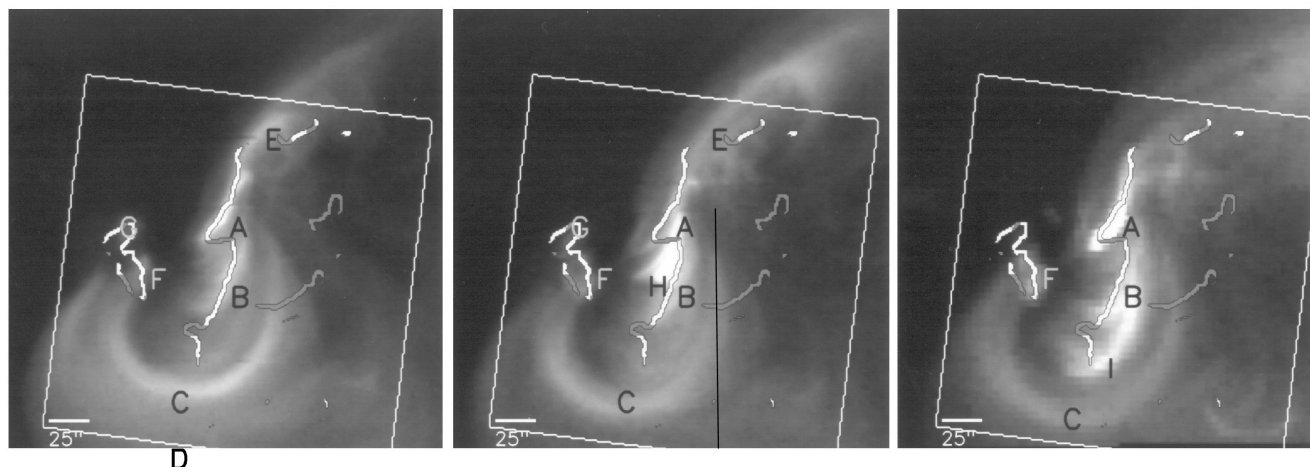
FIG. 9.—Changes in the persistently bright coronal structure of an active region over several hours. This sequence (together with Fig. 3) exemplifies that while enhanced coronal heating in active regions generally persists in the same places for about an hour, it often changes markedly in a few hours. Left : Persistent coronal brightness in AR 6982 (for the orbit with sunrise at 17:58 UT on 1991 December 26) superposed on the neutral-line magnetic shear map from the 18:23 UT magnetogram. Except for its smaller field of view, this frame is the same as the right panel of Fig. 4. Middle : Same as on the left, except that the persistent coronal brightness image is from the orbit with sunrise at 21:13 UT (two orbits later). Right : Same as on the left, except that the persistent brightness image is from the orbit with sunrise at 02:06 UT on December 27 (three orbits after the second frame and five orbits after the first frame). All of the bright features labeled by letters change in brightness or shape or both from frame to frame. Extended loop D is below threshold after the first frame; core point G and extended loop E are below threshold in the last frame. Extended loop E is obviously not the same magnetic loop in the first and second frames; extended loop C shifts southward in each successive frame. Core arcade H is seen only in the second frame; extended loop I is noticeable only in the last frame. All five of our active regions displayed comparably large orbit-to-orbit changes in their persistently bright coronal features.
