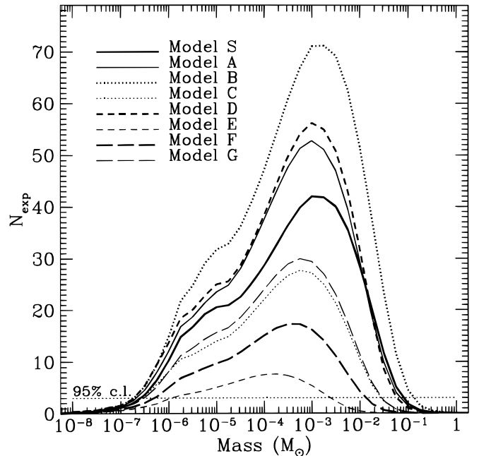
FIG. 10.—A plot of the number of expected events vs. mass for the standard model and seven power-law halo models. The results shown are for the combined spike and standard analyses, and with \hat{t} < 20 days. The line at N_{\text{exp}} = 3 is the 95% c.l. upper limit, and the regions of the curves above this line are ruled out.
