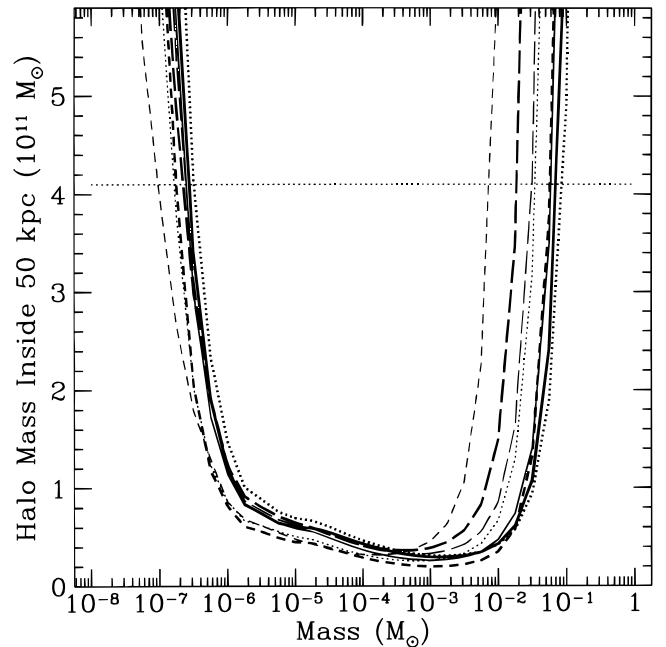
FIG. 12.—Upper limits on the total mass of MACHOs interior to 50 kpc as a function of lens mass. The results shown are for the combined spike and standard analyses, and with \hat{t} < 20 days. The regions above the curves are ruled out at the 95% c.l. Objects of mass 3.2 \times 10^{-7} M_{\odot} < m < 1.87 \times 10^{-2} M_{\odot} cannot make up the canonical value of 4.1 \times 10^{11} M_{\odot} , independent of the model used.
