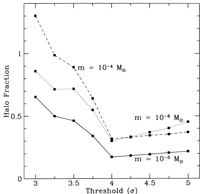
FIG. 7.—Halo fraction upper limit (95% c.l.) as a function of threshold for three values of lens mass. The upper limit rises at lower thresholds because events are detected at these thresholds, and the 95% c.l. upper limit on N_{\text{exp}} increases accordingly.
