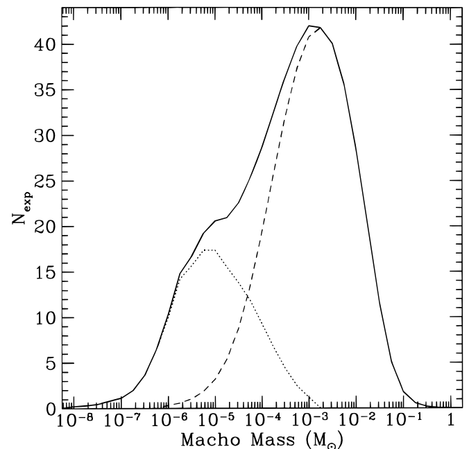
FIG. 8.—Number of expected events as a function of MACHO mass after combining the standard and spike analyses, with a cut on events with t > 20 days. The spike result is plotted with the dotted line (with the double-counted events subtracted), the standard result with the dashed line, and the combined result is shown with the solid line.
