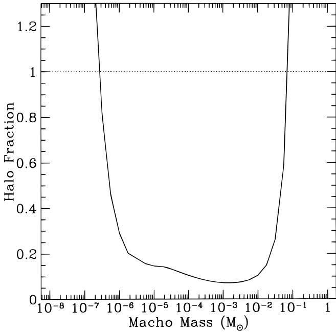
FIG. 9.—Halo fraction upper limit (95% c.l.) for the combined spike and standard analyses and with \hat{t} < 20 days.
