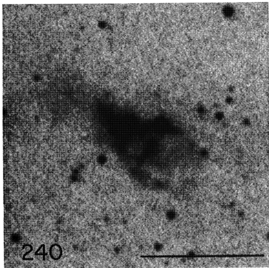
FIG. 1—Photographs of the ring nebulae in the light [O\ III] \lambda 5007 . The individual prints are identified with DEM numbers, the WR stars are located by marginal tick marks, and the horizontal bars indicate 2' on the sky.
