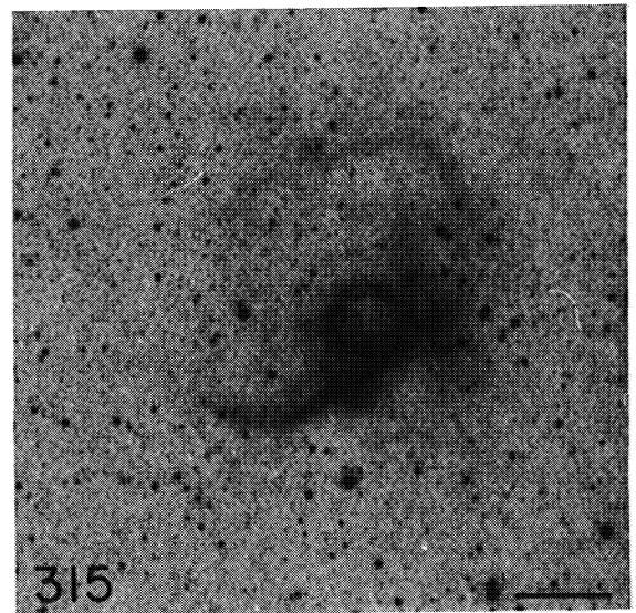
FIG. 1—Photographs of the ring nebulae in the light [O\ III] \lambda 5007 . The individual prints are identified with DEM numbers, the WR stars are located by marginal tick marks, and the horizontal bars indicate 2' on the sky.
