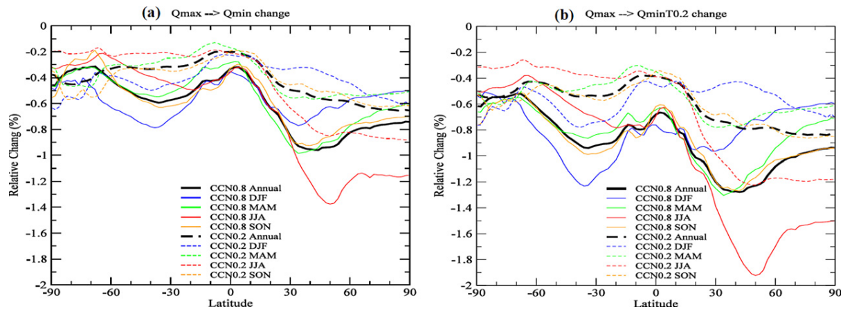
Figure 3. Annually and seasonally averaged zonal mean relative changes of CCN0.8 and CCN0.2 in the lower troposphere (0–3 km above the surface): (a) due to ionization rate change ( Q_{\max} \rightarrow Q_{\min} ) only; (b) due to both Q and T changes ( Q_{\max} \rightarrow Q_{\min T0.2} ). DJF (December, January, February), MAM (March, April, May), JJA (June, July, August), and SON (September, October, November) refer to winter, spring, summer, and fall seasons, respectively.
