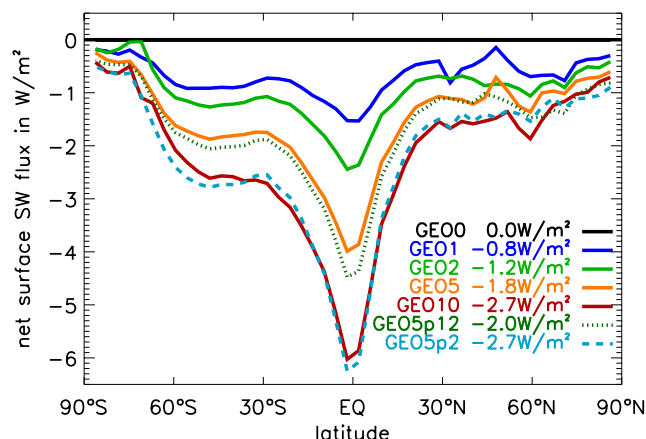
Figure 10. Change in zonal mean annual mean net SW flux at the surface in \text{W m}^{-2} due to geoengineering for clear-sky conditions with respect to the base run (GEO0). Listed values show change in annual mean global mean SW flux.
