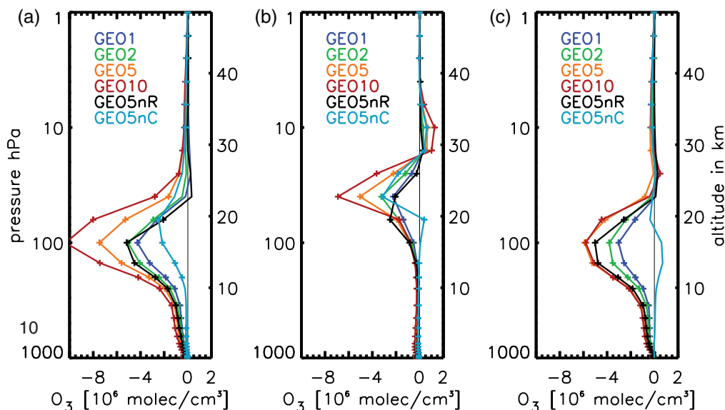
Figure 7. Annual zonal mean O_3 (in 10^6 molecules cm^{-3} ) changes with respect to GEO0 (a) in the south polar region ( 60^\circ S – 90^\circ S ), (b) in the tropics ( 30^\circ S – 30^\circ N ), (c) in the north polar region ( 60^\circ N – 90^\circ N ). Plus signs indicate changes to be statistically significant on the 95%-confidence interval ( t -test).
