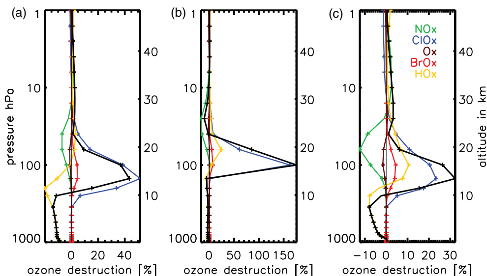
Figure 8. Change in annual zonal mean ozone destruction rate due to injection of 5 Mt/a S (GEO5) in the lower stratosphere. (a) Southern high latitudes ( 60^\circ S – 90^\circ S ), (b) tropics ( 30^\circ S – 30^\circ N ), (c) northern high latitudes ( 60^\circ N – 90^\circ N ). Change of loss rate in per cent relative to the total chemical destruction rate (sum of all destruction cycles) of base run GEO0. Black curve: change in total chemical ozone destruction. Coloured lines: nitrogen ( NO_x ), chlorine ( ClO_x ), hydrogen ( HO_x ), bromine ( BrO_x ) catalyzed destruction cycles and cannibalistic reactions ( O_3 ). The BrO_x catalyzed destruction includes the destruction by the coupled BrO_x – ClO_x –destruction cycle. Plus signs indicate statistically significant changes on the 95%-confidence interval ( t -test).
