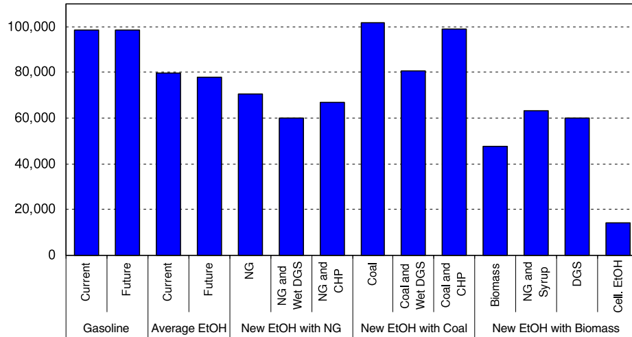
Figure 11. Well-to-wheels GHG emissions of ethanol and gasoline (CO 2 -equivalent grams per million Btu of fuel produced and used).
