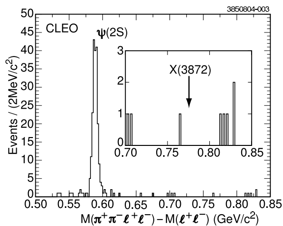
Figure 1. Data events as function of \Delta M \equiv M(\pi^+\pi^-l^+l^-) - M(l^+l^-) . The \psi(2S) is clearly visible and no apparent enhancement is seen in the X(3872) region.
