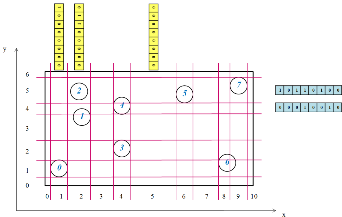
Figure 10. Bitmasks of the axes marking contained solids.
