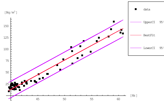
Figure 6. An example of correlation between radon-meter data and low threshold counting rate.
