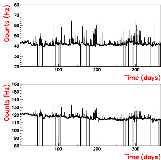
Figure 1. Low energy counting rate in one year of data for internal (top panel) and external (bottom panel) counters.
