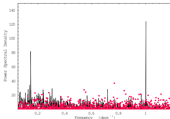
Figure 2. Spectral analysis result of the LVD data (black line) compared to normally distributed data (red point, white noise hypothesis). The LVD data show two main peaks (at 95% CL) corresponding to two signals with period 1 day and 7 days respectively.
