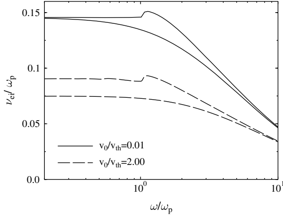
Figure 3. Electron–ion collision frequency as a function of the laser frequency for a hydrogen plasma ( n_e = 10^{21}\text{cm}^{-3} ; T = 10^5 K) for two different field strengths. The upper curve of each pair corresponds to the full dynamical screening, the lower one to the static screening approximation.
