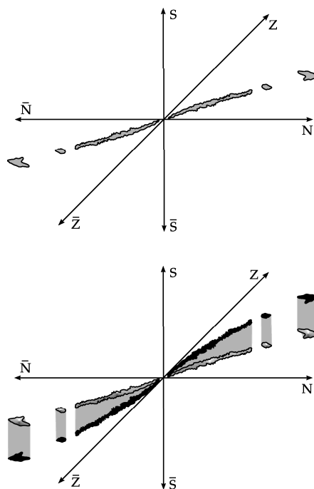
Figure 7. The extension of the periodic system into the sectors of strangeness S, \bar{S} and antimatter \bar{Z}, \bar{N} . The stable valley winds out of the known proton ( Z ) and neutron ( N ) plane into the S and \bar{S} sector, respectively. The same can be observed for the antimatter sector. In the upper part of the figure only the stable valley in the usual proton ( Z ) and neutron ( N ) plane is plotted, however, extended into the sector of antiprotons and antineutrons. In the second part of the figure it has been indicated, how the stable valley winds out of the Z - N -plane into the strangeness sector.
