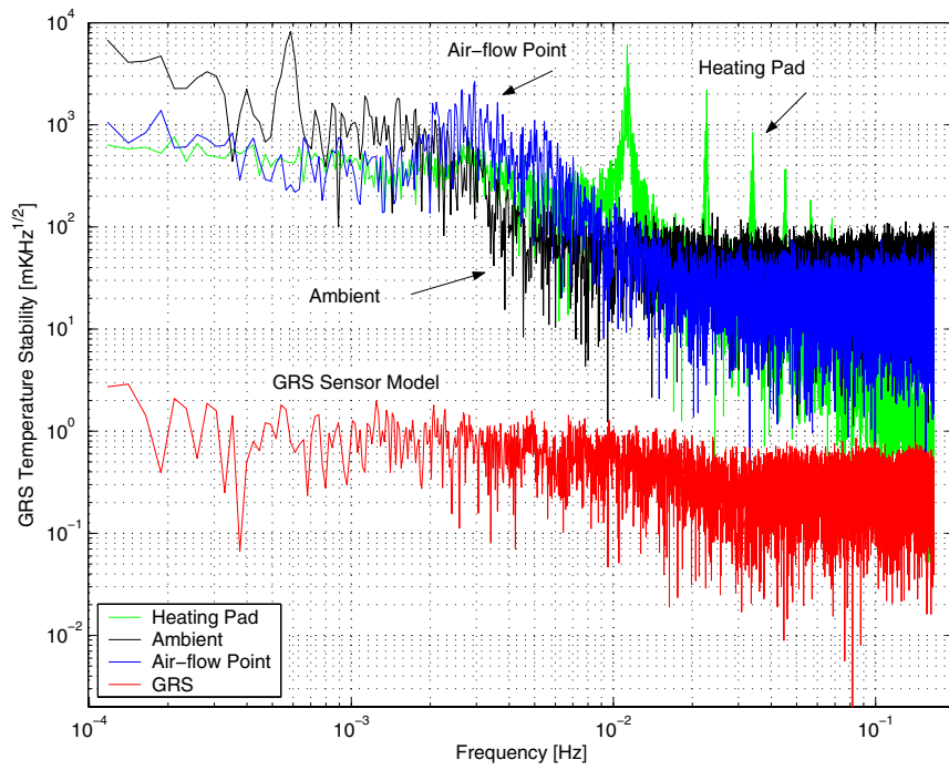
Figure 5. Thermal stability of the GRS system
