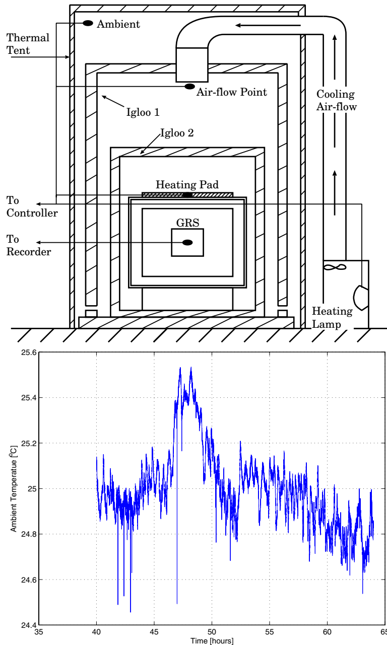
Figure 1. Schematic figure of the experiment (top), the ambient temperature variation (bottom)
