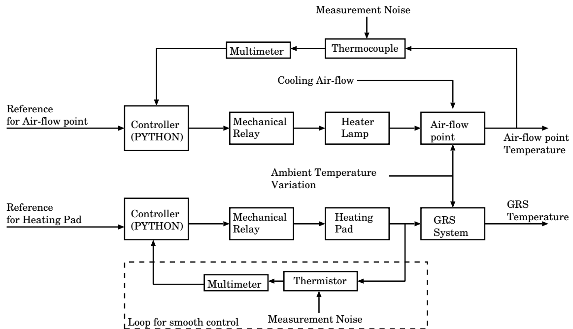
Figure 2. Control block diagram of the entire system
