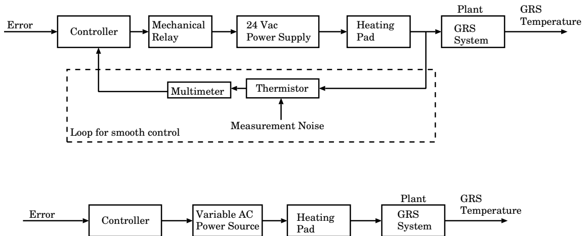
Figure 3. Smooth control using a mechanical relay and constant voltage source (top) and an ideal structure (bottom).
