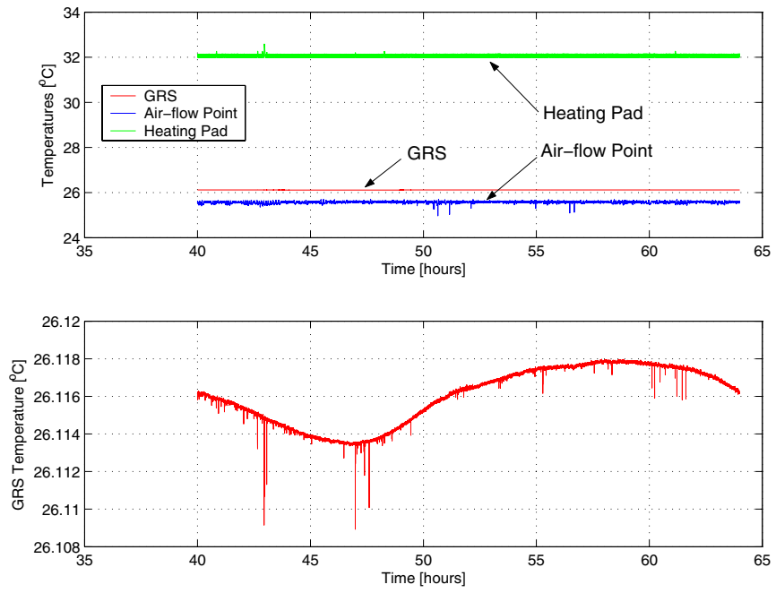
Figure 4. Time history of the GRS temperature: GRS, air-flow point, heating pad temperatures(top), GRS temperature (bottom)
