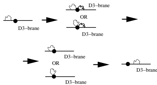
Figure 3. Schematic view of the capture process of an open string state, representing a photon propagating on a D3-brane world, by a D-particle on this world. The intermediate string state, indicated by thick wave lines, which is created on capture of the end(s) of the photon by the D-particle, stretches between the D-particle and the brane world, oscillates in size between 0 and a maximal length of order \alpha' p^0 , where p^0 is the energy of the incident photon, and thus produces a series of outgoing photon waves, with attenuating amplitudes, constituting the re-emission process. The intermediate string state provides also the restoring force, necessary for keeping the D-particle roughly in its position after scattering.
