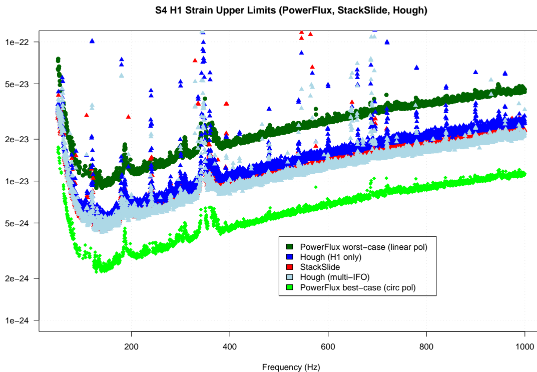
Figure 1. H1 upper limits on h_0 from the three methods. The StackSlide and Hough limits are population-based, while those from PowerFlux are strict and apply, respectively, to the most favorable and least favorable pulsar inclinations. Also shown are the multi-interferometer limits from the Hough search.
