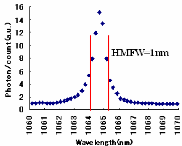
Figure 5. Spectrum of the measured output laser
