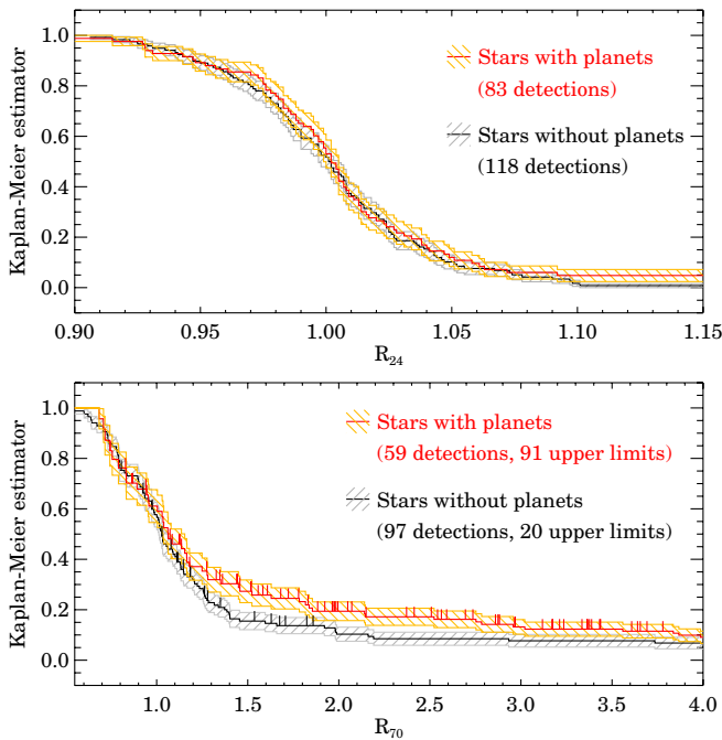
Figure 2. KM estimators for our two samples as a function of observed-to-photospheric flux ratio at 24\mu\text{m} (upper panel) and at 70\mu\text{m} (lower panel). Upper limits are indicated by vertical dashes. The KM estimator at a certain flux ratio gives the fraction of stars having a flux ratio larger than that value.
