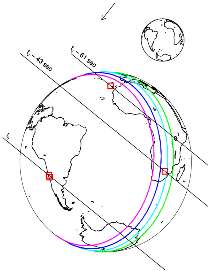
Figure 2. Reconstruction of microlens flyby. Upper figure: arrow defines locus of points from which lens and source appear perfectly aligned, passing just 1 Earth diameter from the Earth’s surface. Lower figure: Earth as seen from OGLE-2007-BLG-224 at the peak of the event. The red squares show the four observatories (in Chile, South Africa, and the Canaries) that observed near peak. The black diagonal lines show contours of constant peak time, with time offsets indicated between Chile and the other two locations. The green curve shows sunrise, while cyan, blue, and magenta curves show civil, nautical, and astronomical twilight. As shown in Figure 1, South Africa observations stopped 10 minutes before peak due to developing daylight.
