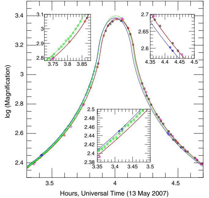
Figure 1. Light curve of OGLE-2007-BLG-224 during 1.4 hours closest to peak. Observatories in South Africa (Bronberg: green), Canaries (RoboNet LT: blue) and Chile (OGLE I : red, \mu\text{FUN} SMARTS I : magenta, \mu\text{FUN} SMARTS H : black) see significantly (several percent) different magnifications due to their different positions on the Earth. From these differences, one can infer that \tilde{r}_E (the projected Einstein radius) is about 10,000 Earth radii. The red and black curves (and points) deviate slightly over the peak because of different limb darkening of the source in I and H bands.
