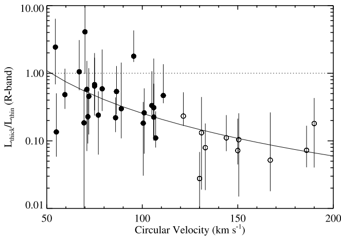
FIG. 18.—Ratio of the total R -band luminosity of the thick disk compared to the thin disk for the sample galaxies. The thin disk luminosities have been corrected for internal extinction. The dotted line indicates where the thick and thin disks contribute equally to the total luminosity. Error bars show the full range of values from different models and are indicative of our systematic errors. Galaxies with prominent dust lanes are plotted as open circles. The solid line is a fitted power law of the form L_{\text{thick}}/L_{\text{thin}} = 0.25(V_c/100 \text{ km s}^{-1})^{-2.1} .
