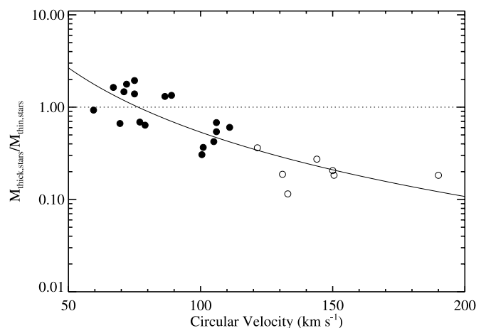
FIG. 22.—Stellar mass ratios of the thick and thin disks. The thin disks' luminosities and corresponding masses have been increased to account for dust extinction. Galaxies with prominent dust lanes are plotted as open circles. The solid line is a power-law fit (M_{\text{thick}}/M_{\text{thin}})_{\text{stars}} = 0.53(V_c/100 \text{ km s}^{-1})^{-2.3} .
