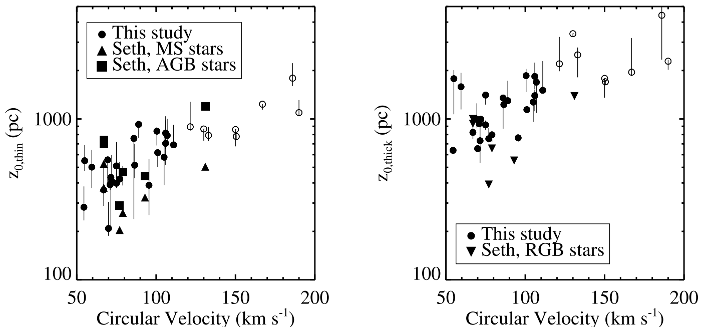
FIG. 12.—Comparison of our results with the scale heights of different stellar populations measured from resolved stars in six nearby galaxies (Seth et al. 2005b). The component we have identified as the thin disk appears to be intermediate between the scale height of young MS stars and medium-age AGB stars, while our thick disk component is similar to the old RGB populations. [See the electronic edition of the Journal for a color version of this figure.]
