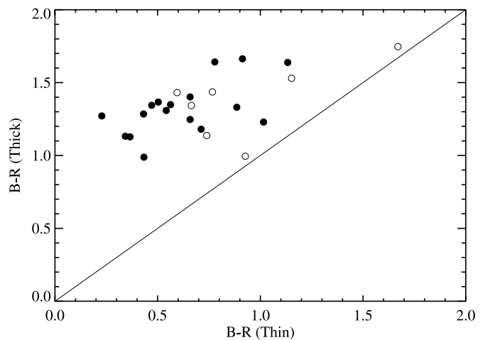
FIG. 21.—Comparison of thin and thick disk colors. The diagonal line indicates where the two components have equal color. Thin disk colors have been corrected for internal extinction. Open circles show galaxies with dust lanes.
