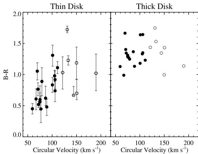
FIG. 20.—Extracted colors for the thick and thin disks. The thin disk colors show the full range of B-R values for the midplane between h_R < R < 3h_R . The thin disk has been corrected for internal extinction, but we assume no correction for the thick disk. Open circles show galaxies with dust lanes.
