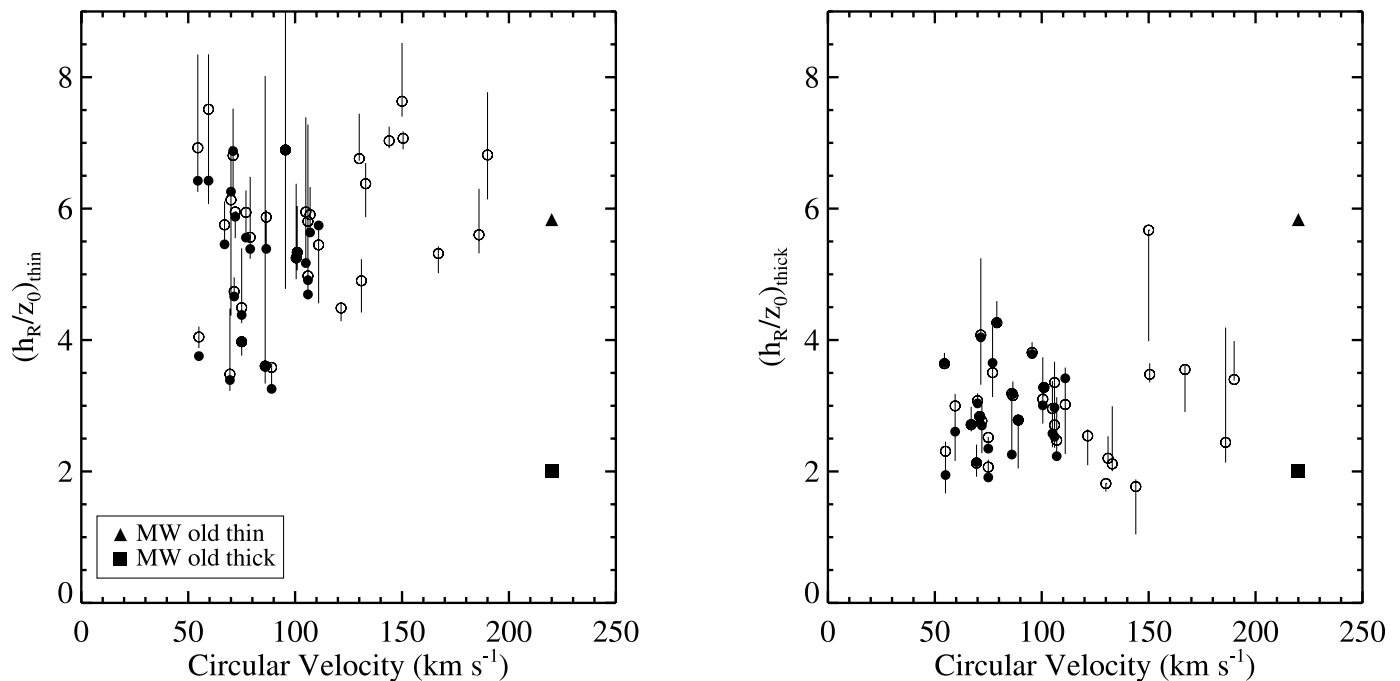
FIG. 16.—Axial ratio ( h_R/z_0 ) vs. circular velocity for the thin ( left ) and thick ( right ) disks. Galaxies with prominent dust lanes are plotted as open circles. The axial ratios of MW disk components are plotted for comparison (Table 5). The axial ratios of our thin and thick disks agree well with the comparable components for the MW. [See the electronic edition of the Journal for a color version of this figure.]
