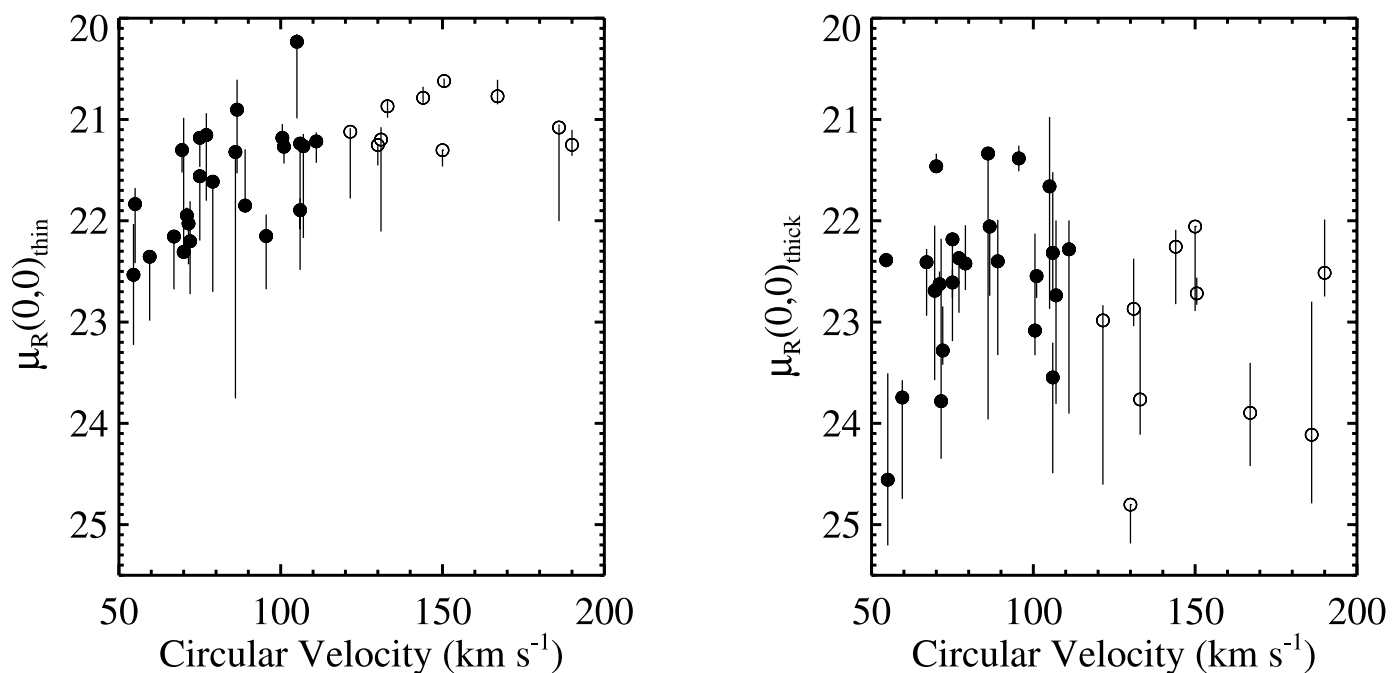
FIG. 17.—Edge-on peak surface brightnesses for the two-disk fits in the R band. Galaxies with prominent dust lanes are plotted as open circles.
