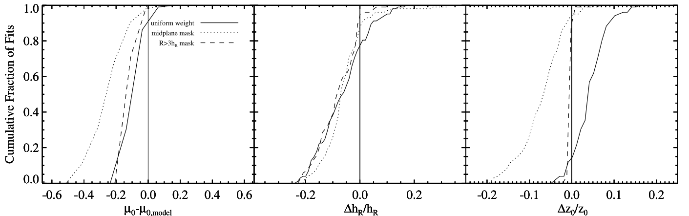
FIG. 1.—Cumulative distributions showing the systematic effects of fitting our galaxies with varying models. All models are compared to a fit using inverse weighting and no masked regions. Fits for all three filters have been combined. The solid curve shows the model that used uniform pixel weighting, while the dotted curve shows the midplane masked model, and the dashed curve shows the |R| > 3h_r radially masked model.
