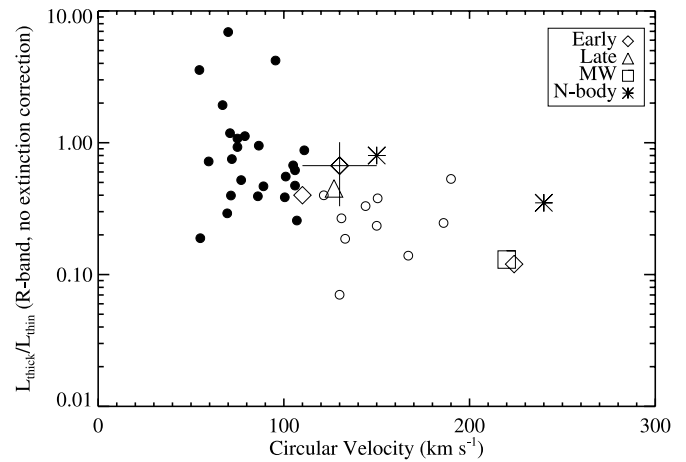
FIG. 19.—Comparison of our luminosity ratios to others in the literature. Comparison points are the same as Fig. 11. Unlike Fig. 18, we have made no correction of internal extinction to allow for easier comparison with previous studies. [See the electronic edition of the Journal for a color version of this figure.]
