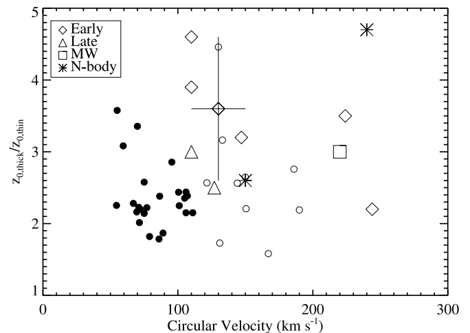
FIG. 11.—Comparison of our scale height ratios to values drawn from the literature. We compare to early-type galaxies (Sb and earlier; diamonds), late-type galaxies (Sc and Sd; triangles), the MW (square), and simulated galaxies (asterisks). The range of values available for the Pohlen et al. (2004) sample of early-type galaxies is plotted as the single point with error bars. [See the electronic edition of the Journal for a color version of this figure.]
