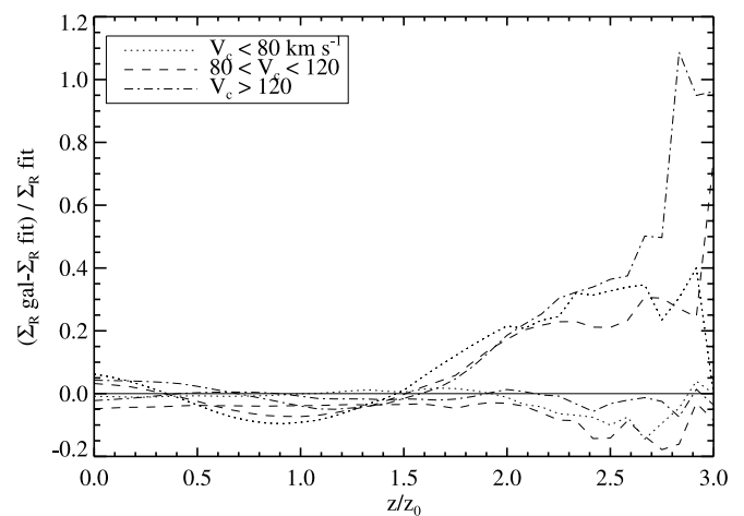
FIG. 7.—Residuals collapsed along the radial direction and averaged over galaxies binned by mass. The single-disk models (top three lines at right) are very poor fits, leaving large amounts of excess flux at high latitudes. The two-disk models (bottom three lines at right) do a much better job fitting the vertical light distribution at all latitudes and show only a small systematic trend to oversubtract at high z . [See the electronic edition of the Journal for a color version of this figure.]
