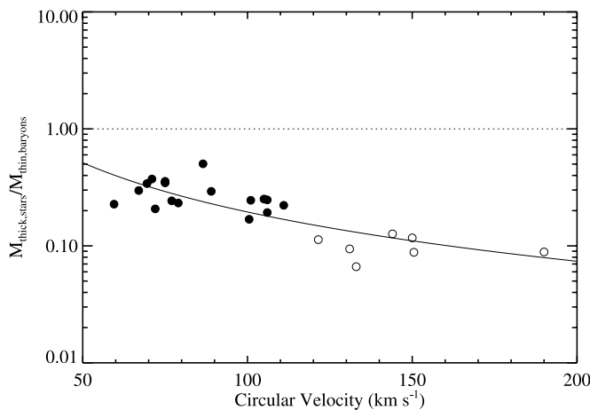
FIG. 23.—Baryonic mass ratios of the thick and thin disks. The thin disks' luminosities, and corresponding masses, have been increased to account for extinction effects and include the estimated thin disk mass stored in gas. Galaxies with prominent dust lanes are plotted as open circles. The solid line is a power-law fit M_{\text{thick,stars}}/M_{\text{thin,baryons}} = 0.19(V_c/100 \text{ km s}^{-1})^{-1.4} .
