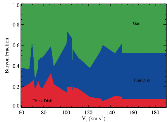
FIG. 24.—Final baryon fractions of the thick and thin components as a function of maximum velocity. The thin disk has been corrected for internal dust extinction. The baryonic mass fraction of the thick disk clearly increases toward lower galaxy mass.
