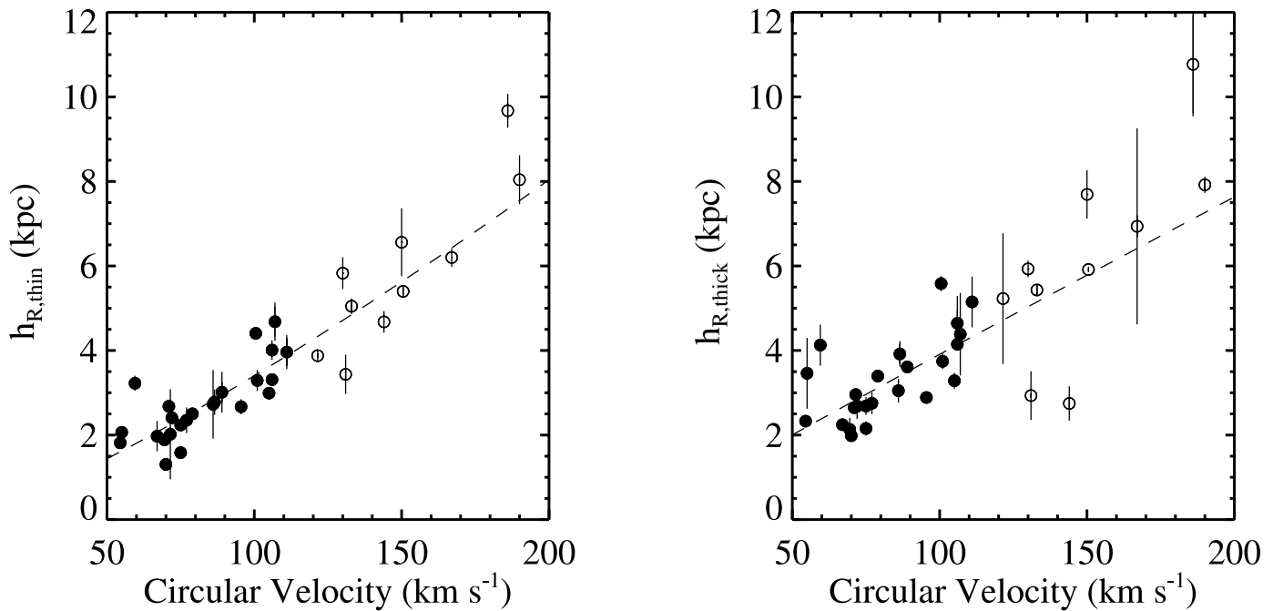
FIG. 13.—Scale lengths of thick and thin disks from the two-disk fits. Open symbols are used for galaxies with prominent dust lanes. The lines show power-law fits of h_{R,\text{thin}} = 3.40(V_c/100 \text{ km s}^{-1})^{1.2} \text{ kpc} and h_{R,\text{thick}} = 3.9(V_c/100 \text{ km s}^{-1})^{1.0} \text{ kpc} .
