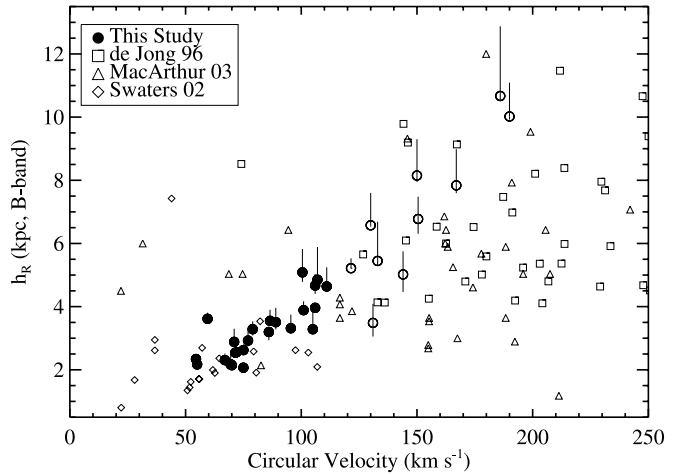
FIG. 3.—Single-disk scale lengths for the R -band (left) and B -band (right) fits. Galaxies with prominent dust lanes are plotted with open circles. For comparison, we show other single-disk fits gathered from the literature. The de Jong (1996) and MacArthur et al. (2003) data are face-on or moderately inclined galaxy samples with the scale lengths measured in the R and B bands (squares, left, and triangles, respectively). The Swaters & Balcells (2002) sample consists of late-type spiral and irregular galaxies with scale lengths measured in the R and B bands (diamonds). The Kregel et al. (2002) data were measured from edge-on galaxies in the R band (squares, left). [See the electronic edition of the Journal for a color version of this figure.]
