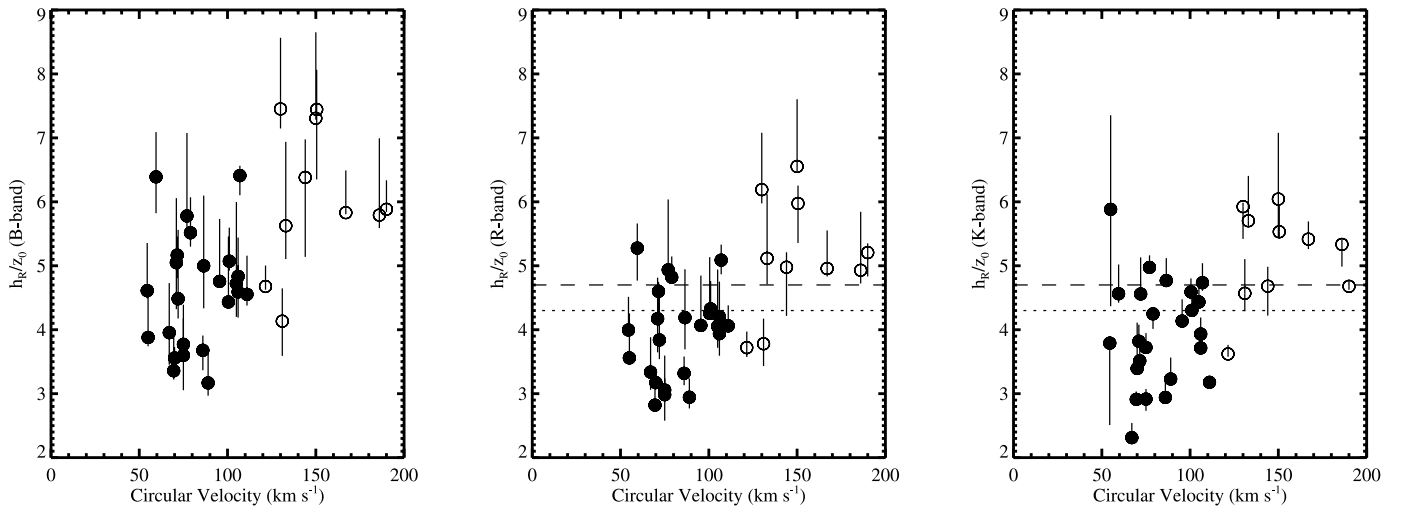
FIG. 5.—Single-disk fits showing the flatness ( h_R/z_0 ) for each band. Open symbols are used for galaxies with prominent dust lanes. Dotted lines show the average flatness for a sample of 34 galaxies in the I band presented in Kregel et al. (2002). Dashed lines show the average flatness measured from a sample of 153 galaxies from the Revised Flat Galaxy Catalog imaged by 2MASS in the K band and presented in Bizyaev & Mitronova (2002).
