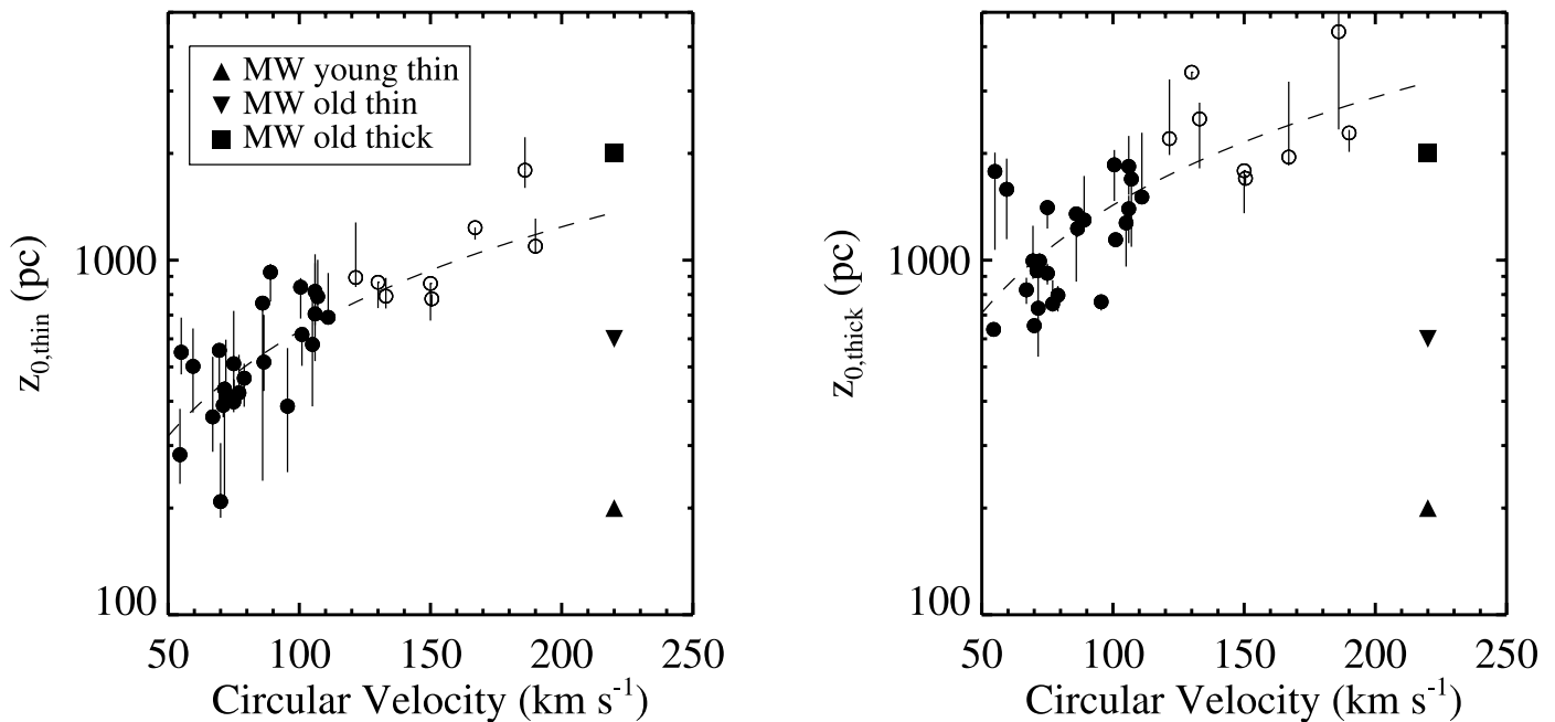
FIG. 9.—Scale heights of thin and thick disks. Values for the MW from Larsen & Humphreys (2003) are plotted for comparison using z_0 = 2h_z for an exponential vertical profile. Open symbols are used for galaxies with prominent dust lanes. Dashed lines show power-law fits to the data [ z_{0,\text{thin}} = (610 \text{ pc})(V_c/100 \text{ km s}^{-1})^{0.90} and z_{0,\text{thick}} = (1400 \text{ pc})(V_c/100 \text{ km s}^{-1})^{1.0} ]. In galaxies that have strong dust lanes, the scale height of the thin disk is likely to be biased toward larger values. [See the electronic edition of the Journal for a color version of this figure.]
