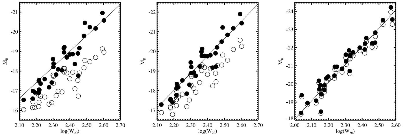
FIG. 8.—TF relation derived from the single-disk fits. Open circles show points uncorrected for internal extinction, while filled circles have been corrected for internal extinction using the method of Tully et al. (1998). Solid lines in the left and middle panels show TF relations from the Hubble Key Project (Sakai et al. 2000). The solid line in the right panel shows the K' TF relation of Verheijen (2001). The luminosities for the two-disk fits show a comparable offset.
