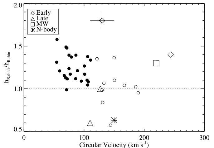
FIG. 15.—Comparison of our scale height ratios to values drawn from the literature. Comparison points are the same as in Fig. 11. [See the electronic edition of the Journal for a color version of this figure.]
