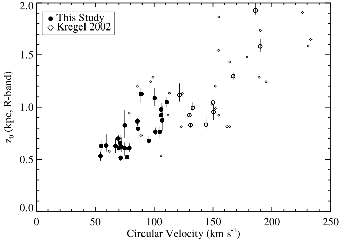
FIG. 2.—Single-disk scale heights for the R -band fits. Galaxies with prominent dust lanes are plotted with open circles. For comparison, we show the I -band scale heights from the edge-on sample of Kregel et al. (2002), plotted as diamonds. [See the electronic edition of the Journal for a color version of this figure.]
