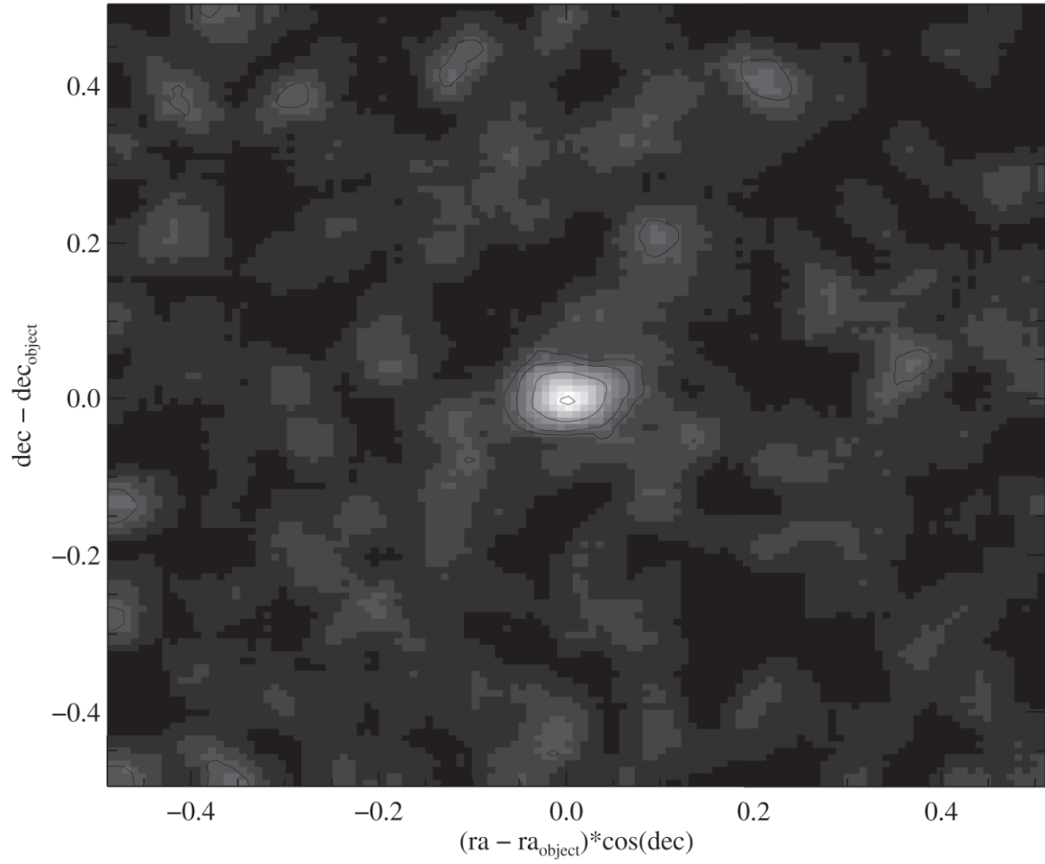
FIG. 2.—Smoothed image of stars with g - r < 0.65 and in a 0.5^\circ \times 0.5^\circ field centered on the detection. The contours represent smoothed stellar densities of 3, 5, 10, and 20 \sigma above the foreground.
