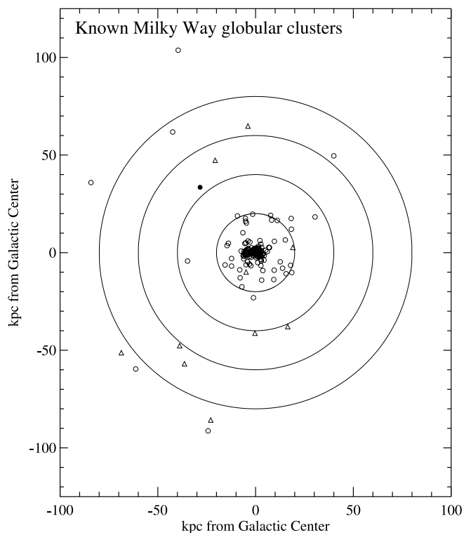
FIG. 7.—Spatial distribution of the (X, Z) positions of 150 known GCs (open circles; Harris 1996), 10 known nearby dwarfs (triangles; Mateo 1998), and the new companion (filled circle). The large circles show projected galactocentric distances of 20, 40, 60, and 80 kpc. The Galactic disk is oriented perpendicular to the y -axis.
