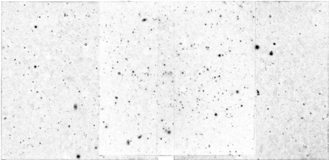
FIG. 3.—APO true-color g, r image of 0.2^\circ \times 0.075^\circ centered on the detection. [See the electronic edition of the Journal for a color version of this figure.]
