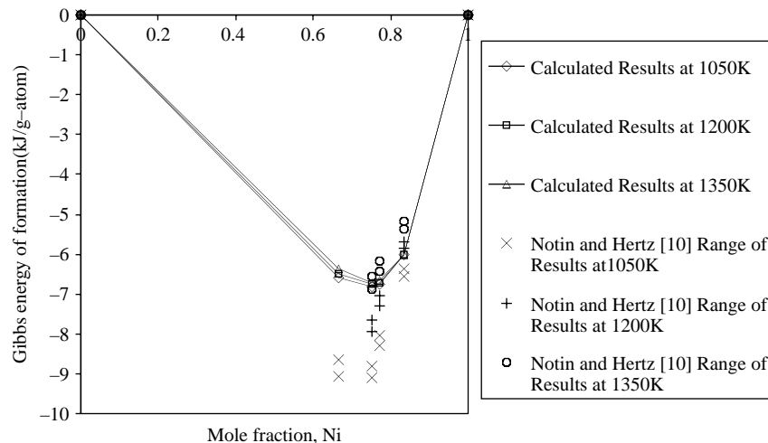
Fig. 5. Comparison between the calculated Gibbs energy of formation and experimental results from the literature.
