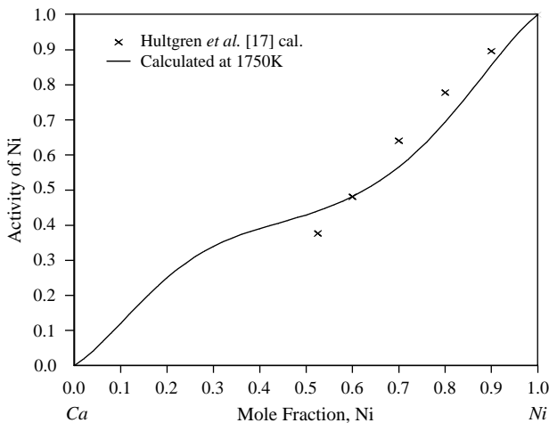
Fig. 8. Activity of Ni in liquid Ca–Ni at 1750 K.
