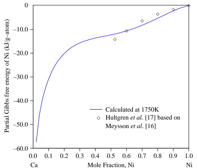
Fig. 10. Gibbs partial energy of Ni at 1750 K.
