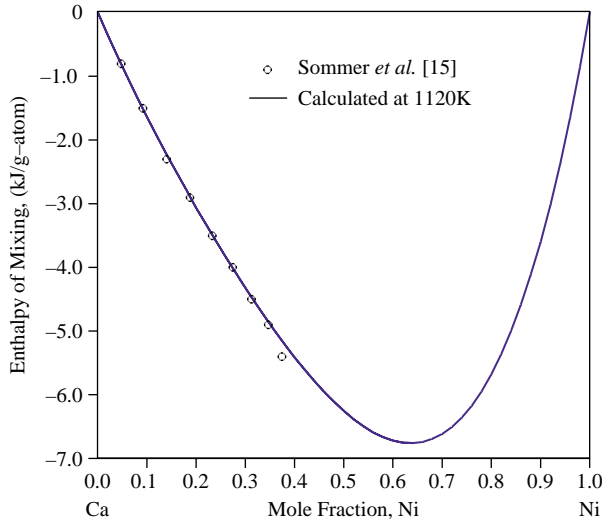
Fig. 6. Enthalpy of mixing of liquid Ca–Ni at 1120 K.
