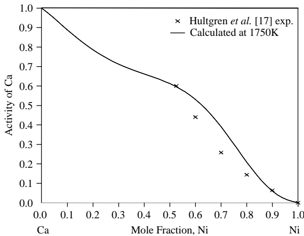
Fig. 7. Activity of Ca in liquid Ca–Ni at 1750 K.
