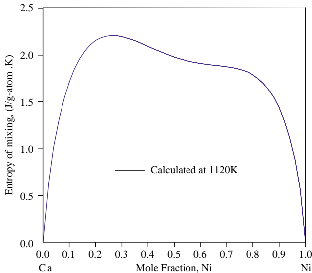
Fig. 11. Entropy of mixing of liquid Ca–Ni at 1120 K.
