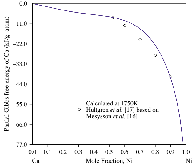
Fig. 9. Gibbs partial energy of Ca at 1750 K.
