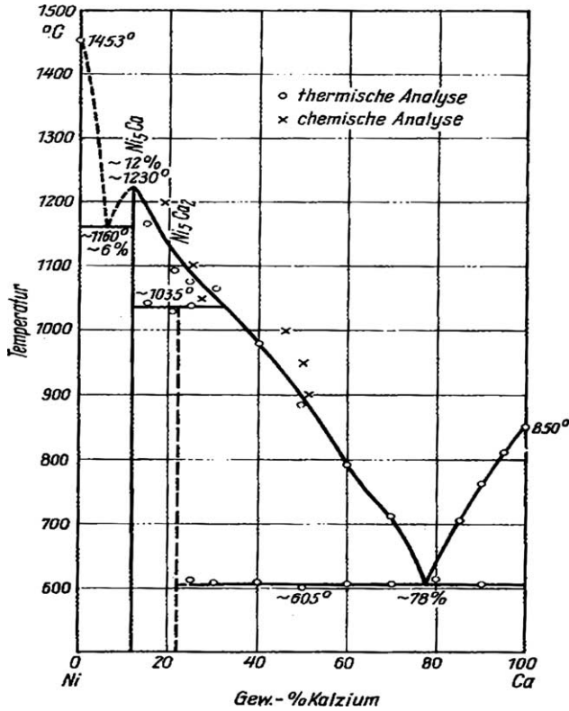
Fig. 1. Ca–Ni phase diagram Takeuchi et al. [6].
