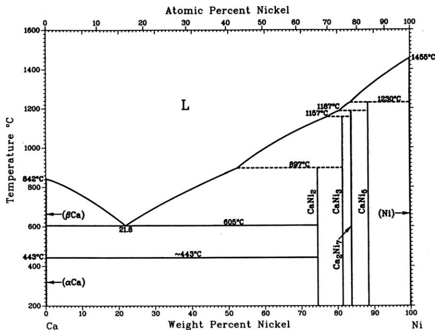
Fig. 2. Ca–Ni phase diagram Okamoto [11].
