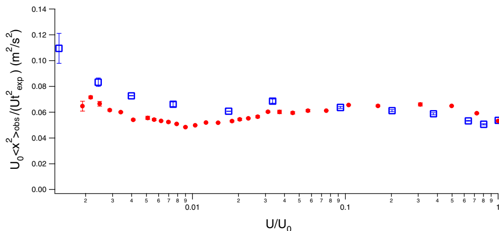
Figure 2. Mean square cloud size in the trap, which is nearly independent of trap depth. Red solid circles: obtained using the trap lowering curve for an energy-independent scattering cross-section. Blue open squares: obtained using the trap lowering curve for unitary gas. Note that the trap lowering time increases from right to left.
