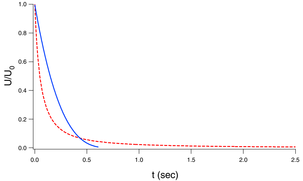
Figure 3. Trap depth U/U_0 versus time. Red dashed line: lowering curve for an energy-independent scattering cross-section. Blue solid line: lowering curve for a unitary gas. Each curve ends when U/U_0 = 1/150 , where the gas becomes quantum degenerate.
