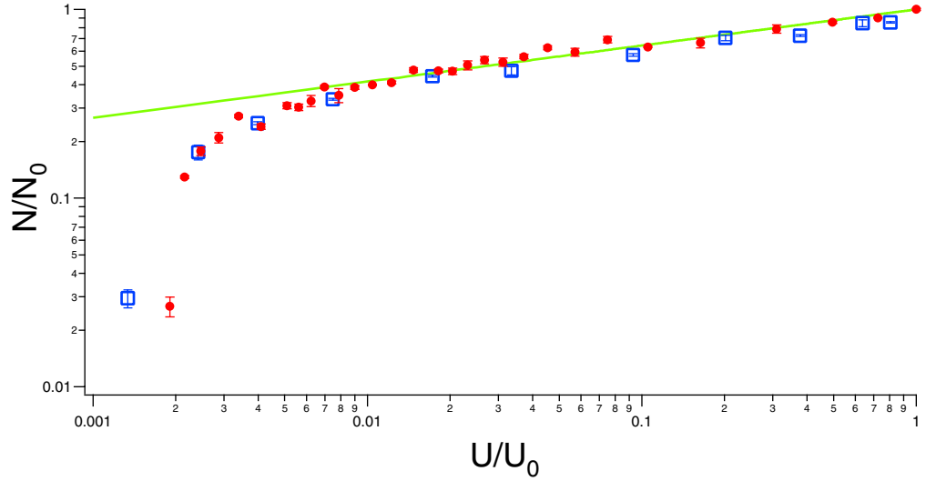
Figure 1. Atom number versus trap depth. The solid green line shows the scaling law prediction for \eta = U/k_B T = 10 . Note that the data deviate from the scaling law prediction when the gas becomes degenerate, near U/U_0 = 0.007 . Red solid circles: obtained using a trap lowering curve for an energy-independent scattering cross-section. Blue open squares: obtained using the trap lowering curve for unitary gas. Note that trap lowering time increases from right to left.
