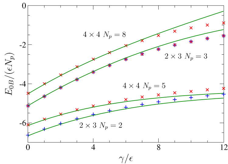
Figure 1. Ground-state energy per particle for the hard-core boson FNU model versus the interaction strength \gamma . The results from equation (28) (—) are compared with those from exact diagonalizations (+) and QMC simulations ( \times ) for two-dimensional systems with periodic boundary conditions and different L_x \times L_y sites and N_\uparrow = N_\downarrow = N_p particles. The statistical errors in the QMC data are negligible in this scale.
