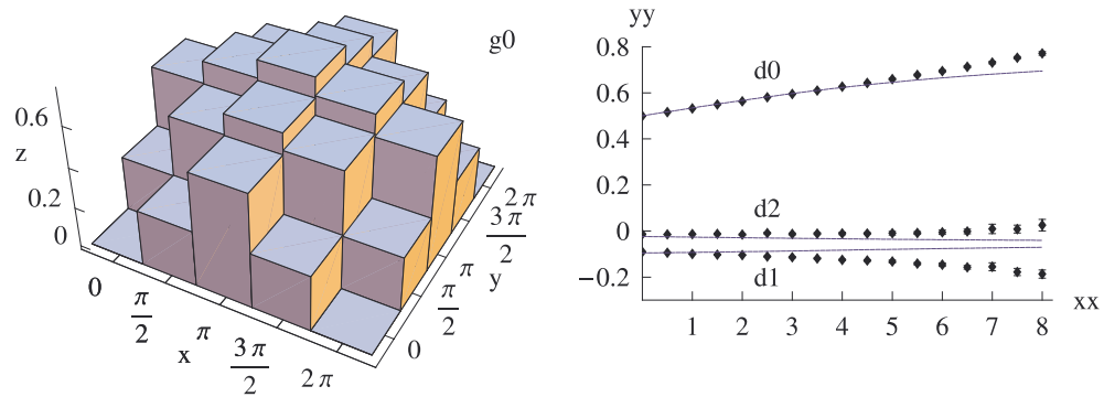
Figure 3. Spin–spin structure factor S(q_x, q_y) for the hard-core boson FNU model at \gamma = 0 in a lattice with 4 \times 4 sites, N_\uparrow = N_\downarrow = 8 particles and periodic boundary conditions. For the same system, on the right plot, we show the values of the ground-state expectation of the operators S_i S_j for d_{ij} = 0, 1, 2 as a function of the interaction strength \gamma (solid lines) compared with Monte Carlo results (dots with error bars).
