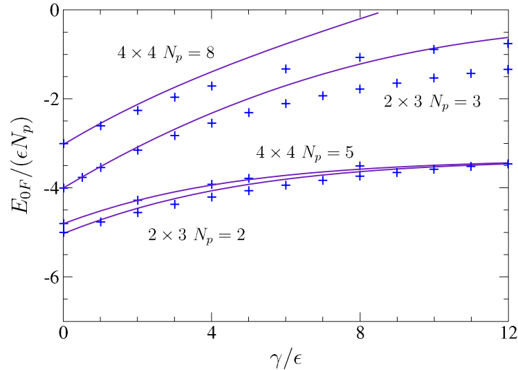
Figure 2. As in figure 1 for the fermion FNU model. In this case no QMC simulations are available. Exact diagonalization data for the 4 \times 4 systems are taken from [15] ( N_p = 8 ) and [16, 17] ( N_p = 5 ).
