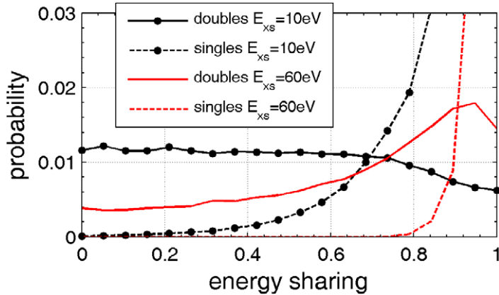
Figure 4. The double ionization probability as a function of energy sharing averaged over all phases \phi when the streaking field is on separately for the ‘double’ and ‘single’ events for 10 eV/60 eV excess energy. The area under the ‘double’ events is 0.011/0.0084, whereas the area under the ‘single’ events is 0.013/0.0106. The sum of the two contributions is the total double ionization probability in the presence of the XUV attosecond pulse and the streaking field.
