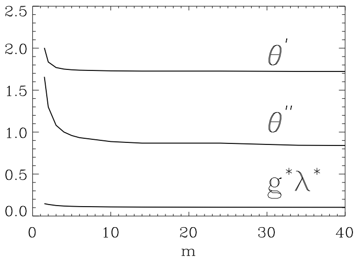
Figure 1: The universal quantities \theta', \theta'' , and \lambda^*g^* as a function of the regulator parameter m .
