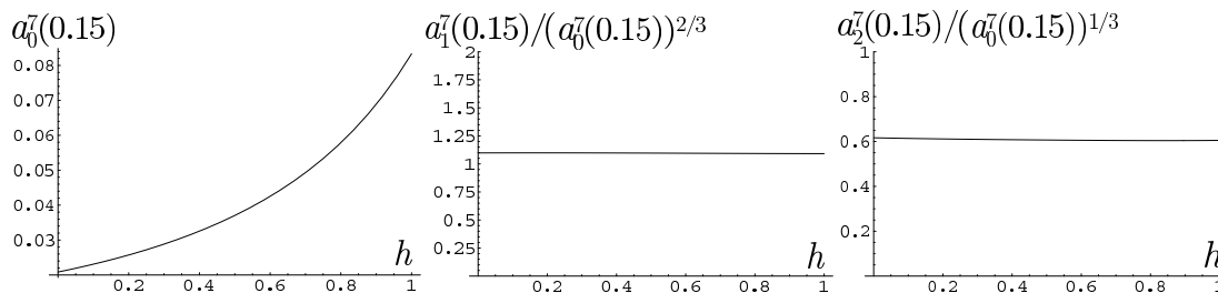
Figure 4: The h -dependence of a_0^7(0.15) , a_1^7(0.15)/(a_0^7(0.15))^{2/3} and a_2^7(0.15)/(a_0^7(0.15))^{1/3} is plotted for a fuzzy CP^3 . The latter two take almost constant values.
