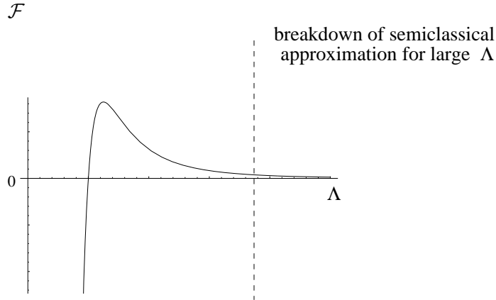
Figure 3: \mathcal{F} as a function of \Lambda . The semi-classical approximation breaks down (indicated by the dashed vertical line at the right) when \Lambda is large.
