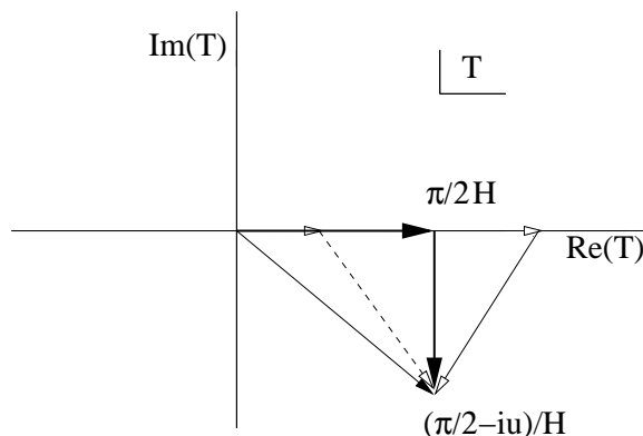
Figure 5: The 4 paths for T = 0 to T = (\pi/2 - iu)/H discussed in the text, from left to right: w = 0 , 0 < w < \pi/2H , w = \pi/2H and w > \pi/2H . Actually, there are infinitely many paths reachable simply by analytic continuation. Here \cosh u = \hat{a}H .
