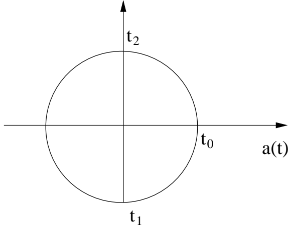
Figure 7: S^4 instanton.
