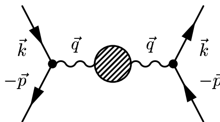
Figure 4: The lowest order medium contribution to dilepton production. The dashed blob represents the \mathcal{O}(e^2) in-medium photon polarization tensor. Lepton momenta follow the fermionic flow.
