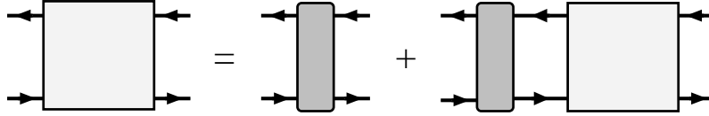
Figure 7: The Bethe-Salpeter equation for the four-point function \Gamma^{(4)} (grey box) in a theory with quartic interactions. The lines represent the full propagator of the theory ( D_\psi ) and the dark grey box corresponds to the kernel \Lambda of this integral equation (see text).
