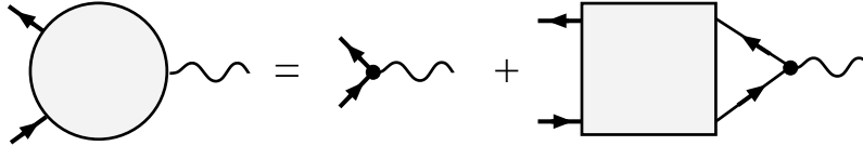
Figure 8: Definition of the resummed vertex V^\mu (grey circle) in terms of the bare vertex ( \gamma^\mu ) and the amputated four-point function \Gamma^{(4)} (grey square).
