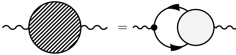
Figure 9: The non-equilibrium photon polarization tensor \Pi^{\mu\nu} expressed in terms of the resummed vertex V^\mu (grey circle).
