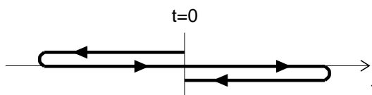
Figure 5: The \mathcal{S} -path in real time.
