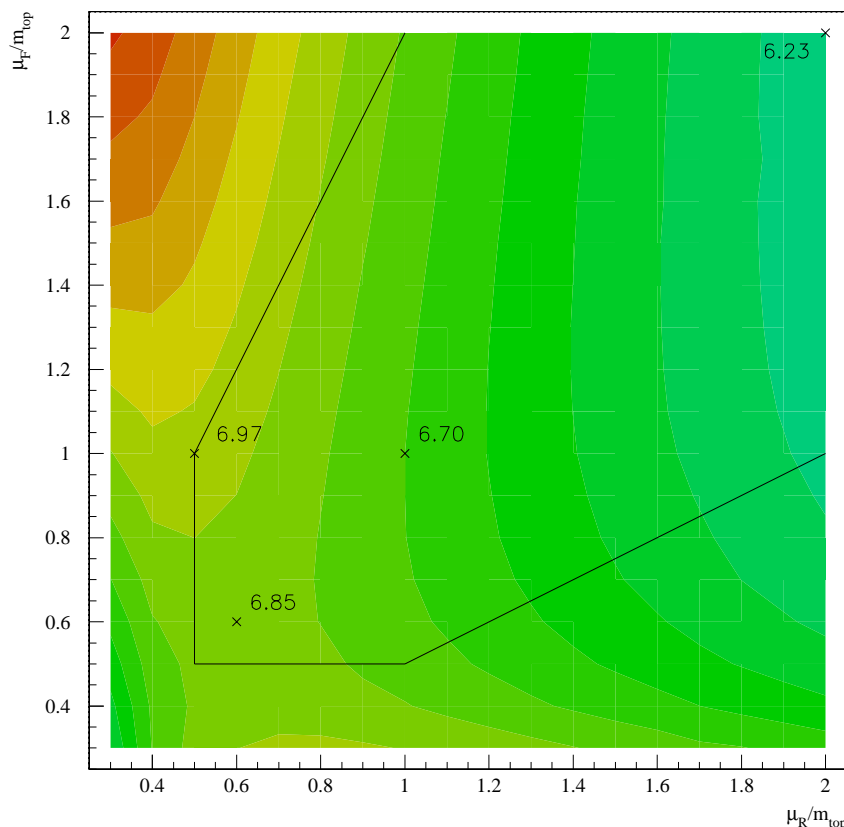
Figure 1: Contour plot of the NLL cross-section, in the \mu_F - \mu_R plane. The oblique solid line defines the region 0.5 < \mu_R/\mu_F < 2 .
