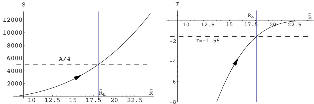
(a) The entropy crossing L as a function of \bar{R} . (b) A plot of the light sheet L in (T, \bar{R}) coordinates.
