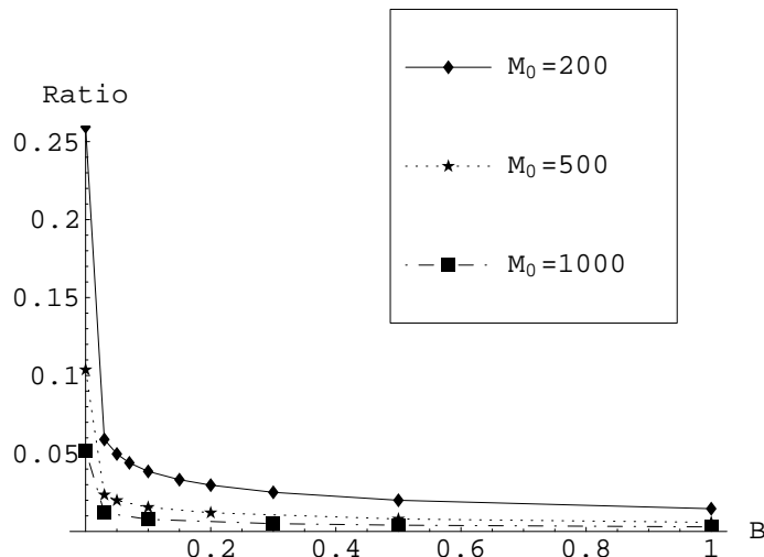
Figure 3: It is plotted the Ratio \equiv 4S/A as a function of the inhomogeneity parameter B , for three different large values of M_0 . One sees that the entropy bound is satisfied for large values of M_0 .
