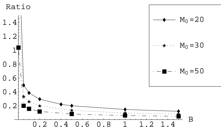
Figure 4: It is plotted the Ratio \equiv 4S/A as a function of the inhomogeneity parameter B , for three different small values of M_0 . For M_0 < 50 , violations occur at small values of B .
