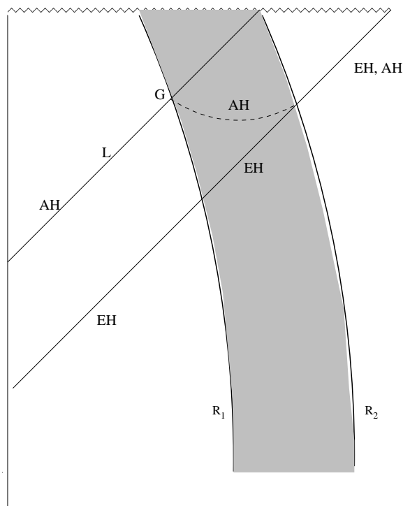
Figure 1: A Tolman-Bondi dust shell falling into a black hole. AH represents the apparent horizon and EH represents the event horizon.
