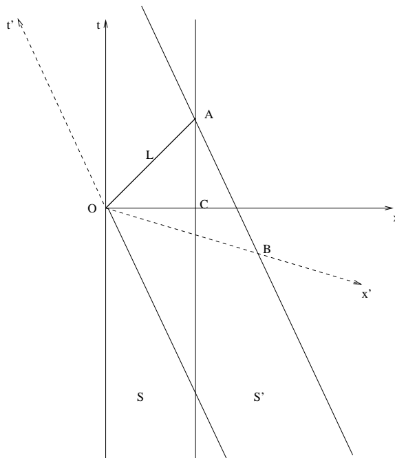
Figure 2: A spacetime diagram for observers in references S and S' passing through the light-sheet L in Minkowski spacetime, respectively. The proper distances between the two observers in S and S' are |OC| and |OB| , respectively.
