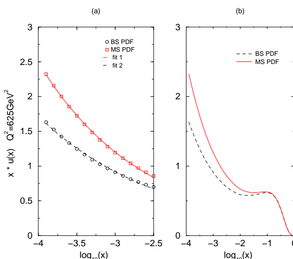
Figure 2: The left-hand graph gives the u -quark distribution at small x at Q^2 = 625 \text{ GeV}^2 . The lines are simple power law fits to the curves: xu(x) = 0.135x^{-0.32} and xu(x) = 0.14x^{-0.27} for the upper ( \overline{\text{MS}} ) and lower (BS scheme) curves. The inset gives the pdf at all x .
