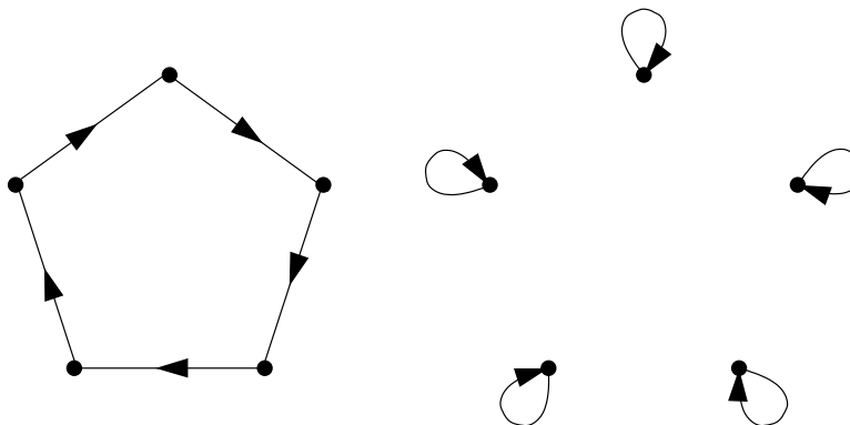
Figure 1: The \mathbb{C}^2/\mathbb{Z}_5 Moose. On the left is the moose for Z_{i,i+1}^1 , \bar{Z}_{i,i+1}^2 , and \bar{\eta}_{i,i+1} . On the right is the moose for A_{ii}^0 , X_{ii}^m , and \chi_{i,i} .
