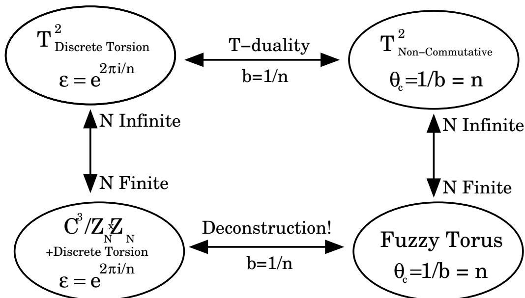
Figure 3: Deconstruction is T-Duality. Note that n \equiv m'/N . The scalings indicated are for fixed volume of the torus seen by closed strings.
