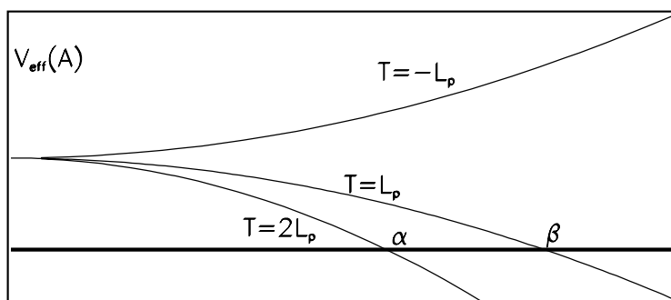
Figure 3: Effective potential V_{\text{eff}}(A) as a function of A with the AdS radius \ell = 1 . \alpha and \beta are turning points.
