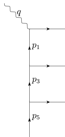
Figure 3: Generic initial-state shower.
