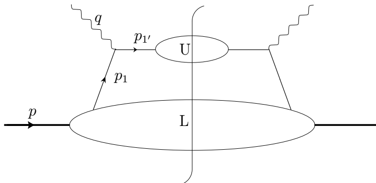
Figure 2: The parton model for deep inelastic scattering is derived from cut graphs of this form.
