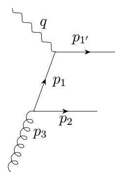
Figure 1: Photon-gluon fusion.
