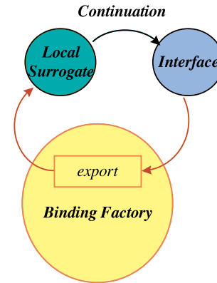
Figure 2. Exporting an interface.
