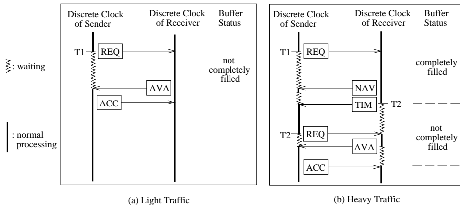
Figure 2. Hand-shaking protocols for packet transmission.
