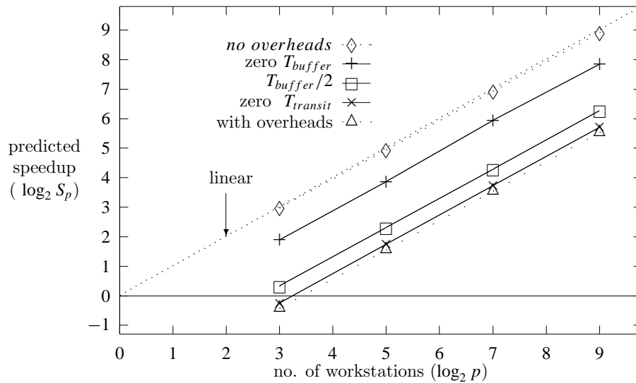
Figure 5. Speedup analysis (using MPS mapping scheme).
