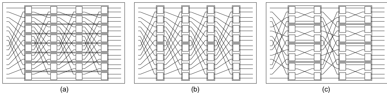
Figure 3. Mapping schemes for a finite number of workstations. (a) Horizontal partition, (b) vertical partition and (c) modular partition.
