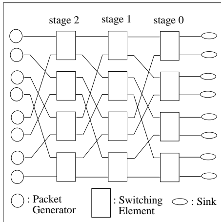
Figure 1. Components of MIN simulation.
