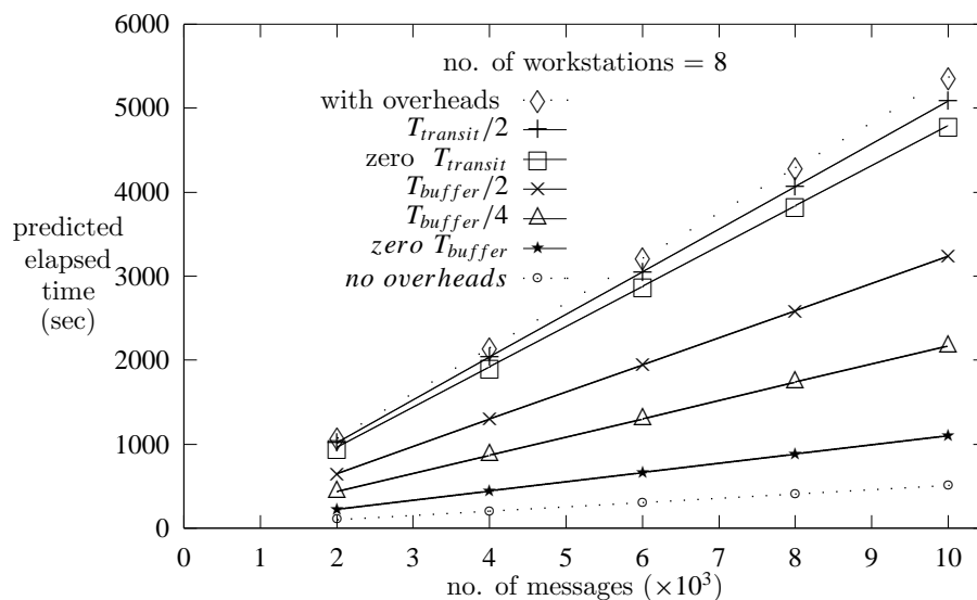
Figure 4. Elapsed time analysis (using MPS mapping scheme).
