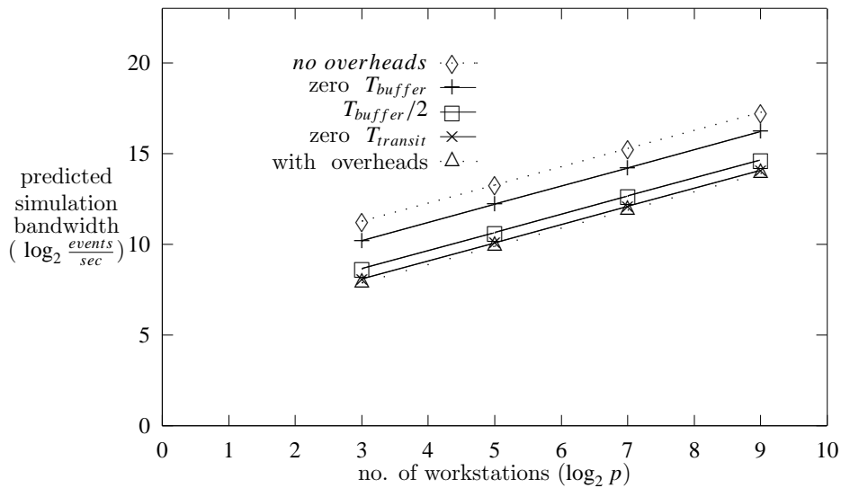
Figure 6. Simulation bandwidth analysis (using MPS mapping scheme).
