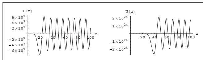
Fig. 5: Plots of \bar{U}_p(z) for p=1 , where we put m=0, 5 , \sqrt{3M^3}\lambda=20 (left) and \sqrt{3M^3}\lambda=40 (right).
