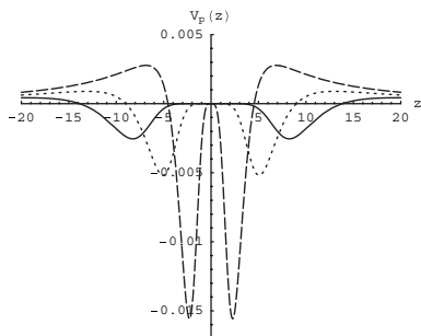
Fig. 3: Plots of the potential \bar{V}_p(z) with p=3 (dashed line), p=5 (dotted line) and p=7 (solid line). We have put \sqrt{3M^3}\lambda=2 .
