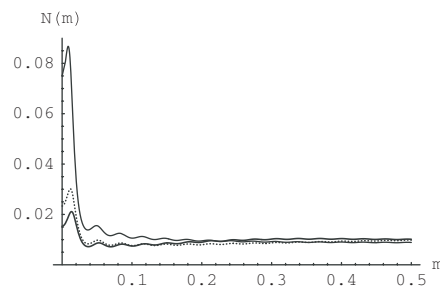
Fig. 6: Plots of N_p(m) for p=1 (thin line), p=3 (points) and p=5 (thick line). We use \sqrt{3M^3}\lambda=2 .
