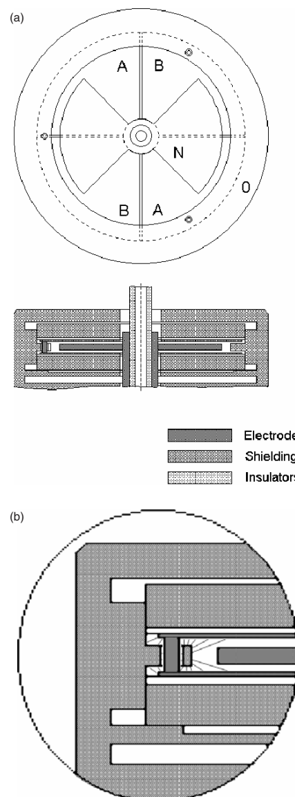
Figure 2. (a) Top view of the torque transmitter and a cross-section of one system. (b) A detail of the cross-section with some electric flux lines.
