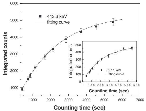
Figure 4. Integrated area of the 443.3 keV emission peak from the decay of ^{128}\text{I} measured as a function of time. The measured half-life is (25.8 \pm 1.0) minutes. Inset: The measured half-life of the 527.1 keV emission peak was determined to be (25.5 \pm 1.5) minutes. Both measurements agree well the literature value of 25 minutes for the half-life of ^{128}\text{I} .
