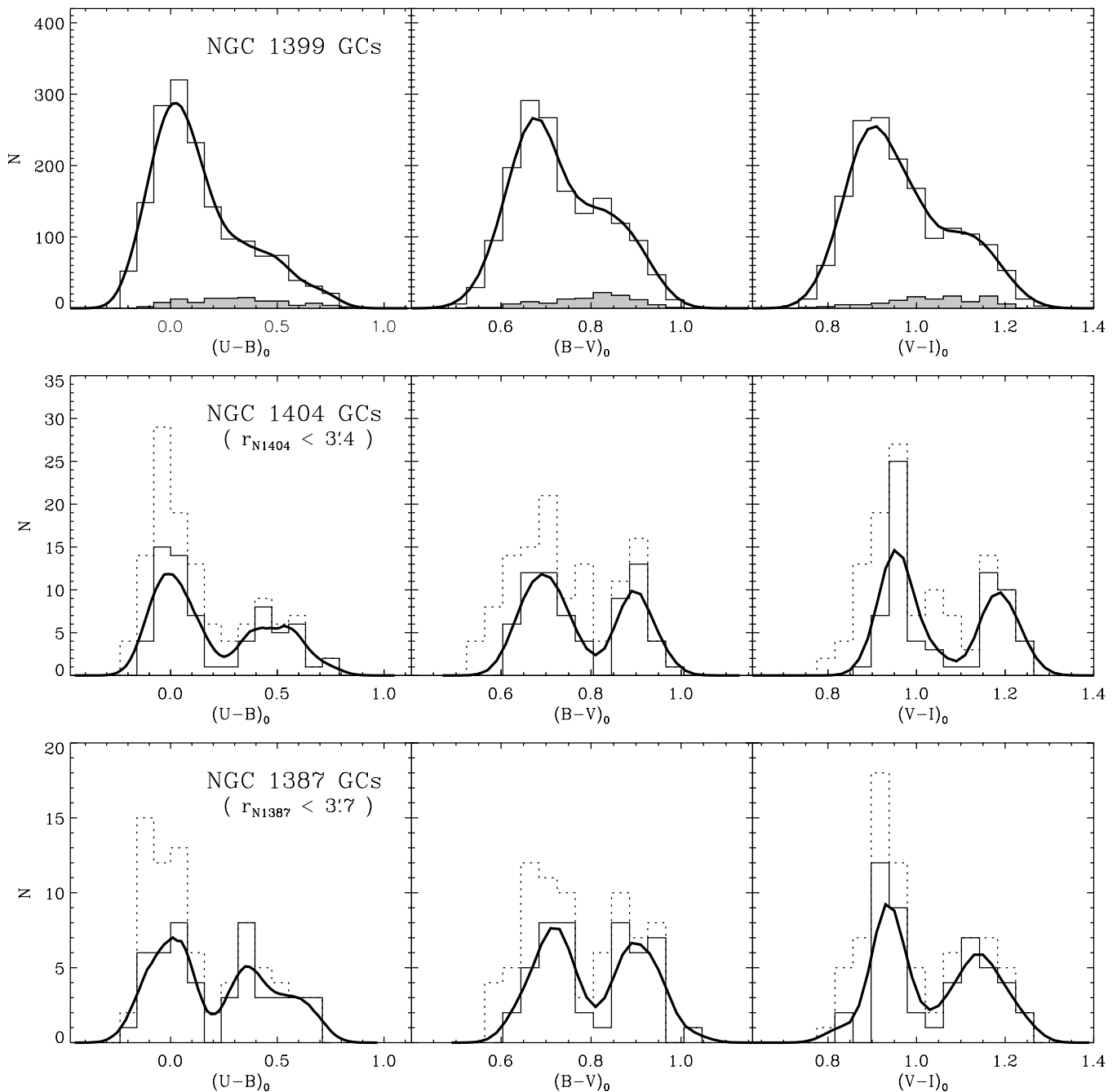
Figure 12. Color distributions of GCs in NGC 1399, NGC 1404, and NGC 1387. Thick solid lines are smoothed histograms with Gaussian kernels of \sigma(U-B) = 0.08 , \sigma(B-V) = 0.04 , and \sigma(V-I) = 0.04 , respectively. The \sigma values are set to be comparable to the mean errors in each color. Filled gray histograms in the top panels show the color distributions of the brightest GCs ( V_0 < 21.5 ). Dotted histograms in the middle and bottom panels represent the color histograms of entire set of GCs within the extent of each galaxy, and solid histograms show the “corrected” distributions for the contamination by NGC 1399 GCs (see the text).
