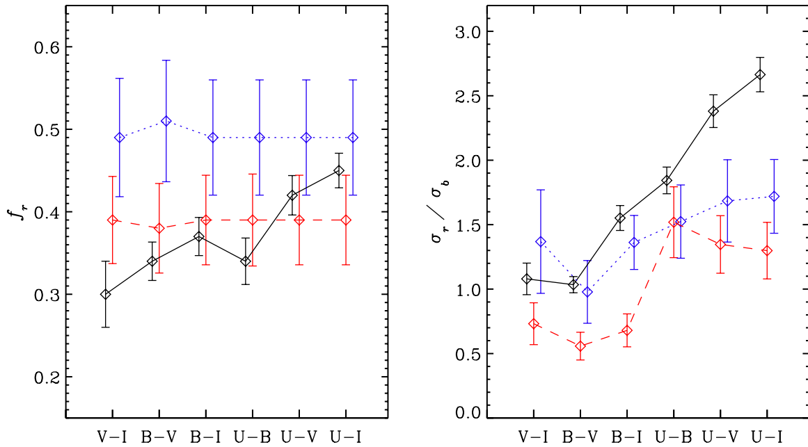
Figure 13. Variation in the red GC fractions (left) and the ratios of standard deviations between blue and red GC colors (right) for various colors. Solid black lines, dashed red lines, and dotted blue lines are for NGC 1399, NGC 1404, and NGC 1387, respectively. For NGC 1404 and NGC 1387, the values were derived from the corrected color distributions for the contribution of NGC 1399 GCs in Figure 12.
