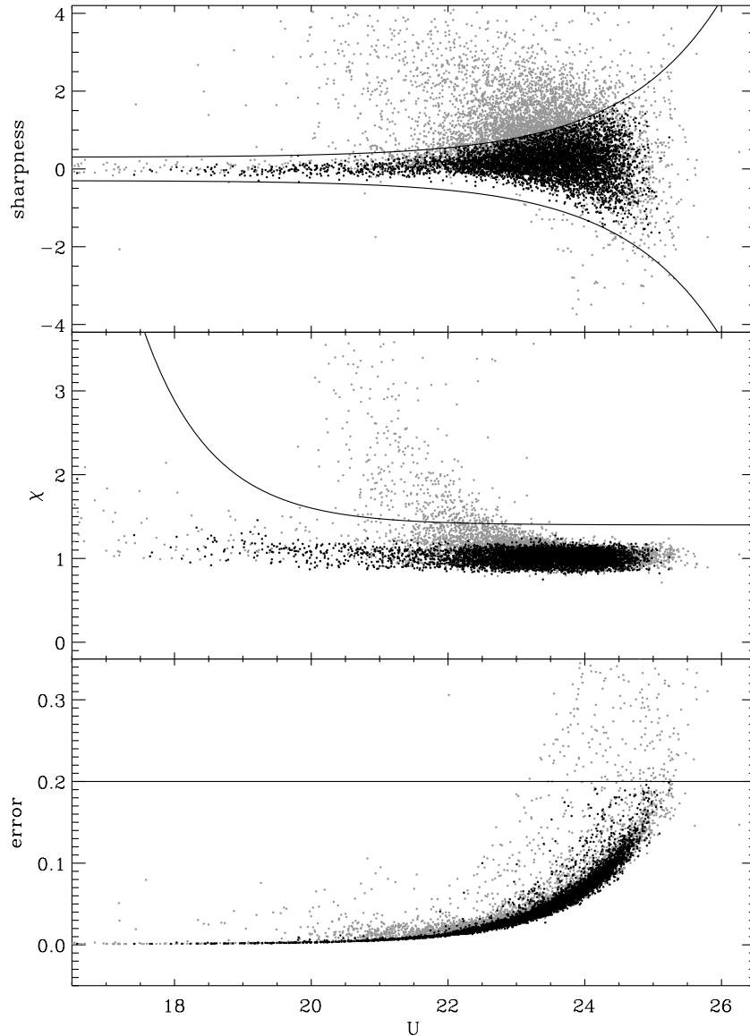
Figure 5. Photometric error and image parameters ( \chi and Sharpness ) in the U band as a function of magnitude. Solid lines show the point-source selection criteria. Black dots represent the selected sources with good photometry, while gray dots represent the sources that do not satisfy any of the selection criteria.
