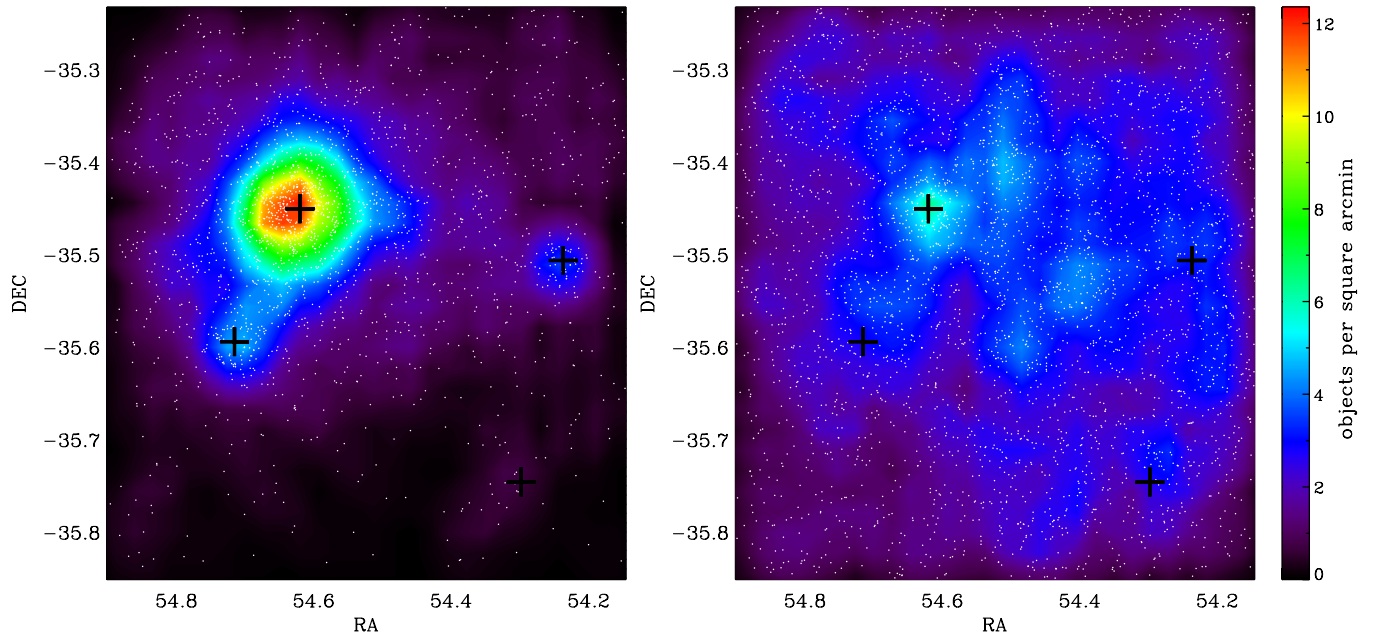
Figure 9. Spatial distribution of GC candidates (left) and foreground/background objects (right) over color-filled density contour maps with the color scale from black to red for increasing surface number density. Black crosses represent the positions of the optical centers of galaxies (from top, NGC 1399, NGC 1387, NGC 1404, and NGC 1389).
