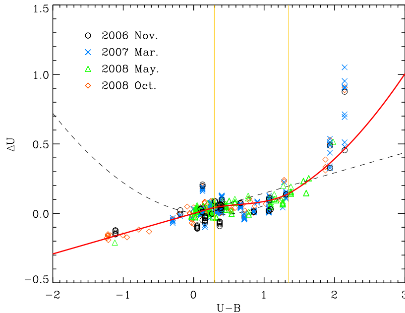
Figure 2. Difference between the standard and instrumental U magnitudes of standard stars after photometric zero point and atmospheric extinction corrections, as a function of U - B . In the calibration of U band, all the standard stars observed in subsequent observing runs during three years were used to derive a reliable solution. Different symbols are used to distinguish observations from different seasons. Two dashed lines represent error-weighted least-squares fits for blue and red standard stars, respectively. The solid red line represents the adopted best-fit function, which connects the two functions using internal division points of them between two vertical orange lines.
