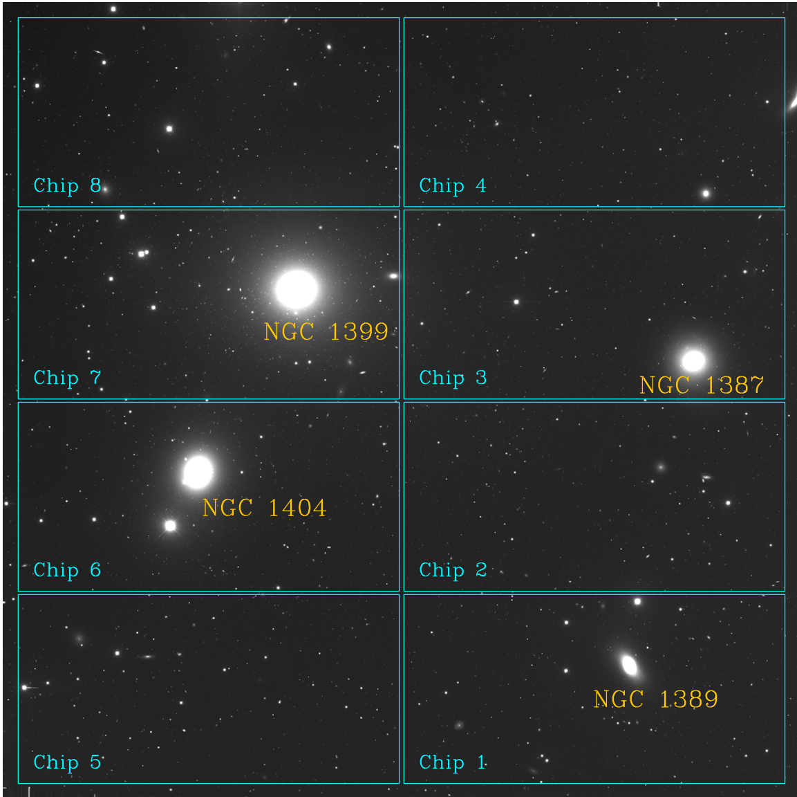
Figure 1. Median combined B -band image of our target field with the configuration of Mosaic II chips overlaid. The gaps between chips were filled in by creating mosaics using a three-point dither pattern. The image covers an area of 36' \times 36' , containing four Fornax cluster galaxies as labeled and their GC systems. North is up, and east is to the left.
