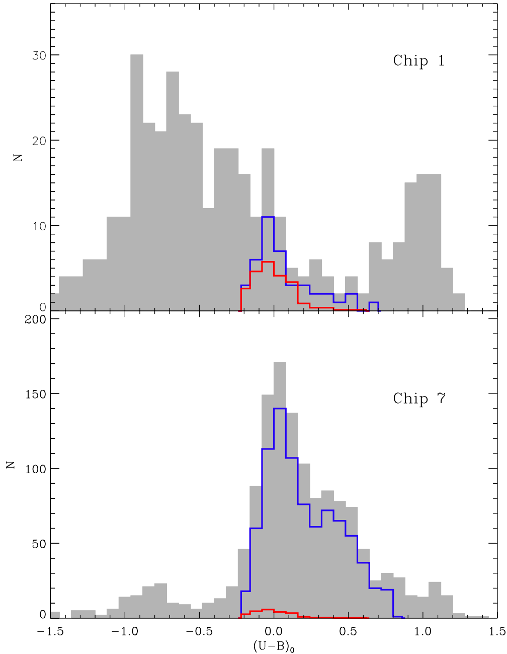
Figure 8. U - B color distributions for all point sources (shaded histogram), GC candidates (blue), and synthetic stars from Besançon model (red) in chip 1 and chip 7. The similarities found in the red and blue color distributions in the upper panel indicate that chip 1 is a good control field.
