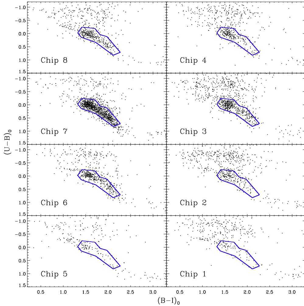
Figure 7. Color-color diagrams of point sources on each chip. Solid boxes indicate the selection criteria for the GC candidates and the chip numbers are indicated in the lower left corner of each panel. Chips 7, 6, and 3 contain NGC 1399, NGC 1404, and NGC 1387, respectively. Chip 1, which is located farthest away from the galaxies, is used to estimate the upper limit of the contamination level of our data.
