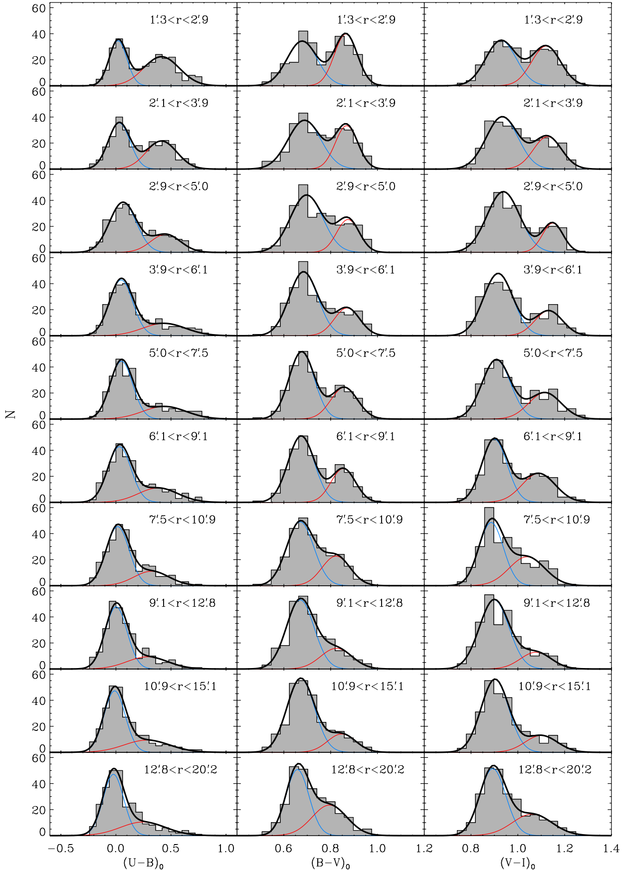
Figure 14. Histograms of (U - B)_0 , (B - V)_0 , and (V - I)_0 colors (left, middle, and right columns) for NGC 1399 GCs in various radial bins indicated in the upper right corner within each panel. The radial bins are defined to contain approximately equal numbers ( \sim 300 ) of GCs. The histograms are expressed by two (i.e., blue and red) Gaussian normal distributions based on GMM analysis. The blue, red, and black lines represent blue GCs, red GCs, and their sum, respectively.
