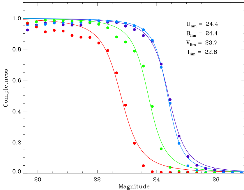
Figure 3. Completeness functions obtained from artificial star tests. Detection efficiencies (filled circle) were fitted to the analytic function by Fleming et al. (1995), which are denoted by solid lines. The purple, blue, green, and red lines represent the U , B , V , and I bands, respectively. The functions are for the overall image, except the galactic central regions and the gaps between mosaic chips where the detection efficiency rapidly drops. Limiting magnitudes where the completeness drops to 50% are indicated in the upper-right corner.
