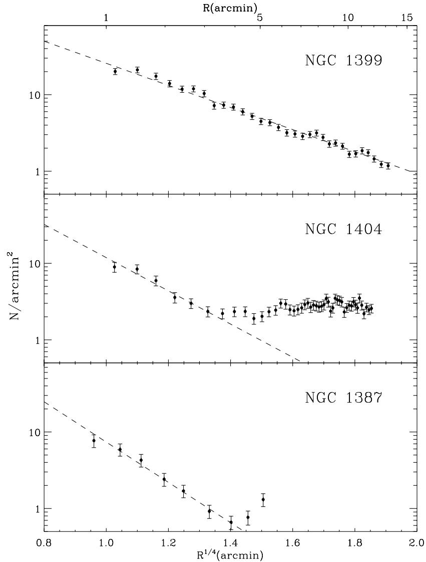
Figure 10. Number of GC candidates per unit area projected on the sky as a function of radial distance from the center of the galaxy. Radial bins are defined to contain approximately equal numbers of GCs ( \sim 100 GCs for NGC 1399; \sim 40 GCs for NGC 1404; \sim 25 GCs for NGC 1387). The numbers are corrected for the spatial completeness, but not for the contamination by foreground/background objects (see the text). Dashed line shows de Vaucouleurs' R^{1/4} fit of each profile.
