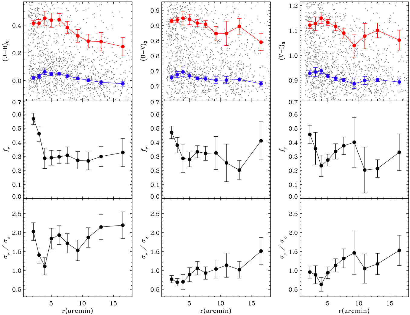
Figure 15. Parameters of bimodality in (U-B)_0 , (B-V)_0 , and (V-I)_0 colors (left, middle, and right columns) as a function of galactocentric distance for NGC 1399 GCs. The top, middle, and bottom panels show the mean colors ( \mu_b and \mu_r for blue and red GCs), the red GC fraction ( f_r ), and the ratios of color dispersions between blue and red GCs ( \sigma_r/\sigma_b ), respectively.
