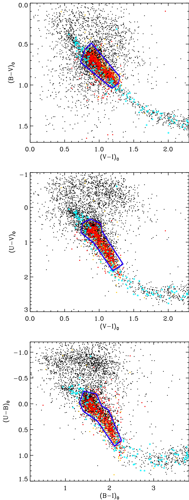
Figure 6. Color selection of GC candidates in NGC 1399. The selection criteria demarcated by blue lines were determined based on confirmed GCs with radial velocity measurements (red dots; Schubert et al. 2010) and/or with size measurements (orange dots; derived from HST ACS data). The cyan asterisks represent foreground stars confirmed with radial velocity measurements (Schubert et al. 2010). GC candidates are clearly separated from background sources in the (U - B)_0 color.
