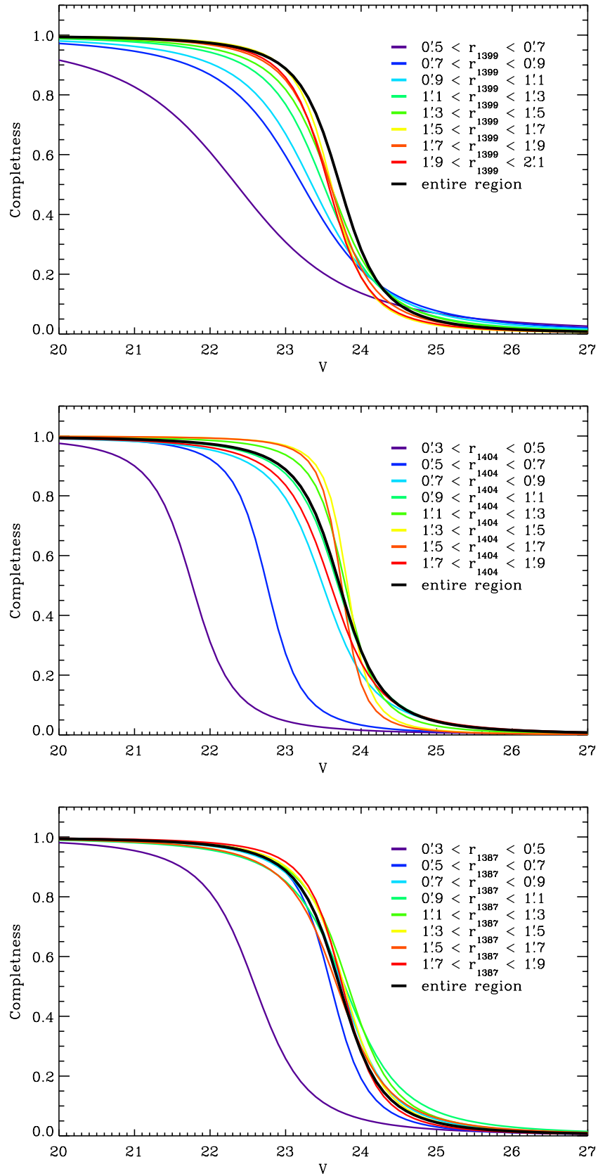
Figure 4. V-band completeness functions at various radial bins from the center of galaxies—NGC 1399 (top), NGC 1404 (middle), and NGC 1387 (bottom). The thick black line represents the overall completeness function. The completeness is very low near the center of the galaxies, and increases as one moves out from the center, and then flattens out beyond 1/3 for NGC 1399, 0/7 for NGC 1404, and 0/5 for NGC 1387.
