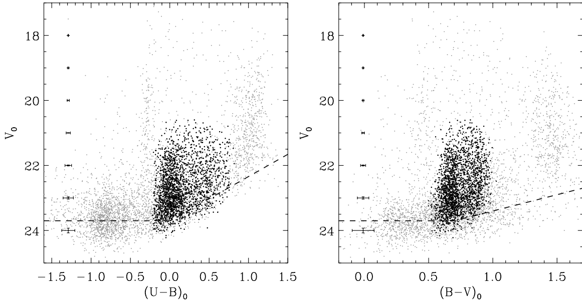
Figure 11. Color-magnitude diagrams of point sources. Black dots represent GC candidates, and gray dots represent foreground/background objects. Observational uncertainties as a function of V_0 are shown by error bars in the left corner of each diagram. Dashed lines indicate the limiting magnitude. The tilt of the limiting magnitude results from lower detection efficiency of red GCs than blue GCs in the U band. The GC candidates fainter than the limiting magnitude are taken out from the subsequent analysis.
