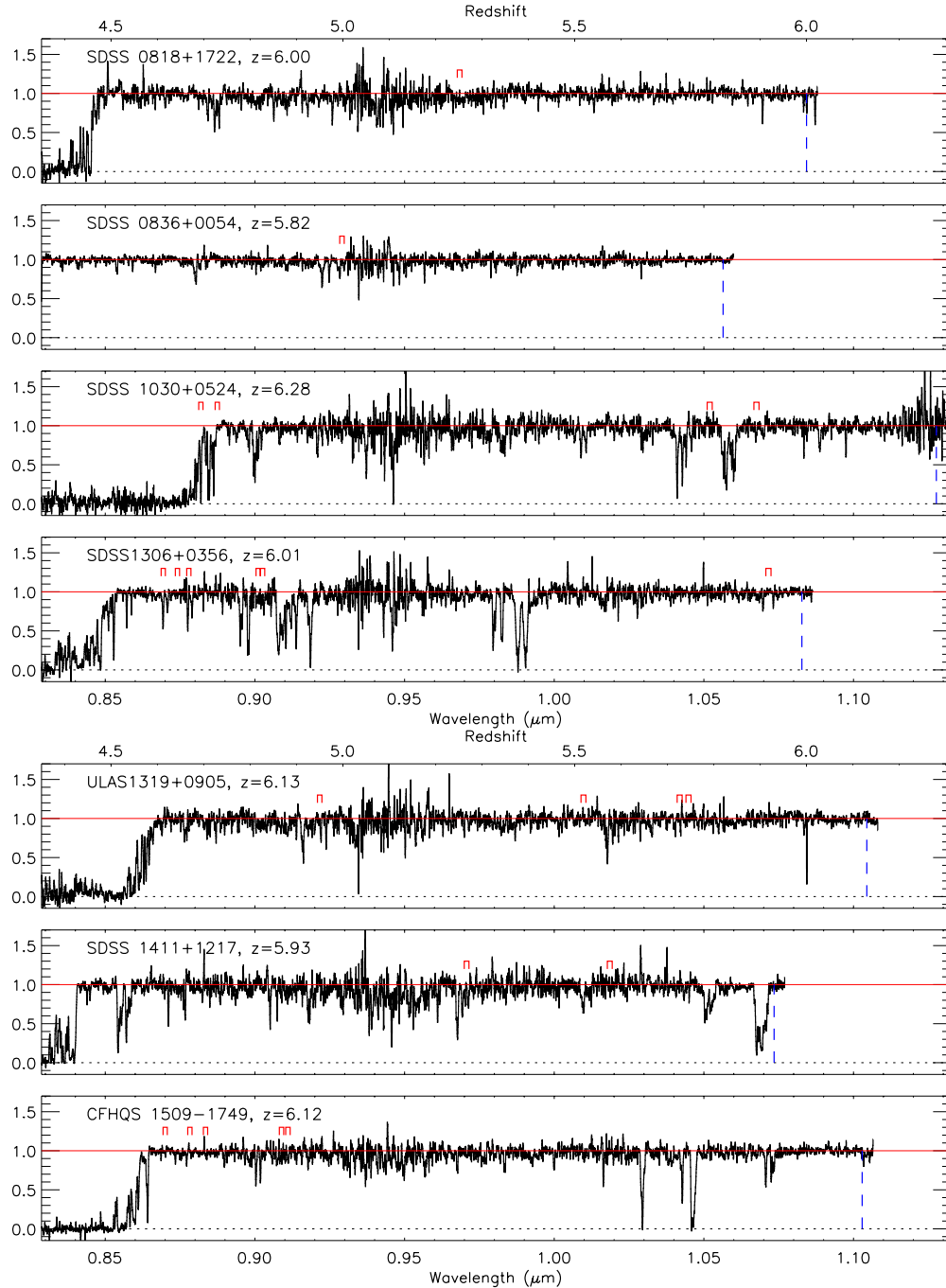
Figure 1. Normalized spectra of the seven sample objects, ranging from the minimum search redshift ( z = 4.35 in SDSS0836+0054) to the maximum z = 6.3 (in SDSS1030+0524). The locations of C IV doublet in Table 2 are shown with red marks, and the C IV wavelength at the QSO emission redshift is shown as a vertical dashed line. The weaker C IV systems that are difficult to see in this plot are better displayed in Figure 3.
