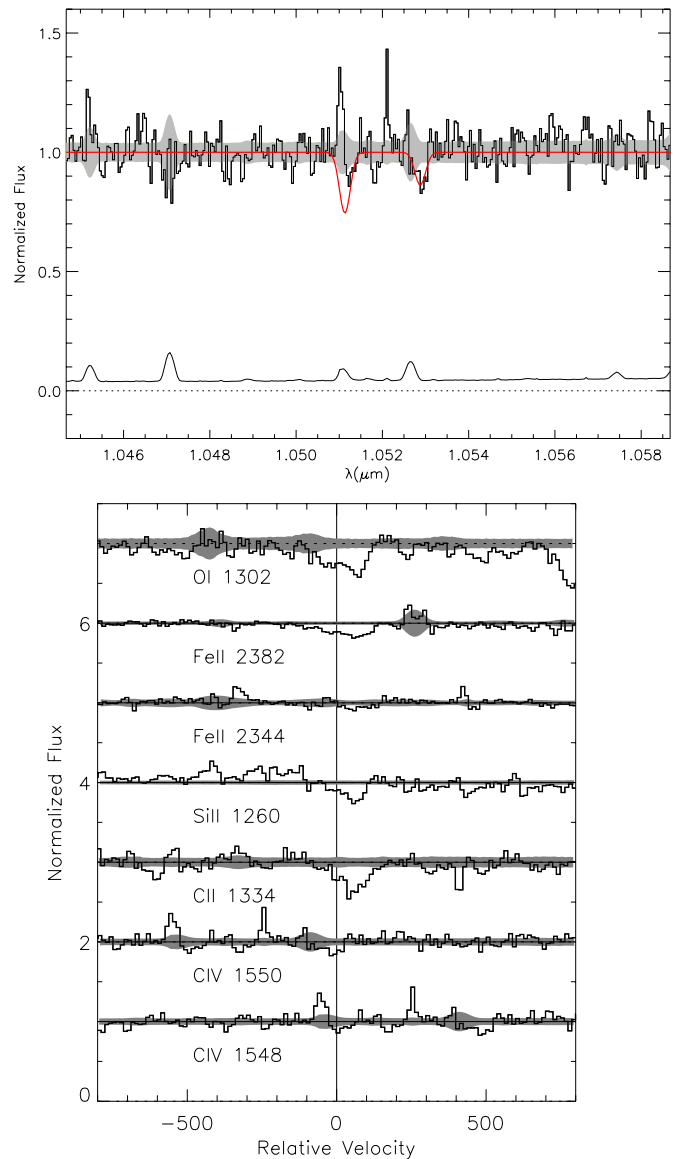
Figure 4. Top: FIRE spectrum showing the C IV region of SDSS0818+1722 at z = 5.78990 , where both Ryan-Weber et al. (2009) and D’Odorico et al. (2011) report tentative detection of a weak C IV system. Gray region shows the \pm 1\sigma error contours, while the solid black line shows a best-fit Voigt profile model to the 1550 Å component alone, which does not provide a good match to the 1548 Å line. There is evidence of systematic error in the sky subtraction on the blue wing of the profile (the positive spike). Bottom: confirmation of detected absorption in low-ionization species at this redshift, including O I, Fe II, Si II, and C II.
