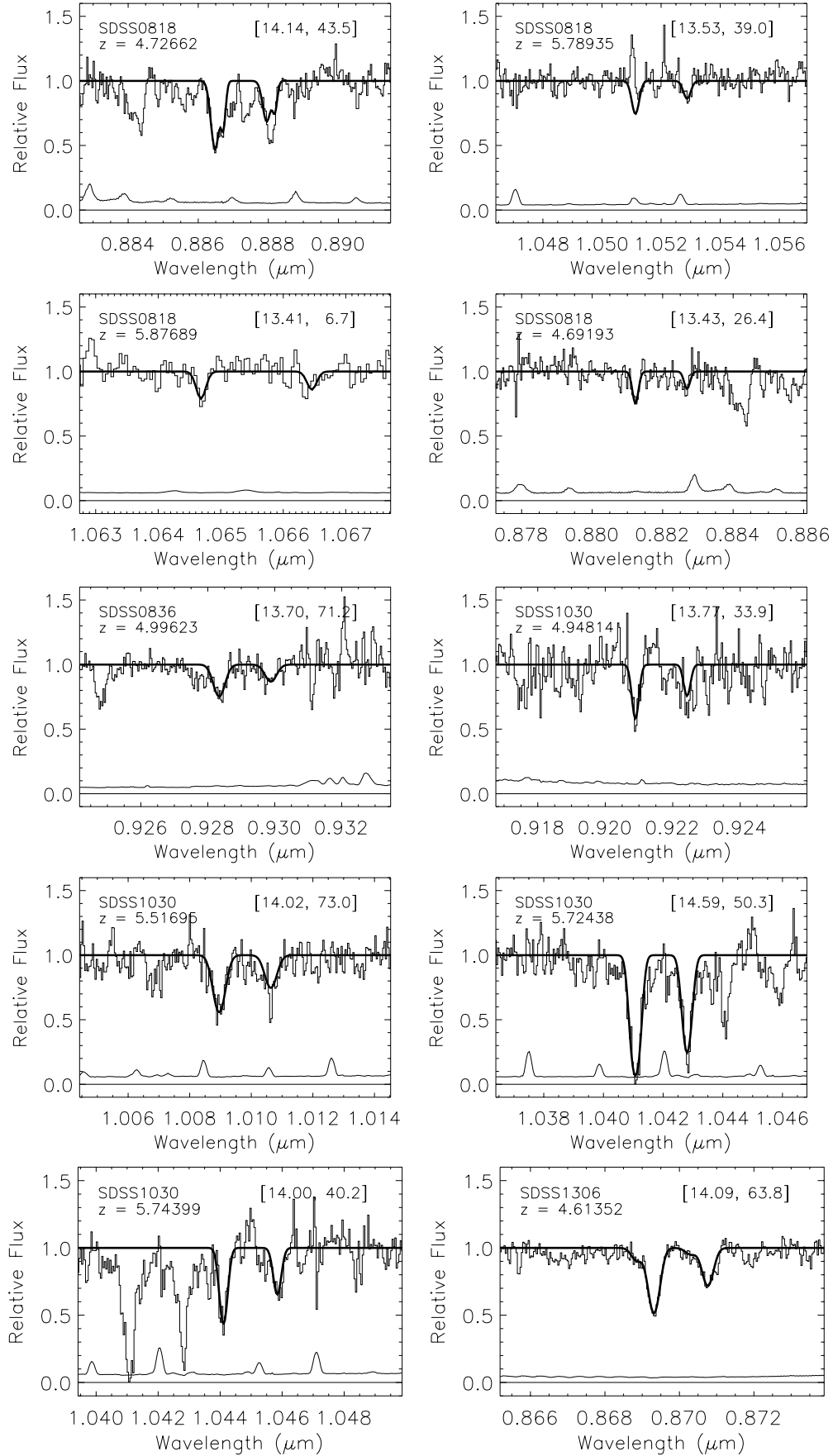
Figure 3. Plots of individual C IV systems listed in Table 2, in units of continuum normalized flux. The 1\sigma error array is shown at bottom and a best-fit Voigt profile is shown with a solid smooth line. The total \log(N_{\text{C IV}}) and b is shown for each system in square brackets.
