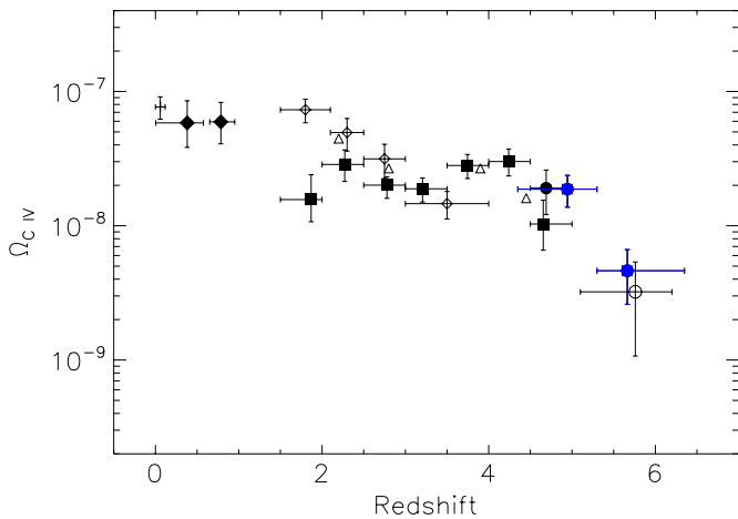
Figure 6. Evolution of the mass density in C IV, expressed as \Omega_{\text{C IV}} , for systems with 13.4 \leq \log(N_{\text{C IV}}) \leq 15.0 . Data from this study are shown in blue; the results of several prior studies are shown for comparison, where all are scaled to our fiducial cosmology and corrected for their varying degrees of completeness. Solid squares show results from Songaila (2001), open triangles are from Songaila (2005), open diamonds are from D’Odorico et al. (2010), solid diamonds are from Cooksey et al. (2010), the cross at z \approx 0 is from Danforth & Shull (2008), the solid black circle is from Pettini et al. (2003), and the open black circle is from Ryan-Weber et al. (2009). Ryan-Weber’s point has been adjusted to reflect re-identification of the putative z = 5.82 C IV system in SDSS1030 as Mg II.
