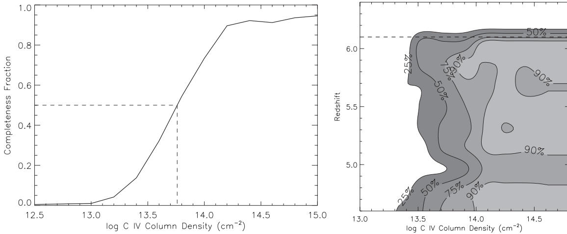
Figure 2. Left: the combined C IV sample completeness averaged over the full path of the survey. Dotted lines show the 50% completeness level, which occurs around N_{\text{C IV}} = 10^{13.75} \text{ cm}^{-2} . Right: the distribution of completeness with C IV column density and redshift. Some redshift ranges—particularly near z = 5.0 —have lower completeness because of higher noise levels in the data. This dependence is taken into account when correcting each detected line up for incompleteness when determining \Omega_{\text{C IV}} .
