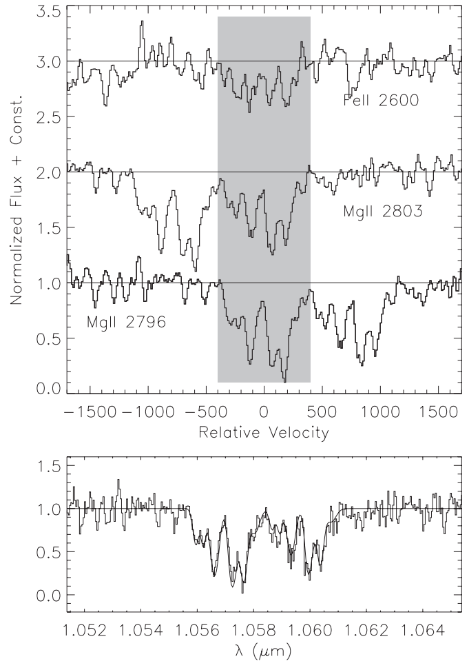
Figure 5. Stacked velocity plot showing matched profiles of the Mg II doublet along with Fe II at z = 2.780 . This identification supersedes prior work which flagged this system as C IV at z = 5.82 . Note the extremely broad velocity spread, which spans a total of \sim 800 \text{ km s}^{-1} . At bottom, we show a Voigt profile fit to the Mg II complex.
