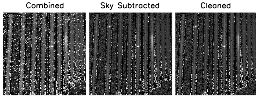
Figure 5. Example SH frames through the reduction process. Left is the post-pipeline combined frame, middle is the sky-subtracted frame, and right is the cleaned sky-subtracted frame, from which one-dimensional spectra are extracted.
