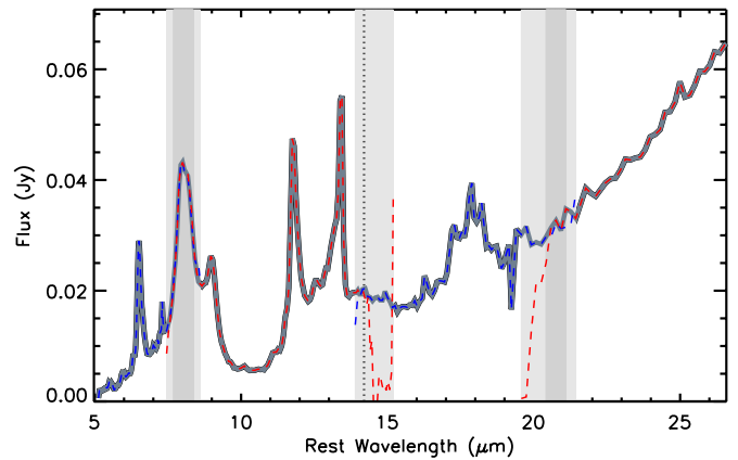
Figure 4. Example of method used to stitch the low-res spectra. The colored dashed spectra are from individual channels, from left to right: SL2 (blue), SL1 (red), LL2 (blue), and LL1 (red). The dark gray spectrum is stitched from these channels. Dark gray shaded areas represent the channel-overlap regions where two channels are medium-combined. The light gray shaded areas are the channel-overlap regions where the stitched spectrum is set to the values of the nearest channel. The default medium-combined region is the central 50% of the overlap region; however, this is adjusted manually to avoid end-of-channel transmission drops. The dotted line is the stitch point for the SL1–LL2 junction, which defaults to the middle of the overlap region but in many cases is set manually due to transmission drops.
