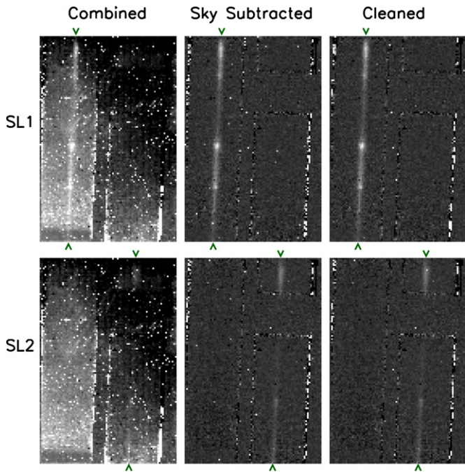
Figure 3. Example SL1 (upper) and SL2 (lower) frames through the reduction process. Left is the post-pipeline combined frame, middle is the sky-subtracted frame, and right is the cleaned sky-subtracted frame, from which one-dimensional spectra are extracted. Pointers mark the ends of the spectra—to the left of the frames for SL1 and to the lower right for SL2. The segments at the upper right are the bonus order spectra.
