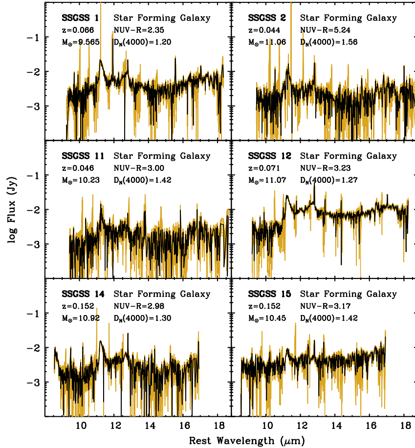
Figure 20. Short-high IRS spectra, reduced and stitched as described in Section 5.2. The yellow shaded region shows the \pm 1\sigma errors. Also given are the SSGSS catalog number, BPT type (Baldwin et al. 1981), redshift, stellar mass, NUV-R color, and D_N(4000) age diagnostic.
