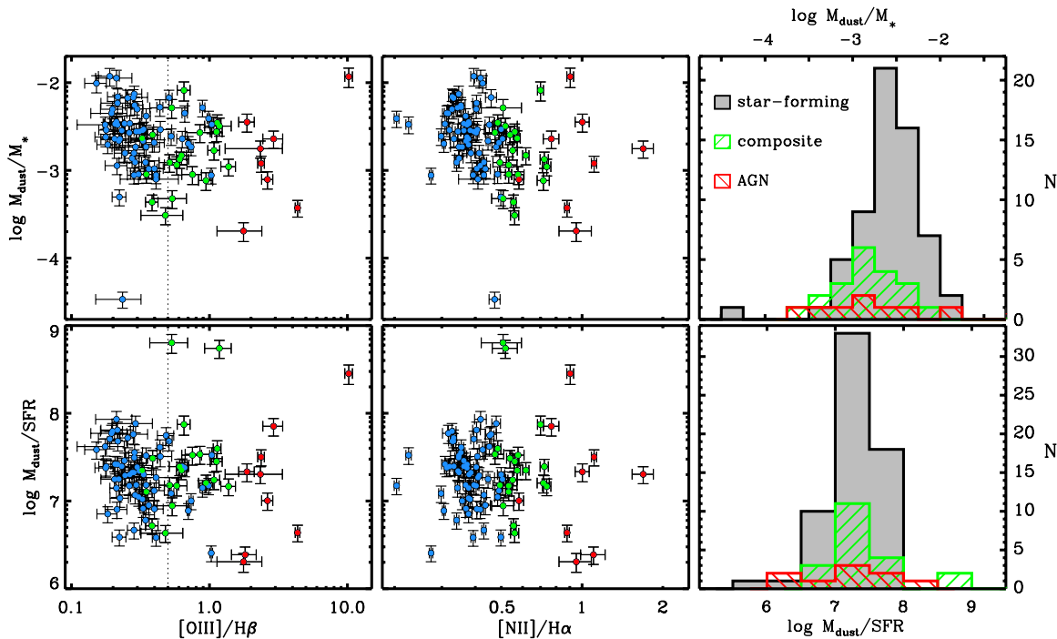
Figure 17. Upper panels: dust-to-stellar mass fraction vs. the optical emission line ratios [O III]/H\beta (left) and [N II]/H\alpha (middle). These line ratios define BPT AGN type, which is designated by the same color coding as Figure 13. Also shown is the distribution of dust fractions by AGN type (right). AGNs have significantly lower dust fractions than SF galaxies. SF galaxies with [O III]/H\beta > 0.5 (dotted line) are young galaxies with starburst-source hard radiation fields; these galaxies have significantly higher dust fractions than AGNs with similar [O III]/H\beta . Lower panels: same as above, except with the ratio of dust mass to SFR_e .
