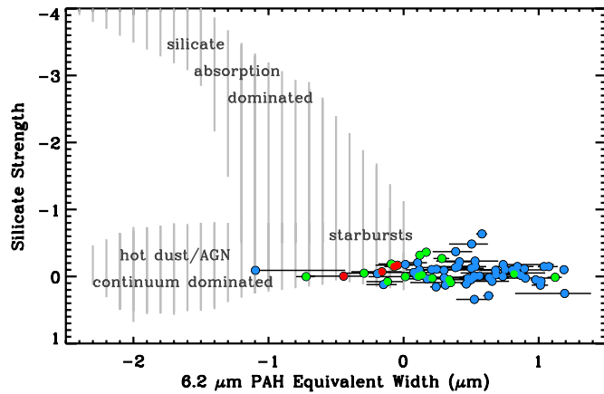
Figure 13. Equivalent width of the 6.2\ \mu\text{m} PAH feature vs. a silicate strength, defined as the log of the ratio of the minimum in the 9.7\ \mu\text{m} absorption trough to the interpolated value at this point from a linear fit to the 4.5\text{--}5\ \mu\text{m} and 14.5\text{--}15\ \mu\text{m} regions. SSGSS galaxies are color coded according to BPT designation (Kewley et al. 2001; Kauffmann et al. 2003a); blue points are star-forming galaxies, green points are composite sources, and red points are AGNs. The shaded region shows the positions on this plot of LIRGs, ULIRGs, starbursts, and AGNs from Spoon et al. (2007). These more extreme galaxies tend to have stronger silicate absorption and brighter continua than the more quiescent star-forming galaxies of the SSGSS sample.
