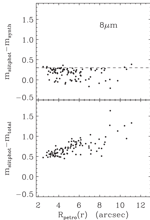
Figure 9. SL slit aperture magnitude minus synthesized and circular aperture magnitudes as a function of r -band Petrosian radius.
