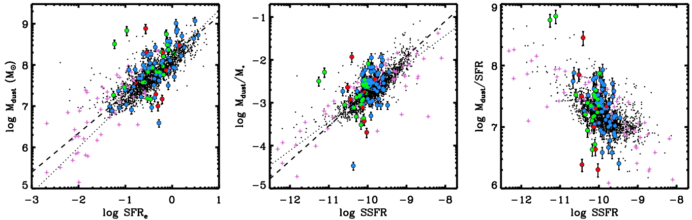
Figure 16. Left: dust masses for SSGSS galaxies from models of Draine & Li (2007) vs. SFR_e (Brinchmann et al. 2004; colored circles, coded by BPT designation; see Figure 13). Also plotted are the results of the dust model of da Cunha et al. (2010) for SDSS galaxies (black points) and SINGS galaxies (pink crosses). The best log-log regression lines are shown for SSGSS (dashed) and SDSS (dotted). Middle: dust-to-stellar mass fraction vs. SSFR; right: dust mass-to-SFR ratio.
