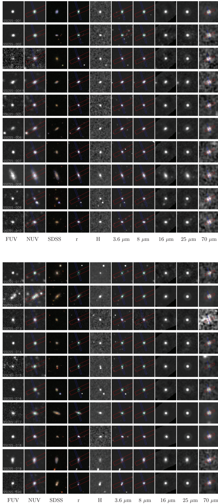
Figure 18. Multi-wavelength images of the 101 galaxies of the SSGSS sample. Each horizontal strip shows a given galaxy in, respectively: GALEX FUV and NUV, SDSS multi-color, r , H , IRAC 3.6 \mu\text{m} and 8 \mu\text{m} , 16 \mu\text{m} from SSGSS peak-up images, and MIPS 25 \mu\text{m} and 70 \mu\text{m} . All boxes are 60'' on a side except for the 70 \mu\text{m} band, which is 120''.
