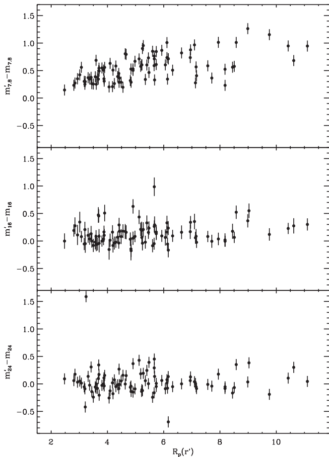
Figure 8. Synthetic minus SWIRE photometry as a function of r -band Petrosian radius 8\ \mu\text{m} , 16\ \mu\text{m} , and 24\ \mu\text{m} . The trend between this magnitude difference and radius observed in the 8\ \mu\text{m} band suggests slit losses in the SL module, but not at longer wavelengths.
