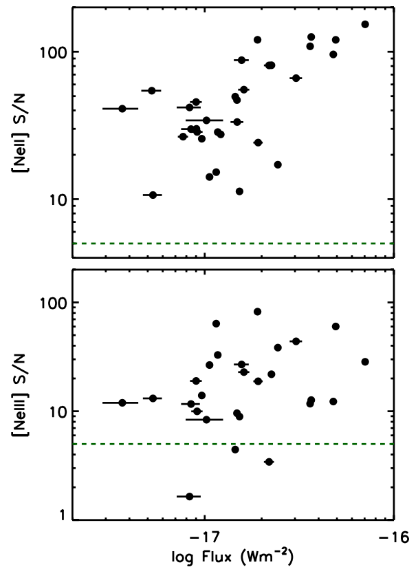
Figure 7. Signal-to-noise ratios of the [Ne II] (upper) and [Ne III] (lower) emission lines from the hi-res spectra vs. the PAHFIT-measured fluxes. Dashed lines indicate target S/N.
