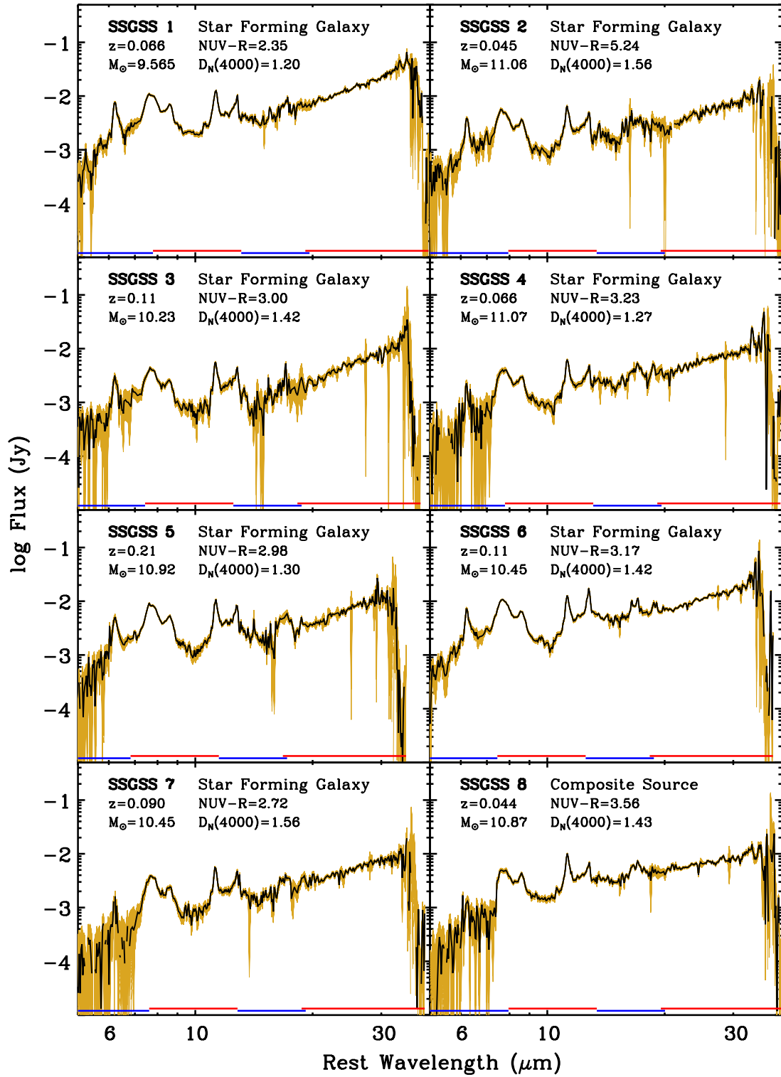
Figure 19. Short-low and long-low IRS spectra, reduced and stitched as described in Section 5.1. The yellow shaded region shows the \pm 1\sigma errors. The wavelength range of each IRS module is shown at the base of each panel, from left to right: SL2 (blue), SL1 (red), LL2 (blue), and LL1 (red). Also given are the SSGSS catalog number, BPT type (Baldwin et al. 1981), redshift, stellar mass, NUV-R color, and D_N(4000) age diagnostic.
