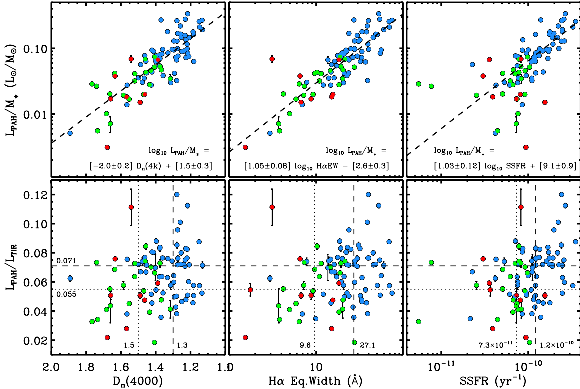
Figure 15. Upper: L_{\text{PAH}}/M_* vs. D_n(4000) (left), \text{H}\alpha EW (middle), and SSFR (right). Galaxies are color coded according to BPT type as in Figure 13. AGNs and composite sources sit on the same loci as SF galaxies, and have systematically older stellar populations. Dashed lines show regression fits for the SF population (blue points), with AGNs/composites excluded. Lower: as above, but for L_{\text{PAH}}/L_{\text{TIR}} . Dashed and dotted lines show the median values for SF galaxies and AGNs/composites, respectively.
