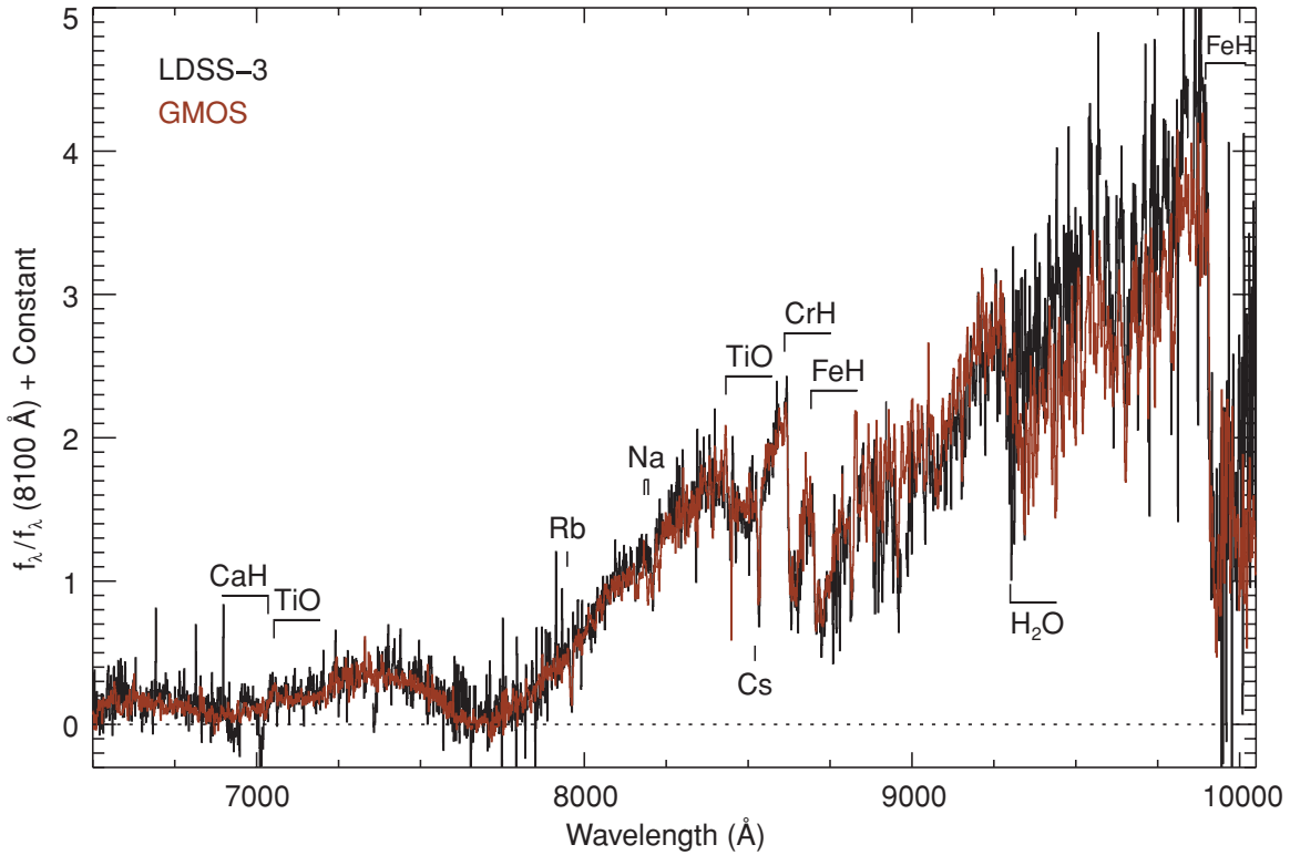
Figure 3. Red optical spectra of 2MASS J0616–6407 obtained with LDSS-3/Magellan (black) and GMOS/Gemini (red). The spectra are normalized to unity at 8100 Å. Prominent atomic and molecular absorption features are indicated.
