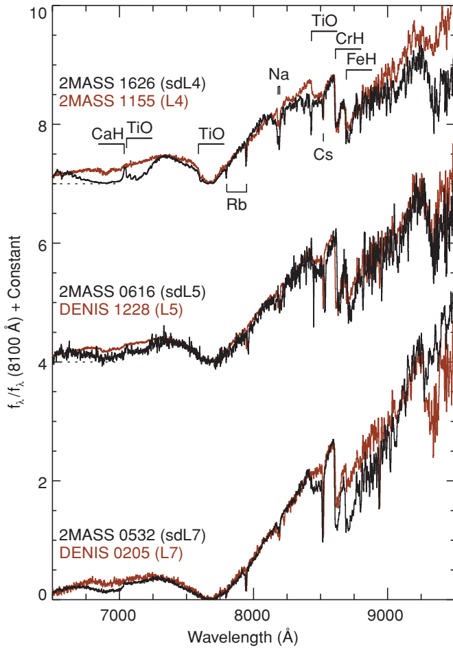
Figure 4. Red optical spectra of 2MASS J1626+3925 (sdL4; Burgasser et al. 2007), 2MASS J0616–6407, and 2MASS J0532+8246 (sdL7; Burgasser et al. 2003) compared to those of 2MASS 1155009+230706 (L4; Kirkpatrick et al. 1999), DENIS-P J1228.2–1547 (L5; Kirkpatrick et al. 1999), and DENIS-P J0205.4–1159 (L7; Kirkpatrick et al. 1999), respectively. The spectra are normalized to unity and offset by constants (dotted lines). Prominent atomic and molecular absorption features are indicated.
