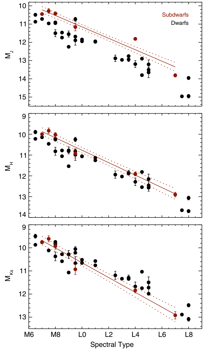
Figure 5. 2MASS M_J , M_H , and M_{K_s} values for LHS 377 (sdM7), LSR 2036+5059 (sdM7.5), LSR J1425+7102 (sdM8), SSSPM 1013–1356 (sdM9.5), 2MASS J1626+3925 (sdL4), and 2MASS J0532+8246 (sdL7) are shown in red. The linear fit to these values and the \pm 1 \sigma range are shown as solid and dotted lines. Shown in black are a sample of field dwarfs from Dahn et al. (2002) and references therein that have not been identified as binaries in high-resolution imaging. All spectral types are based on optical spectroscopy.
