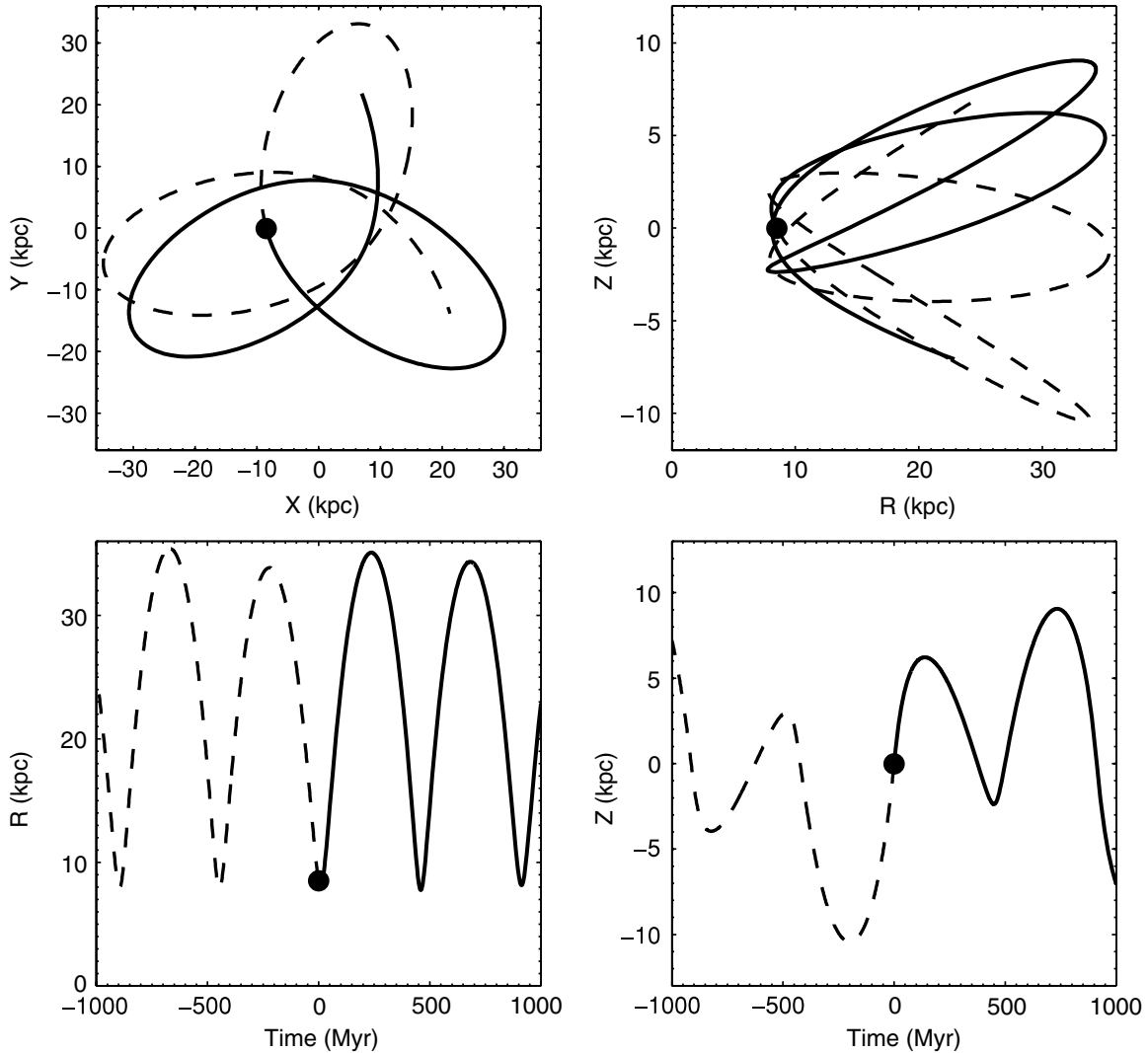
Figure 6. Galactic orbit of 2MASS J0616–6407 over \pm 1 Gyr, based on the halo-dominant mass model of Binney & Tremaine (Model I; 2008). The upper panels show the orbit in (x, y) and (r, z) coordinates. The x -axis is along the line connecting the Galactic center and the Sun while the z -axis denotes height above the Galactic plane. The lower panels show the time evolution of r and z , with past motion denoted by dashed lines and future motion denoted by solid lines. The position of the Sun is denoted with a solid circle.
