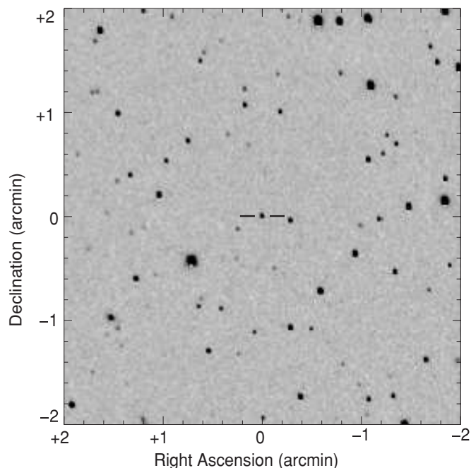
Figure 1. J -band image of the field centered around 2MASS J0616–6407 obtained with the CPAPIR on the 1.5 m CTIO on 2008 January 17 (UT). The field is 4' on a side and north is up and east is to the left.
