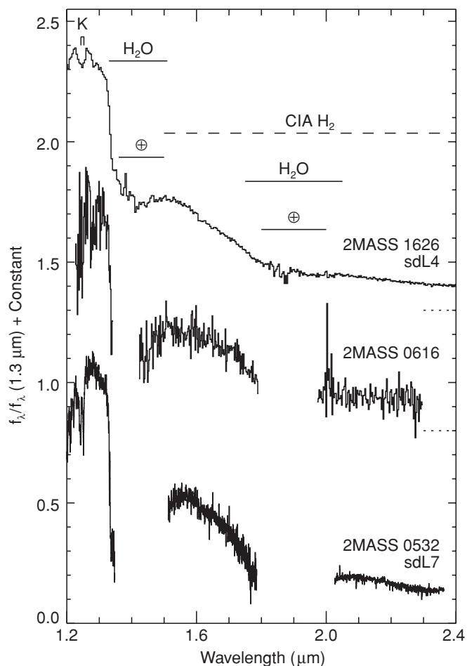
Figure 2. Near-infrared spectra of 2MASS J1626+3925 (sdL4; Burgasser et al. 2007), 2MASS J0616–6407, and 2MASS J0532+8246 (sdL7; Burgasser et al. 2003). The spectra are normalized to unity at 1.3 \mu\text{m} and offset by constants (dotted lines). Prominent atomic and molecular absorption features are indicated. The S/N of the 2MASS J0616–6407 spectrum is not high enough to detect the 1.25 \mu\text{m} K I doublet.
