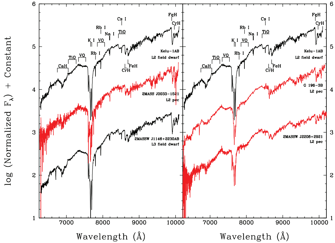
FIG. 11.— Left : Peculiar L2 dwarf 2MASS J0033–1521 compared to the standard L2 dwarf Kelu-1 and the standard L3 dwarf 2MASS J1146+2230. Right : Peculiar L2 dwarfs G 196-3B and 2MASS J2208+2921 compared to the same L2 standard shown in the left panel. In both panels the spectra have been normalized to unity at 8250 Å and a constant offset added to separate the spectra vertically.
