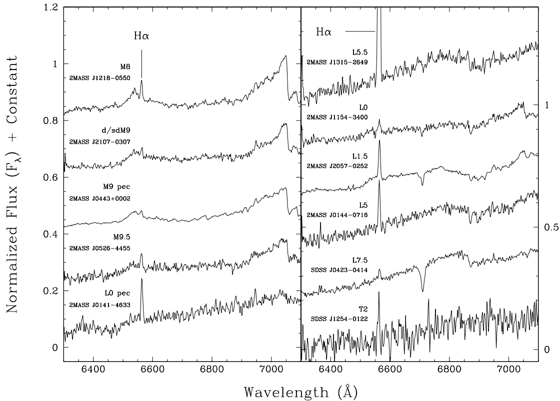
FIG. 6.—Zooms of the Keck/LRIS spectra in the 6300–7100 Å region for those objects in Table 3 exhibiting H \alpha emission. Note that three of the objects (2MASS J1154–3400, 2MASS J2057–0252, and SDSS J0423–0414) exhibit both Li I absorption at 6708 Å and H \alpha emission.
