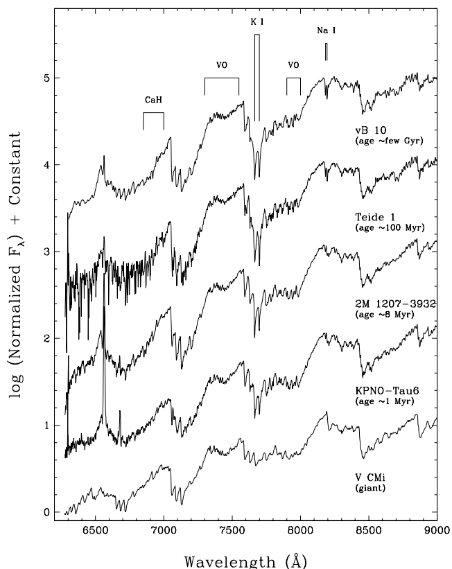
FIG. 7.—Optical spectral sequence showing feature changes as a function of age (gravity) at M8–M8.5. Each object is labeled with its age as deduced from membership in a cluster (either the Pleiades at \sim 100 Myr, the TW Hydrae association at \sim 8 Myr, or the Taurus Molecular Cloud at \sim 1 Myr) or from association with a higher mass primary (in the case of vB 10). Note the weakening of alkali lines (K I and Na I) and the CaH band as well as the strengthening of the VO bands from oldest (vB 10) to youngest (KPNO–Tau6). Although the change in spectral morphology is subtle from object to object, the plot demonstrates that gravity differences can be discerned at the \sim 1 dex level in \log (age). The spectrum of a late-M giant with \log g \approx 0 is shown at the bottom to illustrate the behavior of these features at even lower gravities. All spectra have been corrected for telluric absorption.
