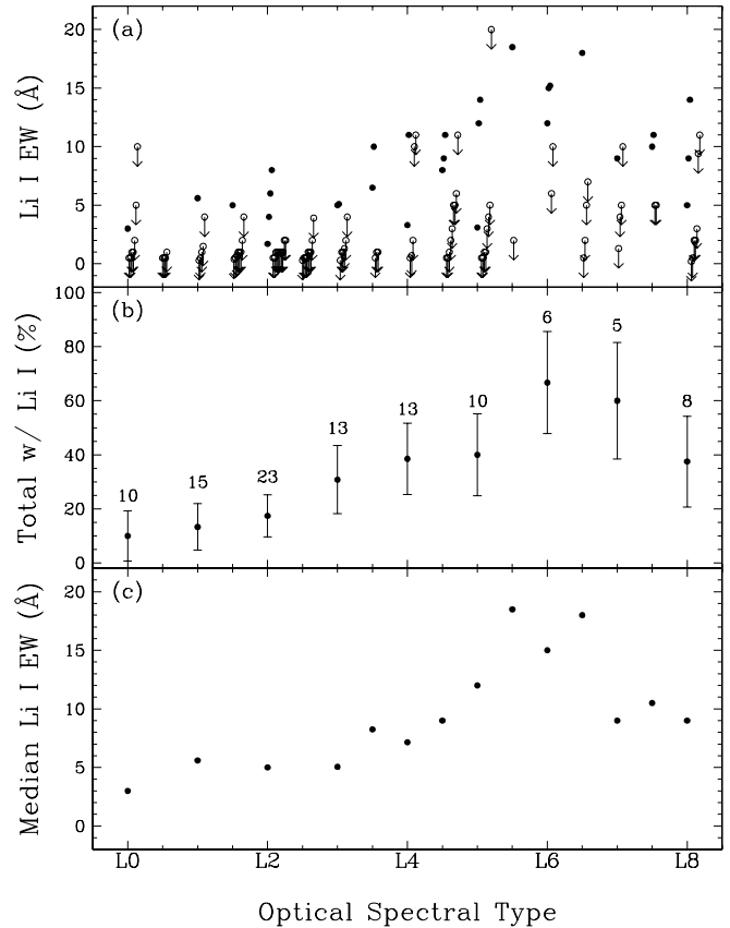
FIG. 17.—Update of Fig. 7 from Kirkpatrick et al. (2000). (a) Li I equivalent widths as a function of spectral subclass for all L dwarfs for which we have ever obtained Keck-LRIS spectra. Filled circles denote objects having a detected Li I absorption line. Open circles with downward arrows denote upper limits to the Li I EW for those objects for which no line was detected. To avoid the overlapping of data caused by the quantization of spectral types, some of the points have been given slight offsets along the x-axis. (b) Percentage of L dwarfs showing Li I absorption as a function of spectral subclass. The only objects used in this computation are those for which a Li I equivalent width of 3 Å or more would be detectable. Points have been binned into integer subtypes in which L0 and L0.5 dwarfs have been combined in the L0 bin, L1 and L1.5 dwarfs have been combined in the L1 bin, etc. The total number of objects in each bin is given above each data point. (c) Median Li strength as a function of spectral class for those objects for which lithium absorption was detected.
