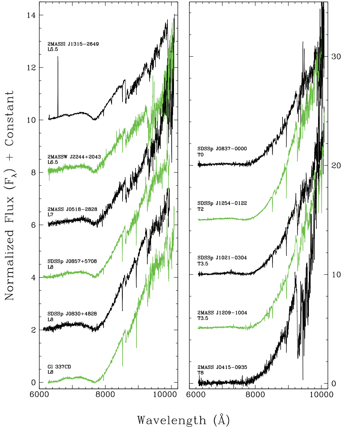
FIG. 4.—Keck/LRIS spectra of the 11 objects in Tables 4 and 5. All spectra have been normalized to unity at 8250 \text{\AA} . Integral offsets have been added along the y-axis to separate the spectra vertically—offsets are 2, 4, 6, 8, and 10 for the left panel, and 5, 10, 15, and 20 for the right panel. All of these spectra have been corrected for telluric absorption except for 2MASS J2244+2043 and 2MASS J0518-2828.
