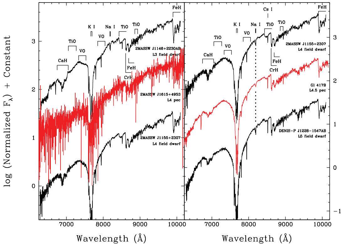
FIG. 12.— Left : Peculiar L4 dwarf 2MASS J1615+4953 compared to the standard L3 dwarf 2MASS J1146+2230 and the standard L4 dwarf 2MASS J1155+2307. Right : Peculiar L4.5 dwarf G1 417B compared to the same L4 standard shown in the left panel and the L5 standard DENIS-P J1228–1547. In both panels the spectra have been normalized to unity at 8250 Å and a constant offset added to separate the spectra vertically.
