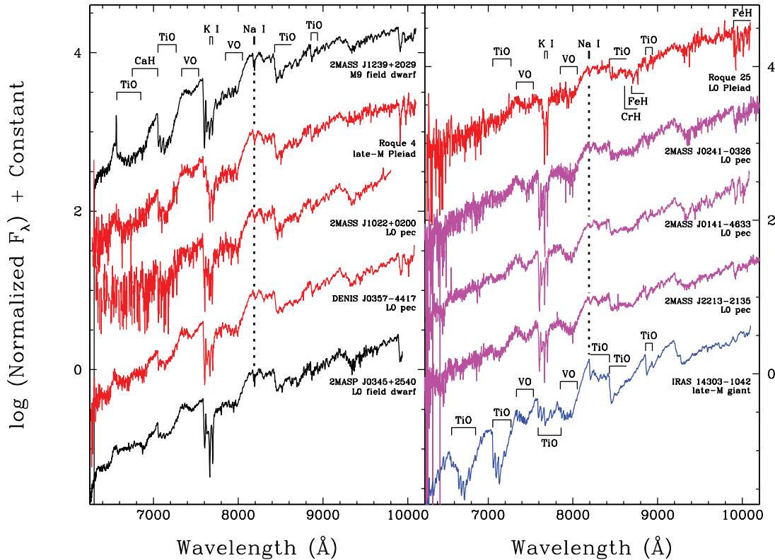
FIG. 9.— Left : Slightly peculiar L0 dwarfs 2MASS J1022+0200 and SDSS J0357-4417 compared to a normal field M9 (2MASS J1239+2029), an M9 dwarf in the Pleiades (Roque 4), and the standard L0 dwarf 2MASS J0345+2540 from Kirkpatrick et al. (1999b). Prominent features are marked. Right : More peculiar L0 dwarfs 2MASS J0241-0326, 2MASS J0141-4633, and 2MASS J2213-2135 compared to an L0 member of the Pleiades (Roque 25) and a late-M giant (IRAS 14303-1042). In both panels spectra have been normalized to unity at 8250 Å and offset along the y-axis to separate them vertically.
