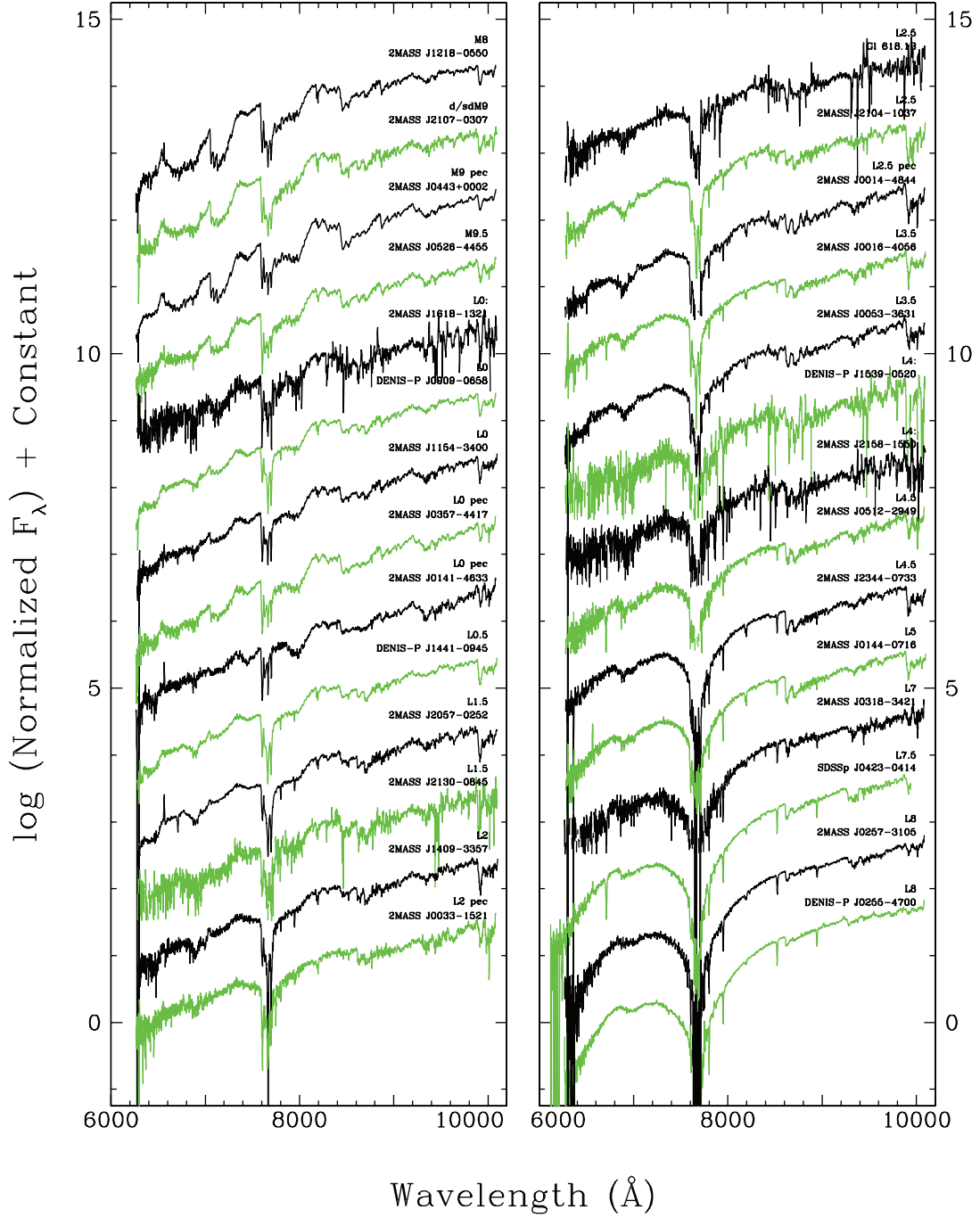
Fig. 3.—Same data shown in Fig. 2, except that the y-axis is scaled logarithmically to emphasize features at shorter wavelengths.
