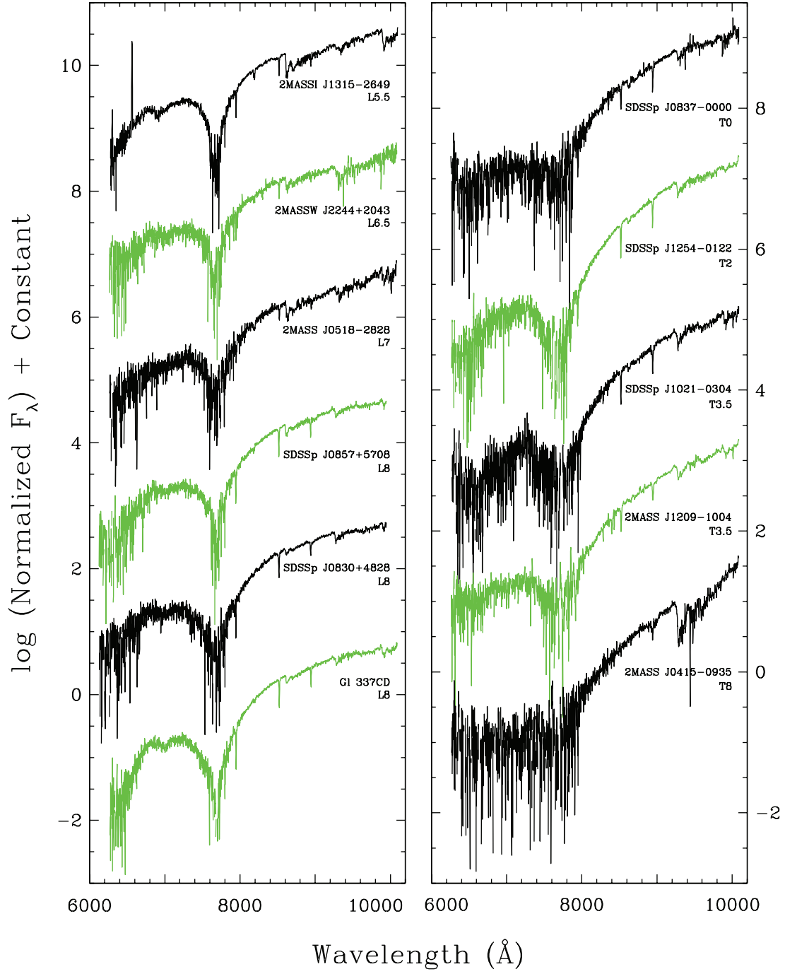
FIG. 5.—Same as Fig. 4, except that the objects are plotted on a logarithmic, rather than a linear, scale to emphasize features at the shortest wavelengths and to avoid overlap at the red end of the spectra. Vertical offsets are integral multiples of two in both panels.
