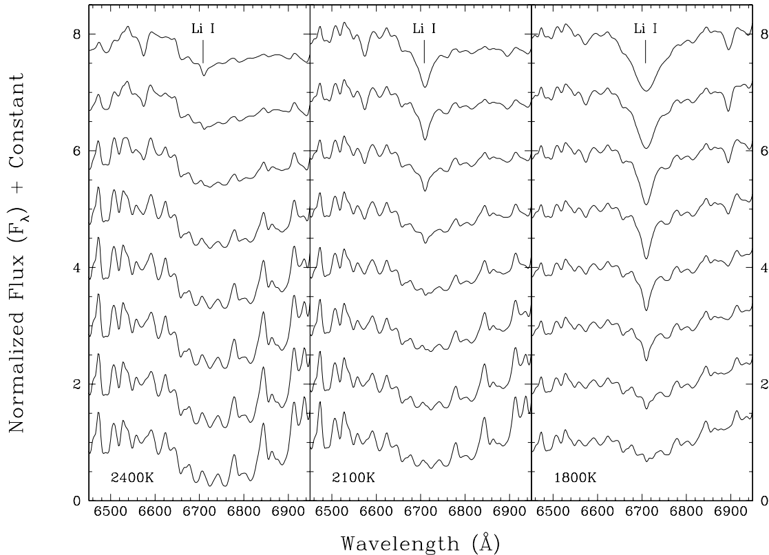
FIG. 22.—Synthetic spectral models at effective temperatures of 2400 K (left), 2100 K (middle), and 1800 K (right) for objects of solar abundance. Each panel illustrates the behavior of the spectra over a range of gravities, decreasing in half-dex increments from \log g = 6.0 at the top of each panel to \log g = 2.5 at the bottom. Note the universal weakening of the Li I line as gravity is lowered. The spectra displayed here have a resolution of 10 Å, identical to that of our empirical spectra.
