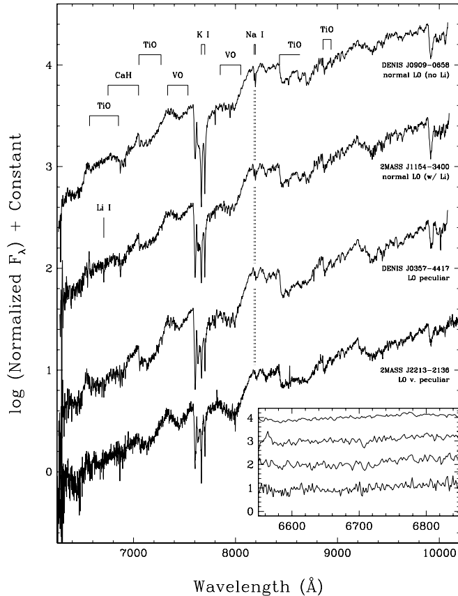
FIG. 18.—Sample spectra of optical L0 dwarfs from each of the four age bins of Table 8. These are displayed on a logarithmic scale, normalized to one at 8250 Å, with integers offsets added in the y -direction to separate spectra vertically. The spectrum with the best signal-to-noise ratio in each bin is shown. The inset shows a zoom-in around the 6708 Å Li I line for each of the four. In the inset, spectra are shown on a linear scale, normalized to one near 6750 Å, and again offset by integers.
