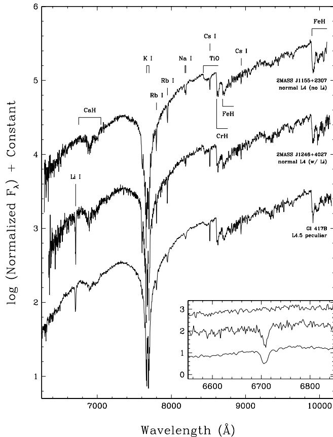
FIG. 20.—Sample spectra of optical L4 dwarfs from each of the three populated age bins of Table 8. The inset shows a zoom-in around the Li I line for each of the three. Normalizations and scalings are the same as in Fig. 18.
