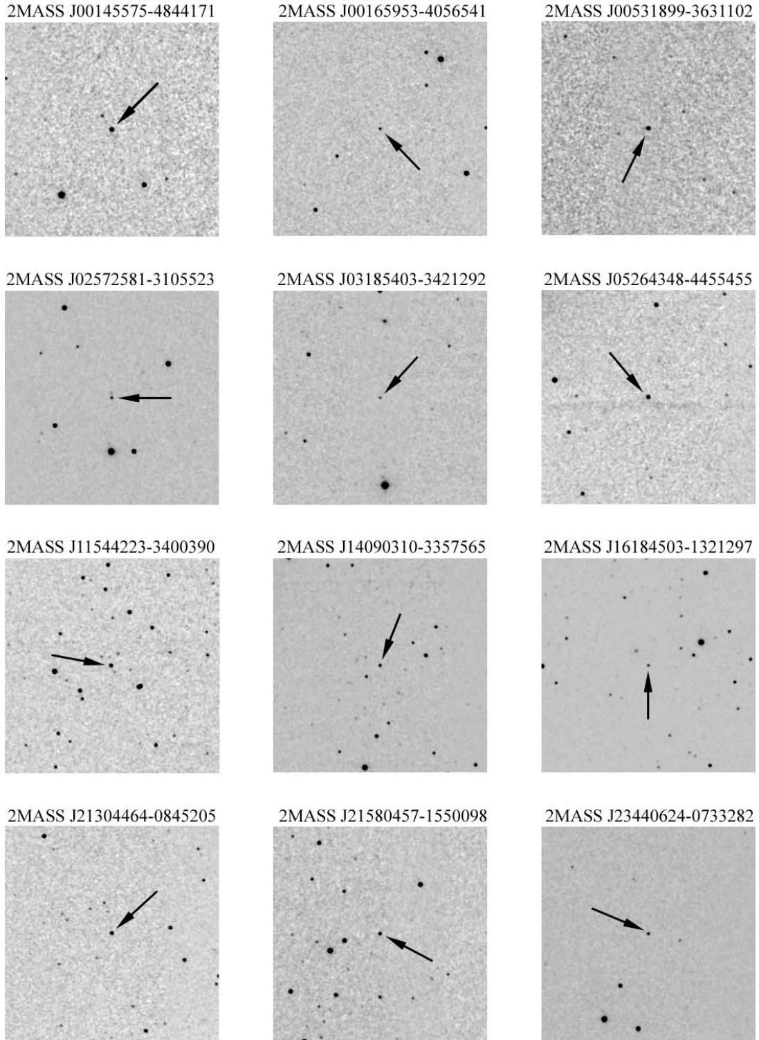
FIG. 1.—2MASS J -band finder charts for the new objects identified in Table 1. All images are 5' square with north up and east to the left. The positions of the new L and late-M dwarfs are marked with arrows. Note that the fainter object a few arcseconds north of 2MASS J02572581–3105523 is merely an artifact—a latent image persisting from the previous 2MASS frame and caused by the brighter star due south.
