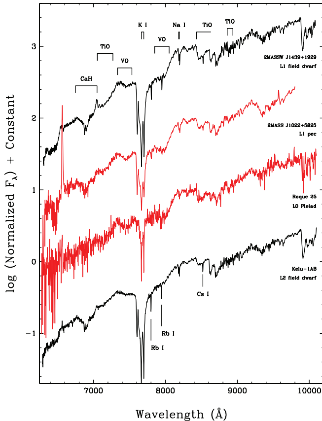
FIG. 10.—Peculiar L1 dwarf 2MASS J1022+5828 compared to the standard L1 dwarf 2MASSW J1439+1929 and an L0 dwarf (Roque 25) in the Pleiades. Prominent features are marked. Spectra have been normalized to unity at 8250 Å and have been offset along the y -axis to separate the spectra vertically.
