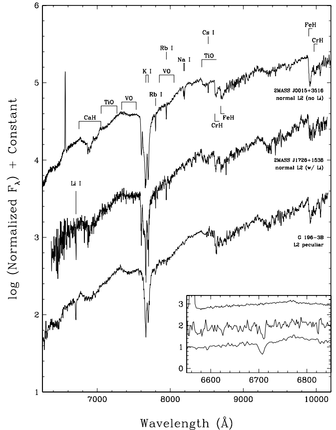
FIG. 19.—Sample spectra of optical L2 dwarfs from each of the three populated age bins of Table 8. The inset shows a zoom-in around the Li I line for each of the three. Normalizations and scalings are the same as in Fig. 18.
