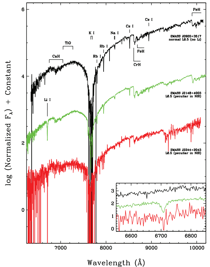
FIG. 21.—Sample spectra of optical L6.5 dwarfs from each of the three populated age bins of Table 8. The inset shows a zoom-in around the Li I line for each of the three. Normalizations and scalings are the same as in Fig. 18.
