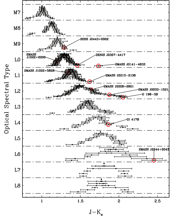
FIG. 14.— J - K_s colors for a collection of M7–L8 dwarfs with optically determined spectral types. Each bin represents a full integral subtype: “M7” includes M7 and M7.5 dwarfs, “M8” includes M8 and M8.5 dwarfs, etc. For each group of objects, the median color in the group is plotted highest in the bin; colors falling farther from the median are plotted progressively farther down the y-axis. Sample selections are described in the text. We use red circles to mark eleven objects we spectroscopically identify as low gravity. We also mark with a red triangle the color location of a peculiar L dwarf, 2MASS J2208+2921, from Kirkpatrick et al. (2000) that did not meet the selection criteria for the plot.
