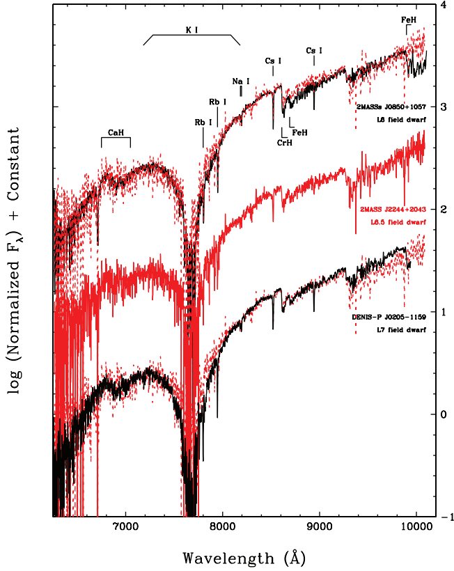
FIG. 13.—2MASS J2244+2043 (red) compared to the L6 and L7 optical standards (black) 2MASS J0850+1057 and DENIS J0205-1159. Even though the near-infrared spectrum of this object is extremely peculiar with respect to normal late-L dwarfs, the optical spectrum differs only subtly from a normal L6.5 dwarf. In both panels the spectra have been normalized to unity at 8250 Å and a constant offset added to separate the spectra vertically. Flux is plotted in logarithmic units so that features across all wavelengths can be more easily distinguished.
