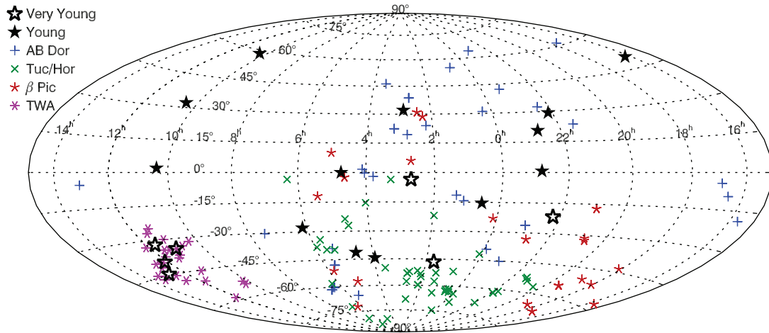
FIG. 15.—Hammer (equal-area) projection of the sky in J2000.0 equatorial coordinates showing members of the AB Doradus moving group ( blue plus signs ), the Tucana-Horologium association ( green crosses ), \beta Pictoris moving group ( red asterisks ), and the TW Hydrae association ( magenta snowflakes ) as listed in Zuckerman & Song (2004). Locations of the 20 low-gravity field dwarfs of Table 6 are shown by filled stars for objects with age estimates \sim 100 Myr and by open stars for objects with age estimates \sim 10 Myr.
