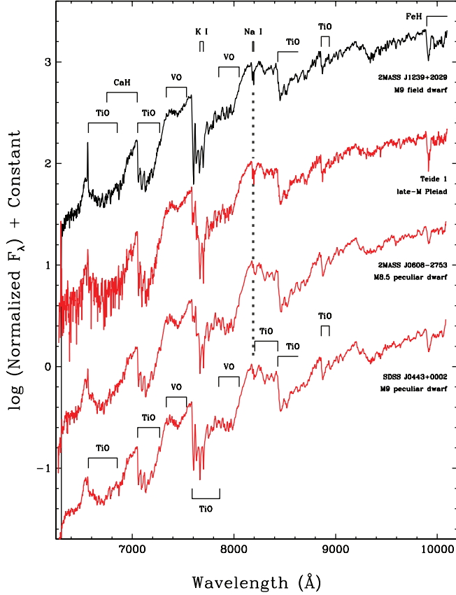
FIG. 8.—Peculiar M8.5 dwarf 2MASS J0608–2753 and the peculiar M9 dwarf SDSS J0443+0002 compared to an M9 field dwarf (2MASS J1239+2029) and a late-M member of the Pleiades (Teide 1). Prominent spectral features are marked. Spectra have been normalized to unity at 8250 Å and offset along the y-axis to separate them vertically.
