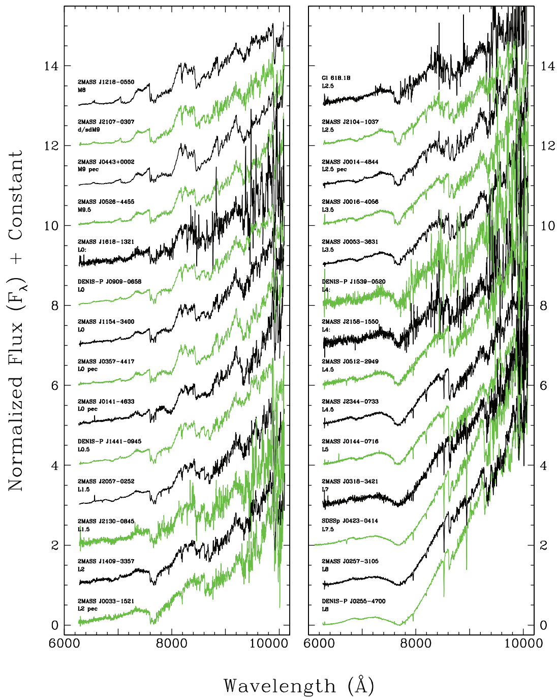
FIG. 2.—Keck/LRIS spectra of the 28 objects listed in Table 3. Each spectrum is normalized to one at 8250 \text{\AA} and an integral offset is added to this normalized flux so that the spectra are clearly separated along the y -axis. Spectra are ordered from earliest to latest with M8 through L2 shown in the left panel and L2.5 through L8 shown in the right panel. The spectra shown here are not corrected for telluric absorption. Colors of the spectra in Figs. 2–5 alternate between black and green to aid in presentation.
